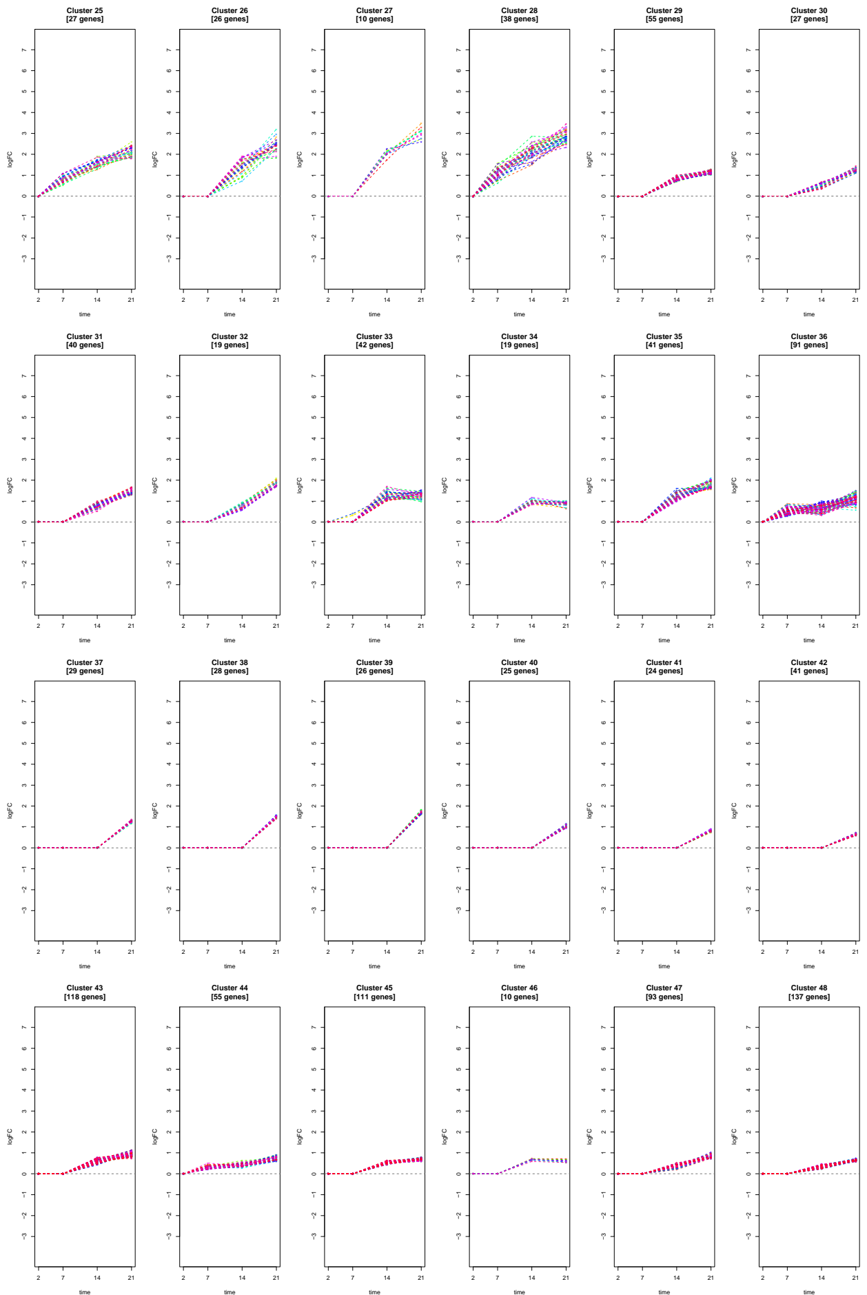
Additional file 5: Fig. S5. Expression profiles of the tomato gene clusters during TYLCV infection. DEGs were clustered into 48 groups based on their expression changes during infection. For each cluster the log 2 FC of the DEGs (y axis) are represented during TYLCV infection (x axis, 2, 7, 14 and 21 dpi).
