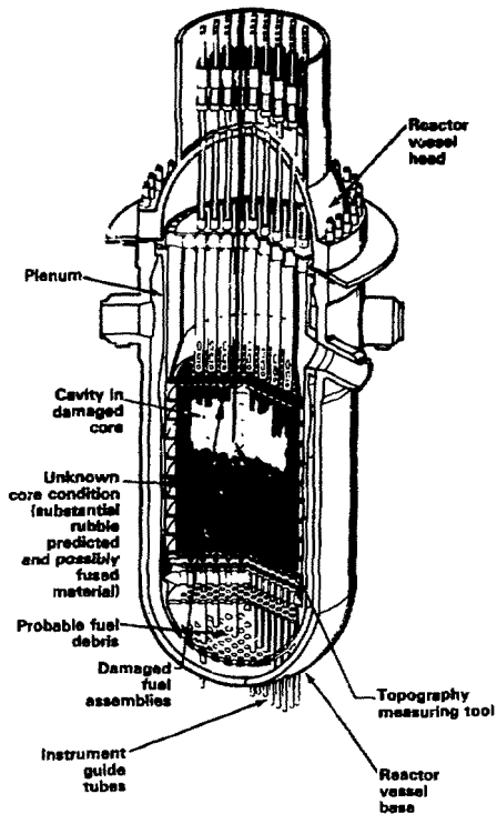
REACTOR VESSEL SHOWING DAMAGED FUEL AND CAVITY
