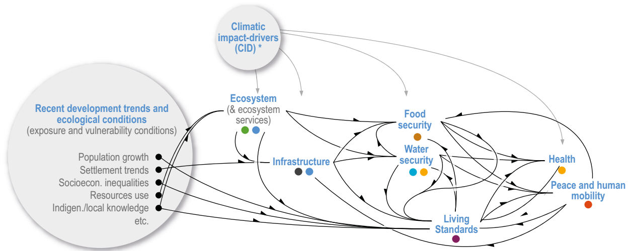
(b) Illustration of interactions at the Key Risk level (e.g. from ecological risk to key dimensions for human societies)
