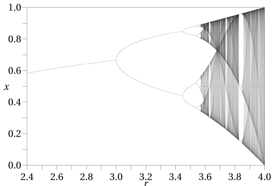
Figure 2.- Bifurcation diagram for the logistic map as a function of r .
