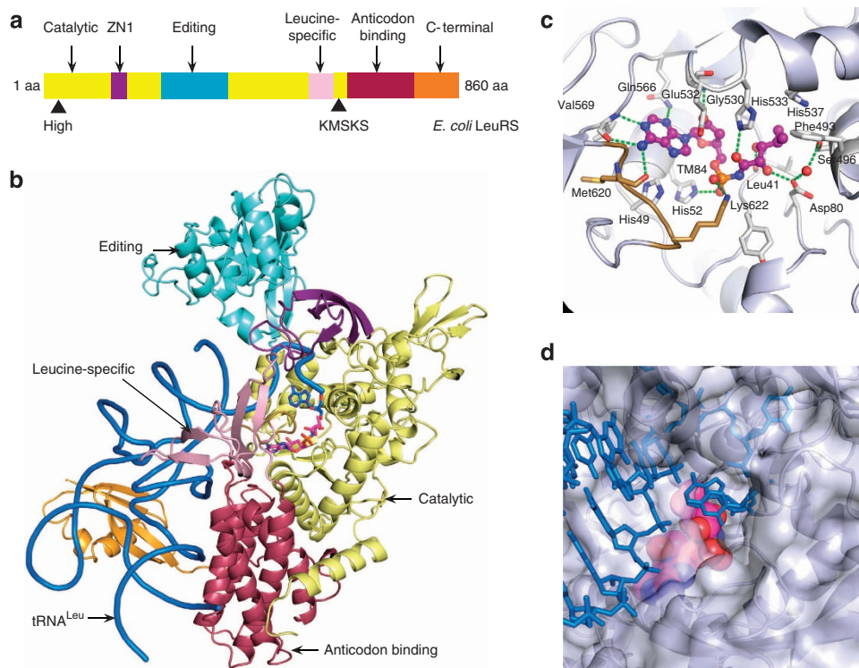
Figure 4 | Structure of the LeuRS Ec · tRNA Leu · TM84 inhibition complex. (a) Domain structure of LeuRS Ec . (b) Structure of LeuRS Ec · tRNA Leu · TM84 complex in ‘aminoacylation-like’ conformation. Domains coloured and labelled, tRNA Leu (blue) with Ade76 and TM84 depicted with stick bonds in synthetic active site. (c) Active site interactions with TM84. (d) Encapsulation of TM84 (space filling model—pink) in synthetic active site. LeuRS Ec protein surface—grey and tRNA Leu —blue.
