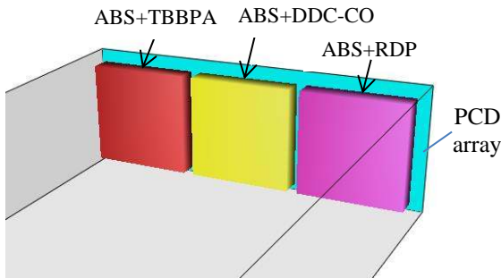
Figure 1: Simulated radioscopy system scheme (X-ray source is too far to be visible).
