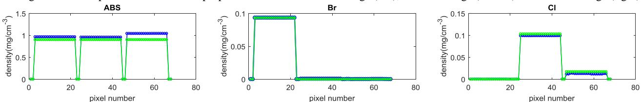
Figure 3: 1-D profiles along dash lines in Figure 2. Green curve represents the theoretical density of basis materials if the decomposition is perfect, blue curve represents our measurement: ABS basis (left), Br basis (middle) and Cl basis (right).
