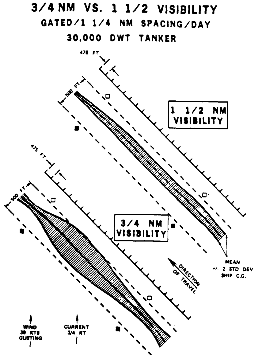
Figure 12 Navigational performance for gated buoys spaced 3/4 nautical mile apart and 1-1/2 nautical miles apart*
