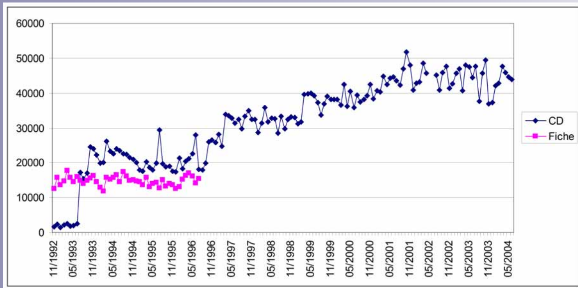
Figure 1: Monthly FBIS Volume, November 1992–June 2004
