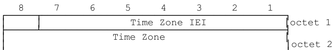
Figure 10.67a/GSM 04.08 Time Zone information element
