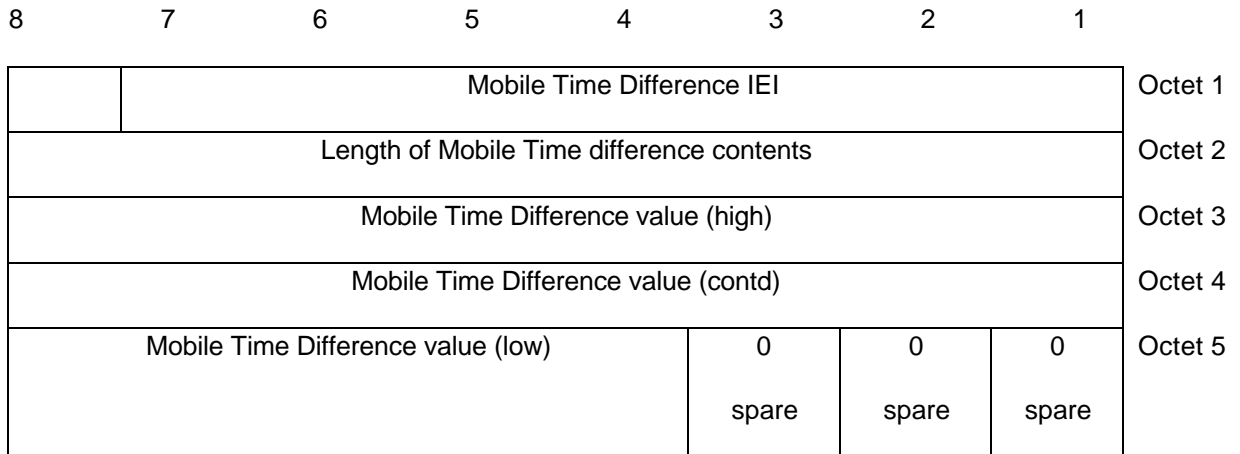
FIGURE 10.39a/GSM 04.08 Mobile Time Difference information element
