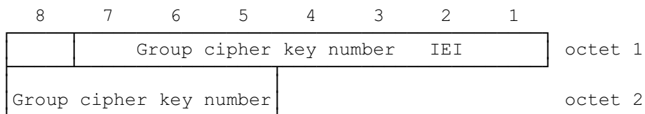
FIGURE 10.8"/GSM 04.08 Descriptive group or broadcast call reference
