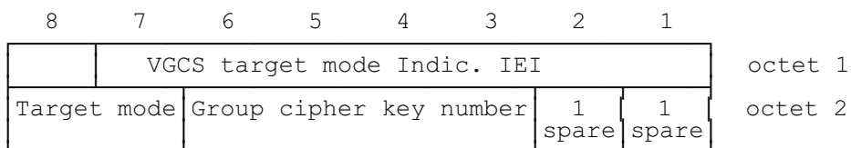
FIGURE 10.44f/GSM 04.08 VGCS target mode Indication information element
