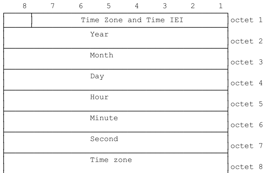
Figure 10.68a/GSM 04.08 Time Zone and Time information element
