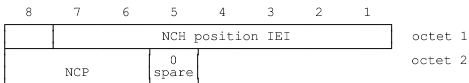
FIGURE 10.44c/GSM 04.08 NCH Position information element
