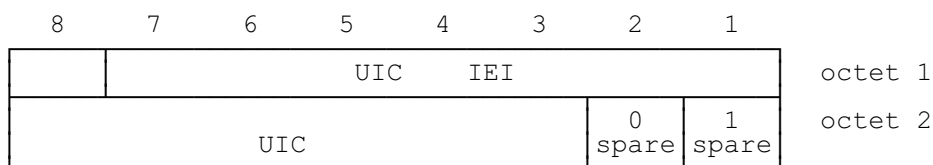
FIGURE 10.44h/GSM 04.08 UIC information element
