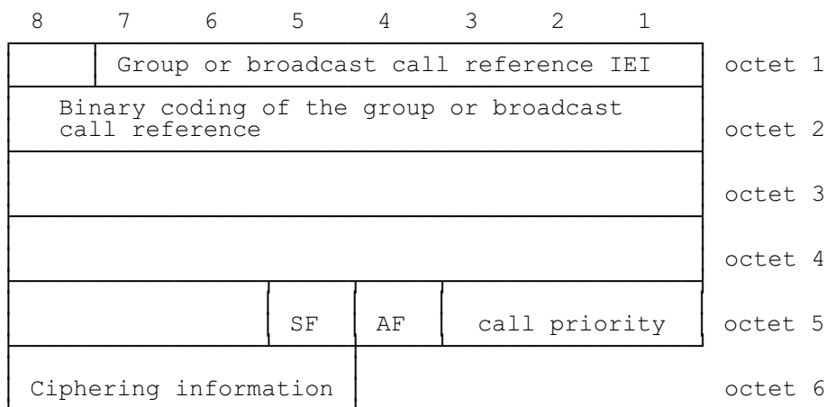
FIGURE 10.8/GSM 04.08 Descriptive Group or Broadcast Call Reference
