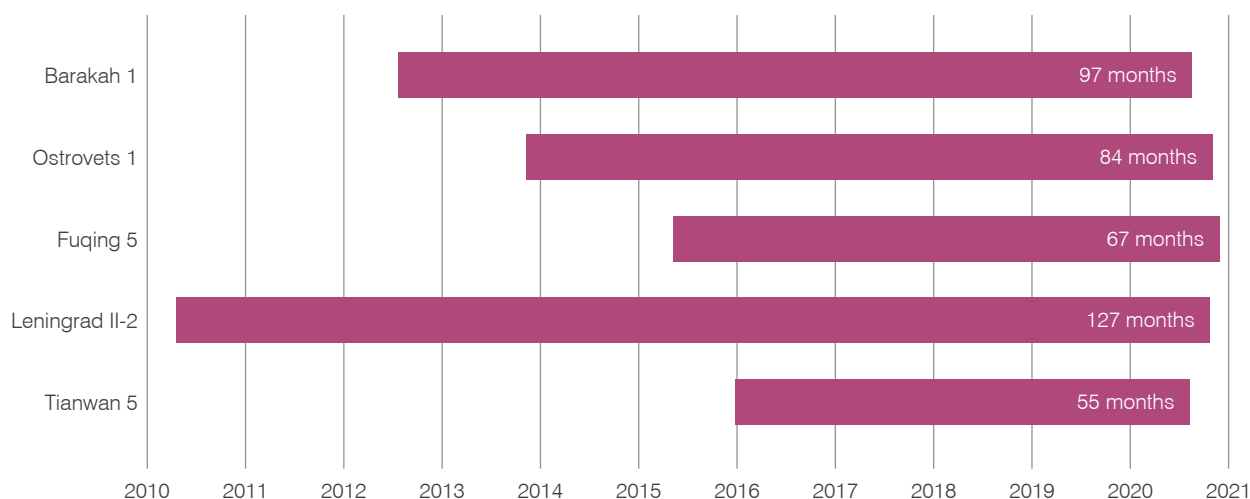
Figure 10. Construction times of new units grid connected in 2020
