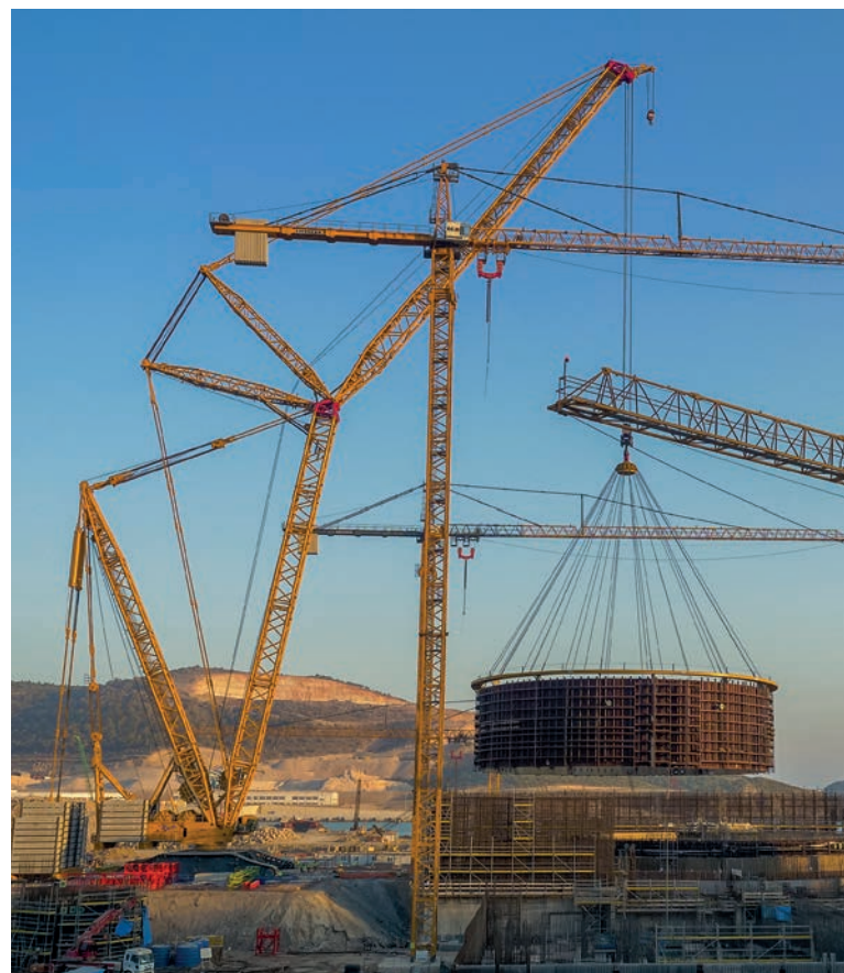
June 2020, Unit 1 reactor building inner containment second tier installation (Image: Akkuyu image bank, ROSATOM)
