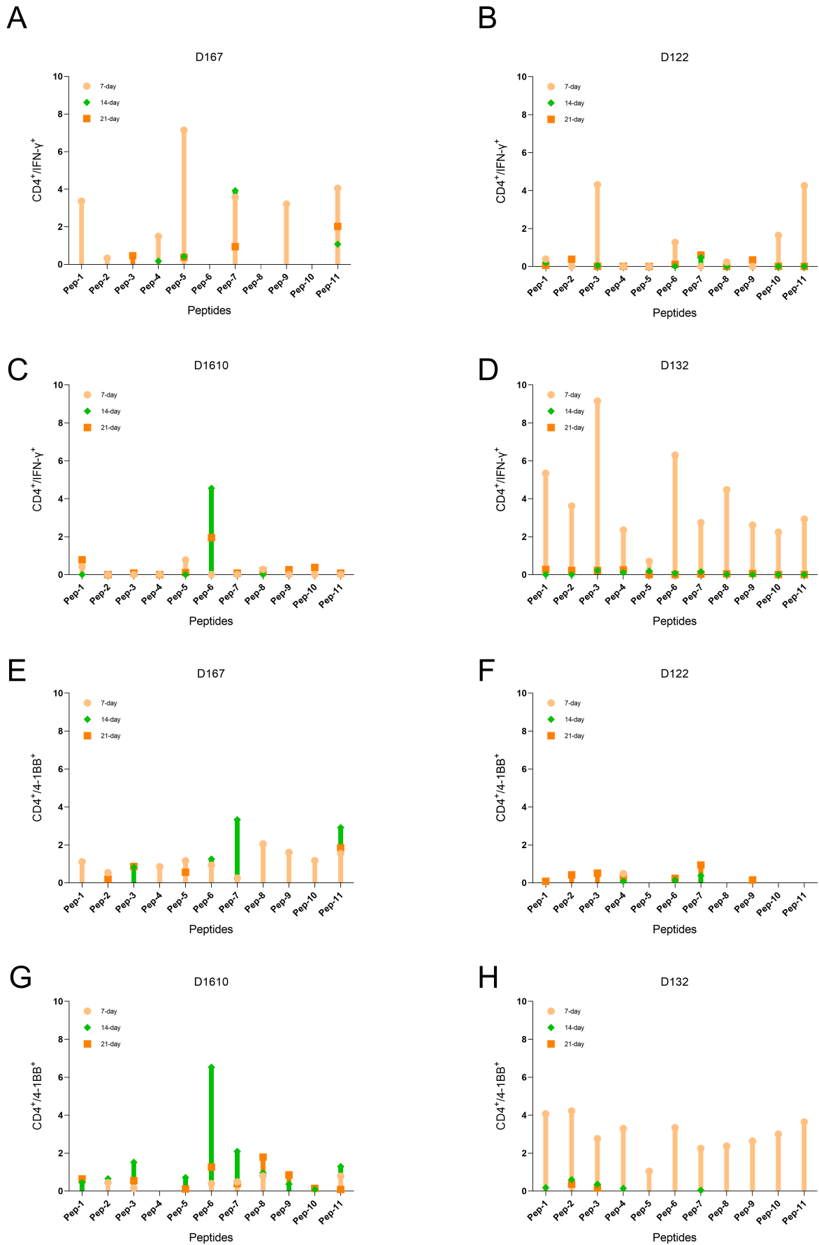
Figure S3. A-H. Kinetics and magnitude of IFN- \gamma and 4-1BB expression by CD4 T-cells in the presence of individual peptides in unexposed donors.
