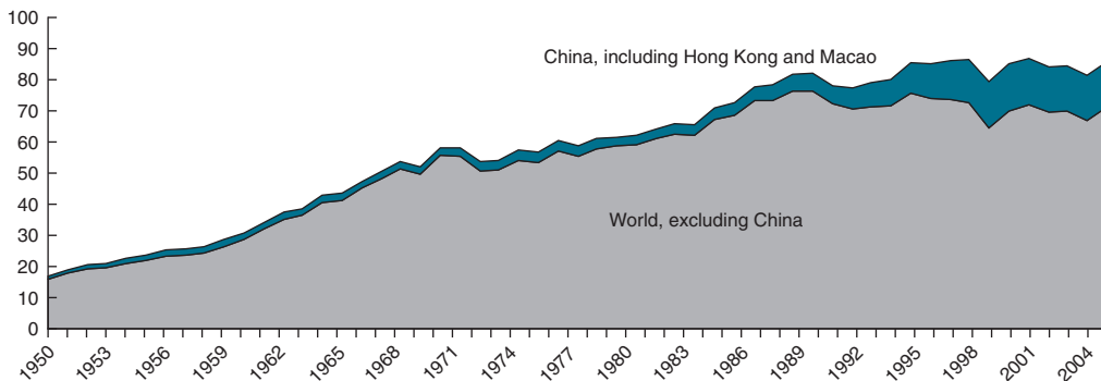
Figure 5.2 Total marine fish catch has leveled off
