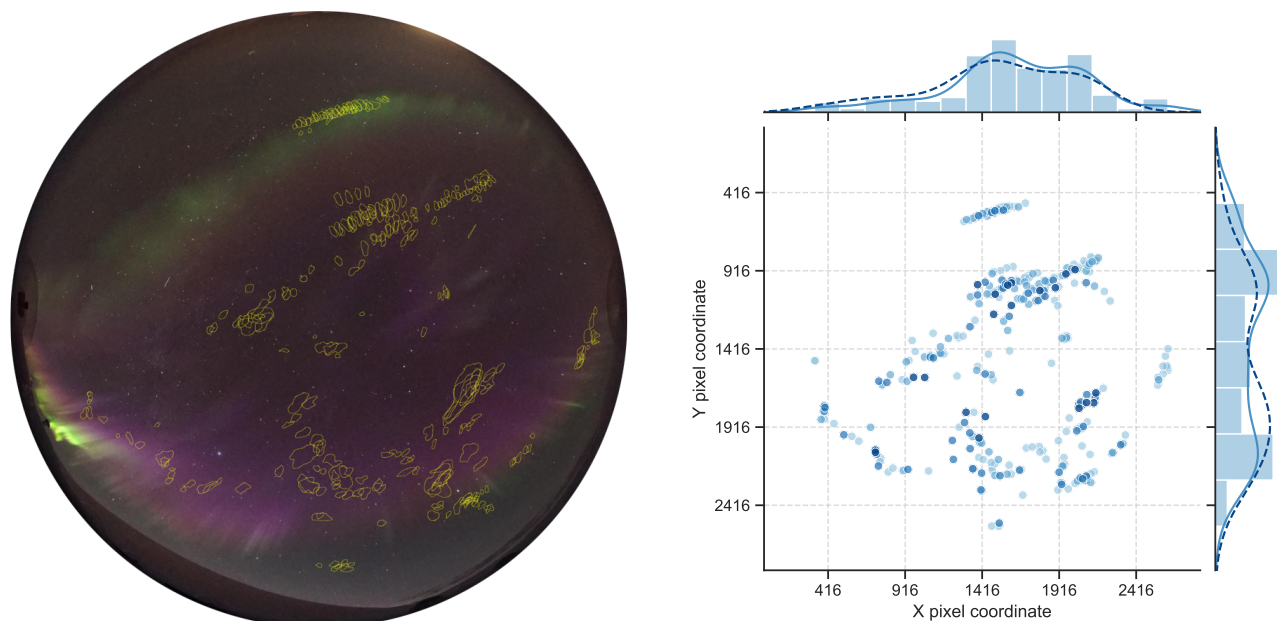
Figure 1. Left: All 262 marked FAE candidates for event 3, overlaid on the first image of the series taken at 07:36:35 UT. Geomagnetic east corresponds to the left side of the image, geomagnetic north to the top. Right: All 305 FAE locations in horizontal and vertical pixel coordinates with histogram distribution and kernel density estimation (KDE). FAEs are shaded according to confidence groups, with darker shades being FAEs of higher quality. The dashed KDE line is only calculated for FAEs of groups 1 and 2. Credit: ASC image provided by the KHO.
