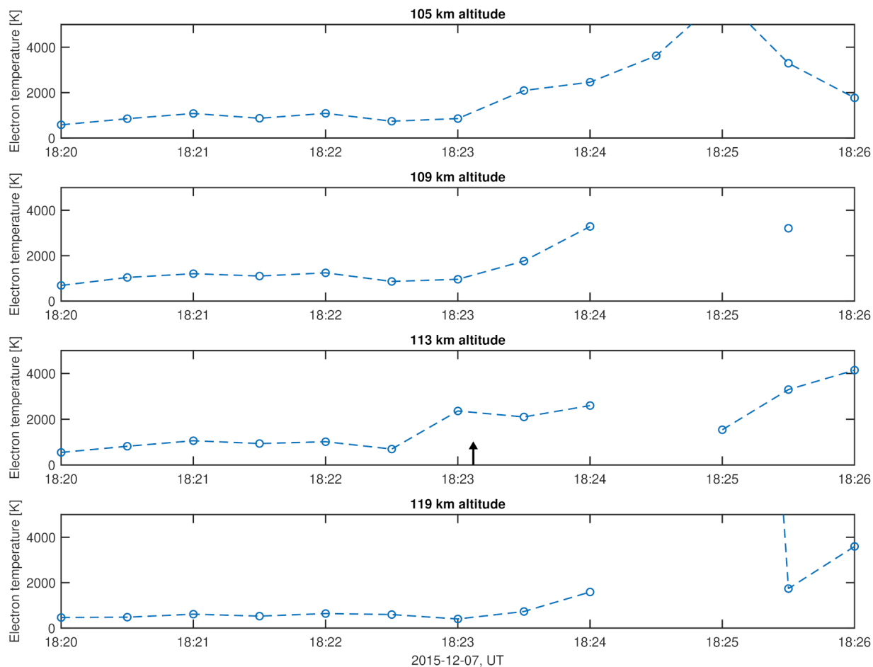
Figure 7. Time series of electron temperatures at four successive altitudes between 105–119 km from incoherent scatter data from the ESR (analysed with GUIDAP) for 18:20–18:26 UT on 2015-12-07. Data points with errors > 50\% of the values were removed. The arrow marks the time of the FAE passing and denotes the distinct increase in electron temperature specifically at 113 km.
