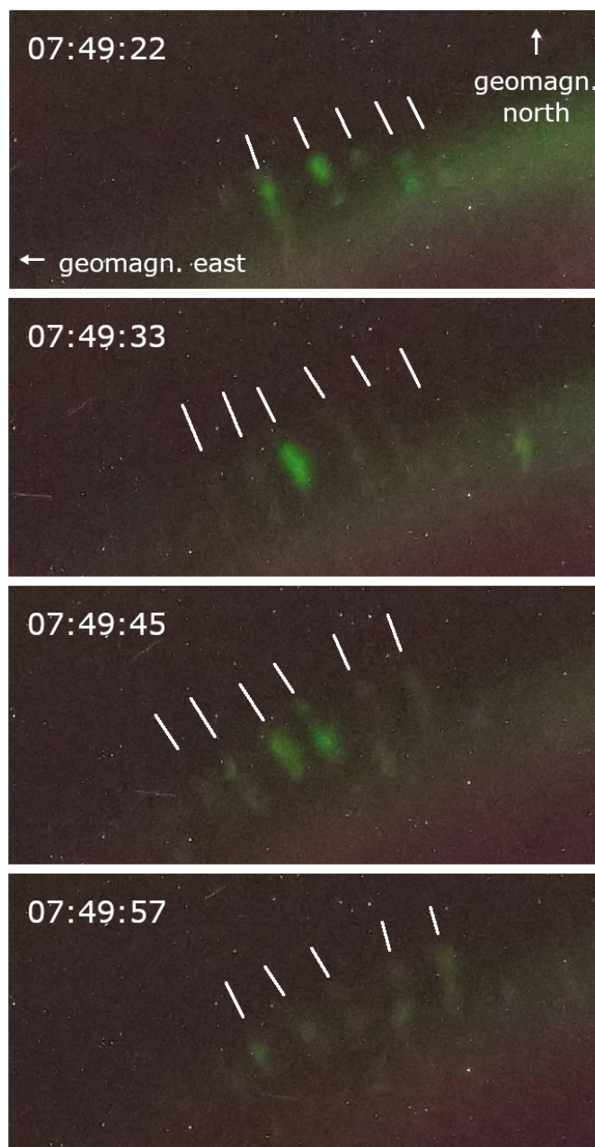
Figure 3. Movement of a category 2 FAE group northwards of the main auroral arc (northwest of zenith) over four successive images taken on 2017-12-18 around 07:49:40 UT. The images are cropped to 1250 \times 660 pixels to make the FAEs easily identifiable. White lines indicate the apparent alignment of the FAEs and were used to determine approximate distances between them. Credit: ASC images provided by the KHO.
