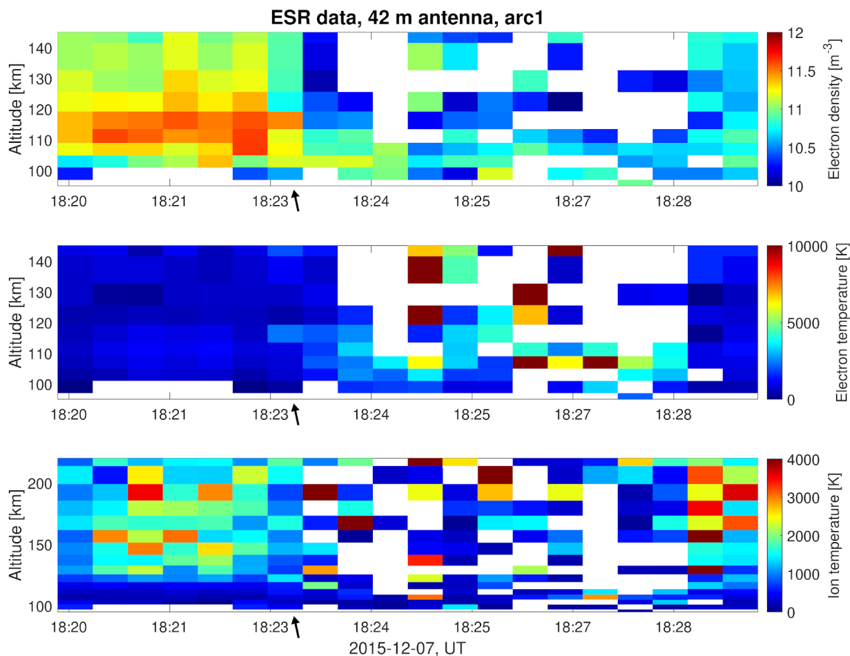
Figure 6. Incoherent scatter data from the ESR (analysed with GUISDAP) for 18:20–18:30 UT on 2015-12-07, with electron densities in the upper, electron temperatures in the centre and ion temperatures in the lower panel. Data points with errors > 50\% of the values were removed. The arrows mark the time of the FAE passing.
