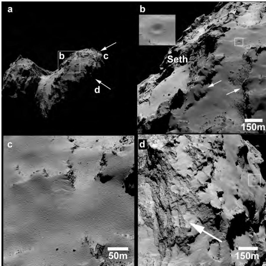
Fig. 5. WAC image showing most of the Ash region on the comet's body (right lobe). [b]: NAC image showing the smooth nature of the dust covering the Ash region. Box shows the location of the 40 meters-wide candidate impact crater, which is highlighted in the inset. Arrows show locations where units resembling Seth's brittle material are exposed from beneath the dusty coating (see section 3.1.4). An anaglyph of this figure is available as online supplementary material. [c]: NAC image showing another close-up of the Ash region at higher resolution. [d]: NAC image showing an exposed region in Ash below the dusty coating that shows terracing and layering. The box outlines the same crater displayed in [b] for orientation.
