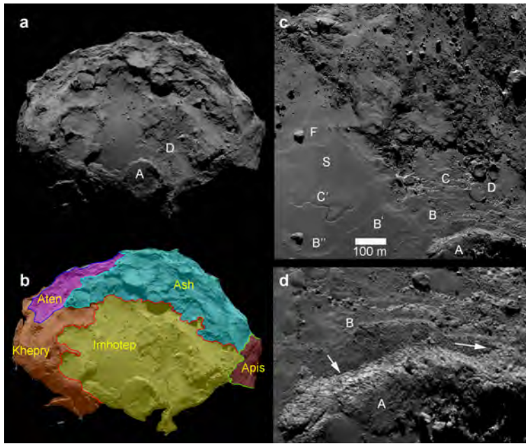
Fig. 4. [a, b]: WAC image of Imhotep region and a similar view with colorized regions overlapped. The Imhotep region borders The Khepry, Ash and Apis regions in addition to at least one currently non-illuminated region. [c]: NAC image showing the smooth deposits (S), linear features (features B', B'', and C'), circular mounds (D), possible terraces (B and C), a 40-meters-wide boulder (F) and circular mesa (A). [d]: A close-up of the same image for the circular mesa showing the fractures that appear to form polygonal patterns in some locations (see arrows).
