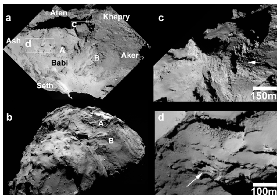
Fig. 9. [a] NAC image showing the Babi region and its surroundings. To view more accurate regional boundaries refer to the online supplementary material. [b] Cropped WAC image showing an oblique view of the comet's body centered at Babi. Note the dark-toned material (A), which corresponds to exposed cliff material and the ridge (B) that separates Babi from Aker. Similar ridges separate Babi from Seth and Ash. [c] A crop of NAC image showing the diamond-shaped mesa that separates Babi from the Khepry region. Notice the presence of bright boulders in the foot of the mesa's scarp (arrow). [d] A crop of NAC image showing the layering in Babi in proximity to Aten's depression.
