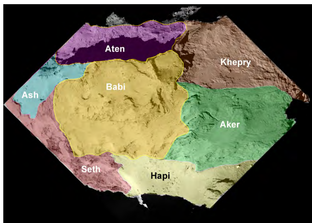
Fig. 10. NAC image showing the regional boundaries and nomenclature superposed over figure 8a
