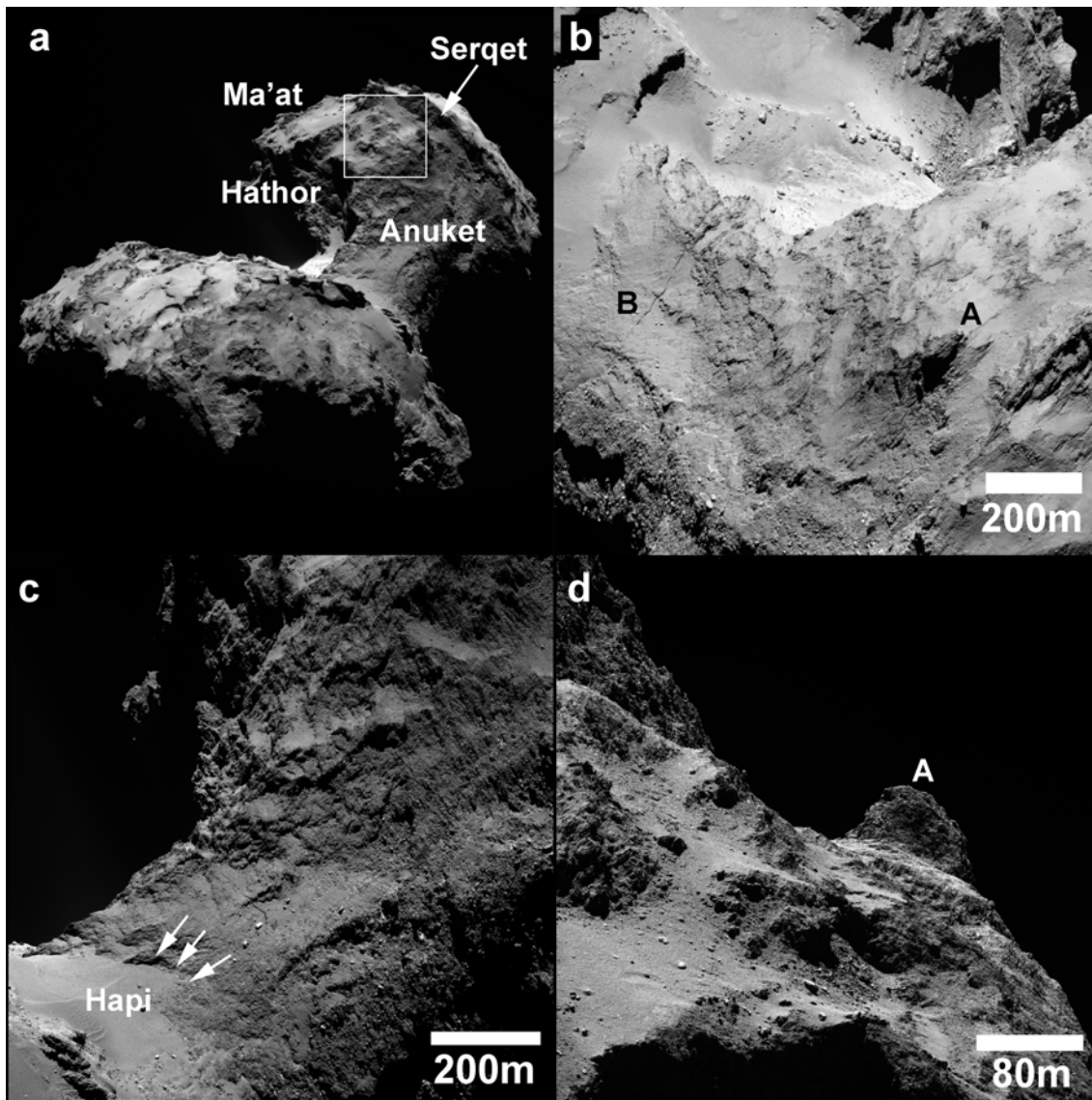
Fig. 19. [a] WAC image showing the Anuket region. Note the sharp scarp that separates it from Hathor and the ridge (arrow) that separates it from Serqet. The box shows the approximate location of [d]. [b] A crop of NAC image showing the Anuket region in more detail. The region shows a distinctive morphology resembling melted-wax texture. Overall, the region is rough but smoothen out a little as it approaches Ma'at (towards the right of the image). A notable feature in Anuket is a \sim 500 m-long fracture that runs across the region (feature B). A particular knob (A) is marked to correlate it with another viewing angle in [d]. [c] NAC image showing another view of Anuket at different lighting conditions, which highlights the region's distinctive texture. Note the absence of lineations that dominate the adjacent Hathor region. Arrows point to parts of the boundary between Anuket and Hapi [d] NAC image taken at low orbit ( \sim 10 km) showing part of Anuket that is relatively smooth, which can be shown in this image to be caused by partial burial of the region by patches of debris resembling that of Ma'at. This image is a strong indicator that the Anuket surface material may extend below the Ma'at debris.
