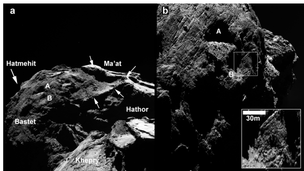
Fig. 24. [a] WAC image showing the Bastet region and its surroundings. The arrow points to the approximate location of Hatmehit behind the horizon. Note the unit's darker tone with respect to Ma'at and Khepry. (A) and (B) point to alcoves showing evidence for mass wasting. The features are further highlighted in [b]. Arrows point to locations of the boundaries between adjacent regions [b] NAC image showing the Bastet region in higher spatial resolution. The region is characterized by pervasive fracturing that is roughly oriented parallel to the plane of Hatmehit but occasionally displays cross-cutting relationships. Fractures appear to form polygonal patterns as well in some locations (see inbox).
