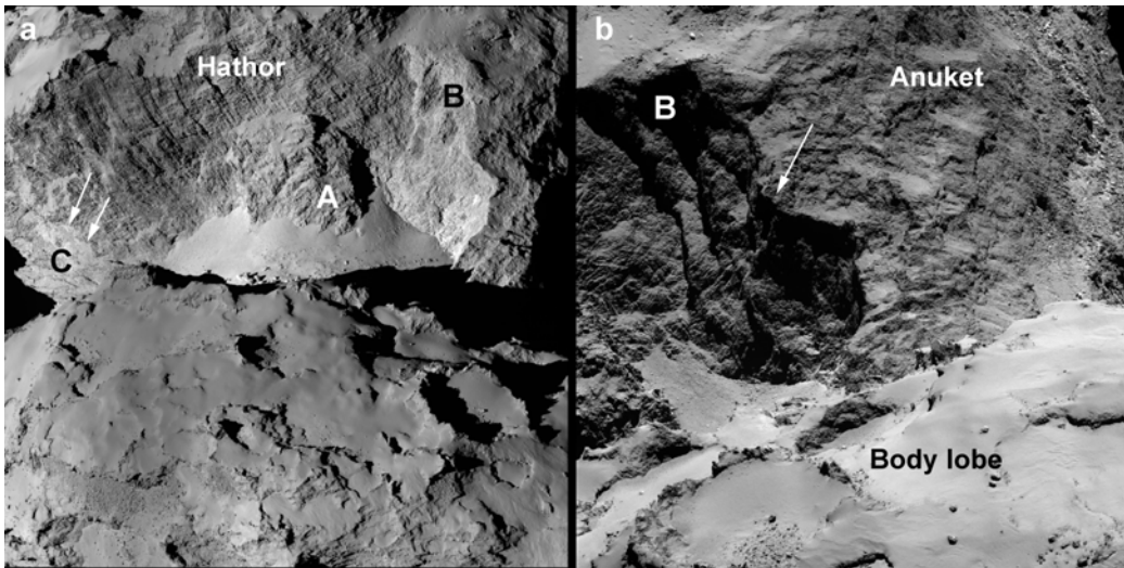
Fig. 16. [a] NAC image showing the Hathor region with the body lobe in the foreground. The region comprises a cliff-like structure with rectilinear lineations that distinguish it from other consolidated and fractured regions such as Bastet (boundary highlighted by arrows). Notable features in the region include an alcove structure that appears brighter and smoother than its surrounding at this illumination angle (B) and protruding, possibly detached, block of material (A) that shows similar surface features to the background. Anaglyphs of this image, as well as [b], are available as online supplementary material (Fig. 17), which highlights the complex morphology of the cliff and the transition to Bastet at feature (C) and associated arrows. [b] NAC image highlighting the alcove structure (B), which in this viewing geometry shows longitudinal terraces, which could hint at concentric layering of the head lobe. Notice the sharp contact with Anuket (arrow), which further suggests that Hathor is an outcrop for the internal structure of the comet below the overlying Anuket materials.
