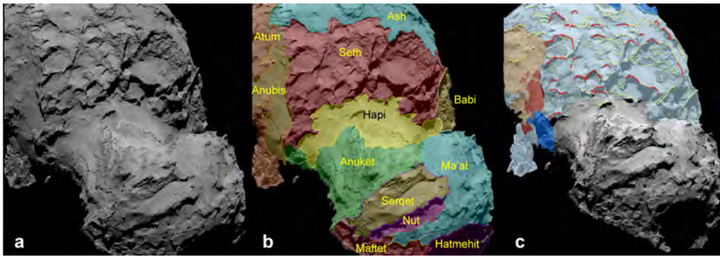
Fig. 1. [a] NAC image of comet 67P/C-G showing many of the regions discussed in this paper. [b] Same image with regional boundaries and nomenclatures added. [c] NAC image showing a similar, but not identical, view of the comet with superposed geological/geomorphological units to highlight the differences between both techniques. Refer to the main text for details. For original image IDs of this figure in addition to all other figures in the paper, please refer to table 3 in the online supplementary material.
