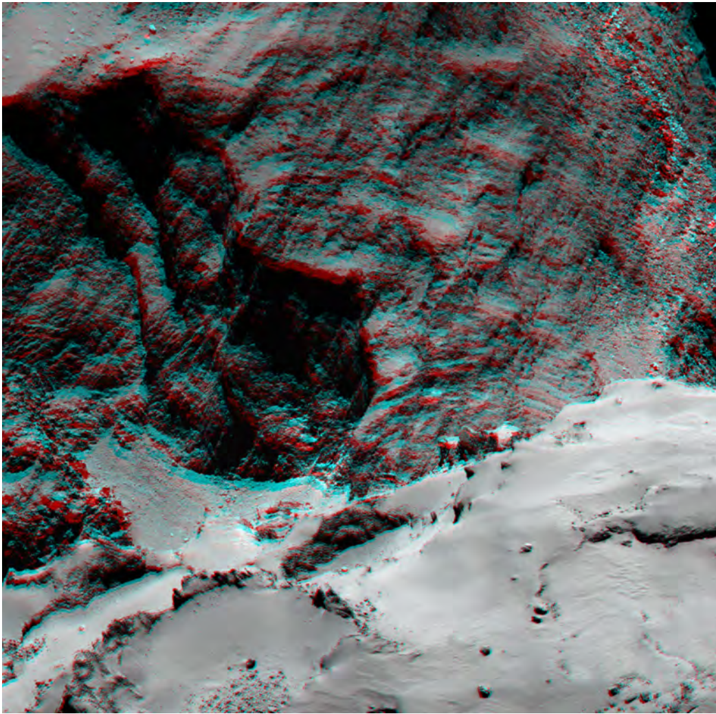
Fig. 18. Anaglyph version of figure 13b in the main text.
