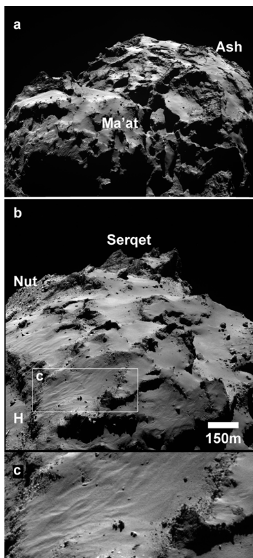
Fig. 20. [a] WAC image showing a view of the comet with the head lobe in the foreground showing the light-toned Ma'at region. Note the morphological similarity with the Ash region on the body lobe. [b] NAC image showing a significant part of the Ma'at region and its surroundings. Feature (H) corresponds to the Hatmehit region. The Ma'at region is generally smooth in texture and almost featureless except for the regions around the Hatmehit depression where the debris appears striated (inbox). [c] Close-up of box in (b) showing the ripple-like features in Ma'at that are common around the Hatmehit depression. The features appear to be aligned perpendicular to the depression's rim.
