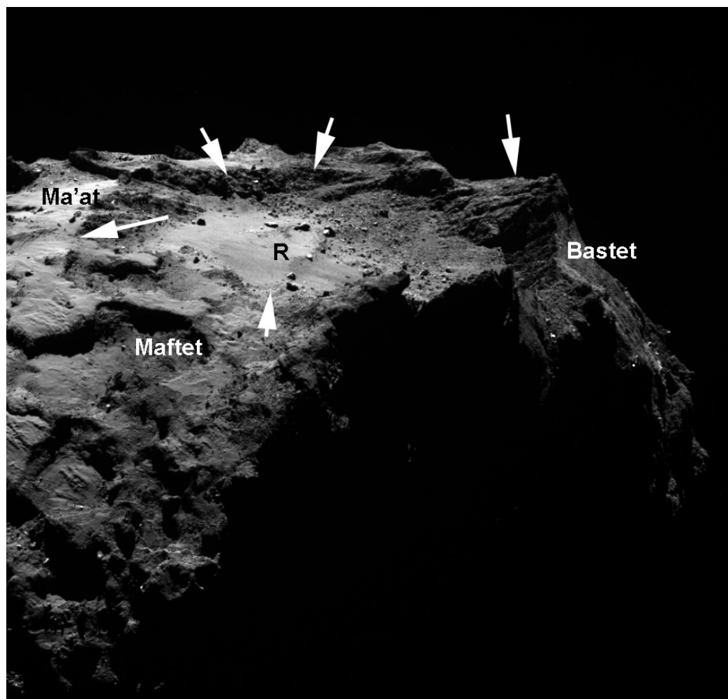
Fig. 25. WAC image showing an oblique view of the Hatmehit depression and the regions surrounding it. Note the smooth morphology of the interior, the talus-like debris occupying parts of the depression on Bastet's side and the curvilinear ridge (feature R) that appears to traverse through the central part of the depression. Arrows highlight the depression's rim.
