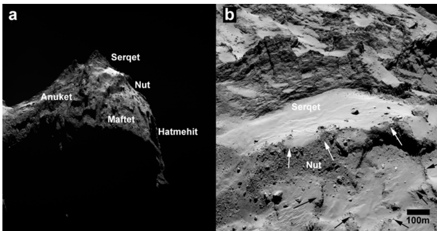
Fig. 21. WAC image showing a side view of the Serqet and Nut regions. Serqet is mainly composed of ridge, which separates it and other region on the distal part of the lobe from the inner regions towards the neck, and a smooth flat plain that forms the rim of the Nut depression. [b] NAC image highlighting the morphological features. Note that both Serqet and Nut are covered by patches of Ma'at debris, which is occasionally striated. In addition, the part of Nut region adjacent to Serqet plain material is covered by boulders and talus that may have formed through the erosion of the Serqet region. Arrows point to locations of the boundary between Nut and Serqet as well as its surroundings.
