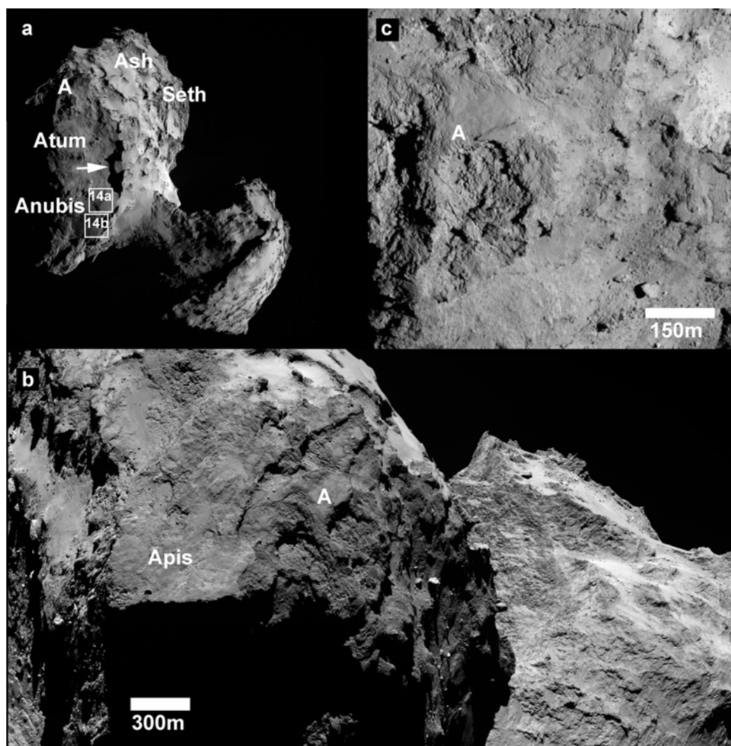
Fig. 12. [a] WAC image showing the side of the comet with Atum and Anubis regions on the body lobe. “A” marks the location of a complex depression that is highlighted in [b] and [c] as well. Boxes show the locations of Figures 14a and 14b while the white arrow shows the ridge separating Seth and Anubis, which is further highlighted in Figure 14c. [b] NAC mosaic of two images showing an oblique view of the Atum region, its contact with Apis, and feature “A”. Note the rough and pitted texture, and limited number of boulders. An anaglyph version of this figure is available as online supplementary material. [c] Cropped NAC image showing part of the Atum region concentrating on feature “A”.
