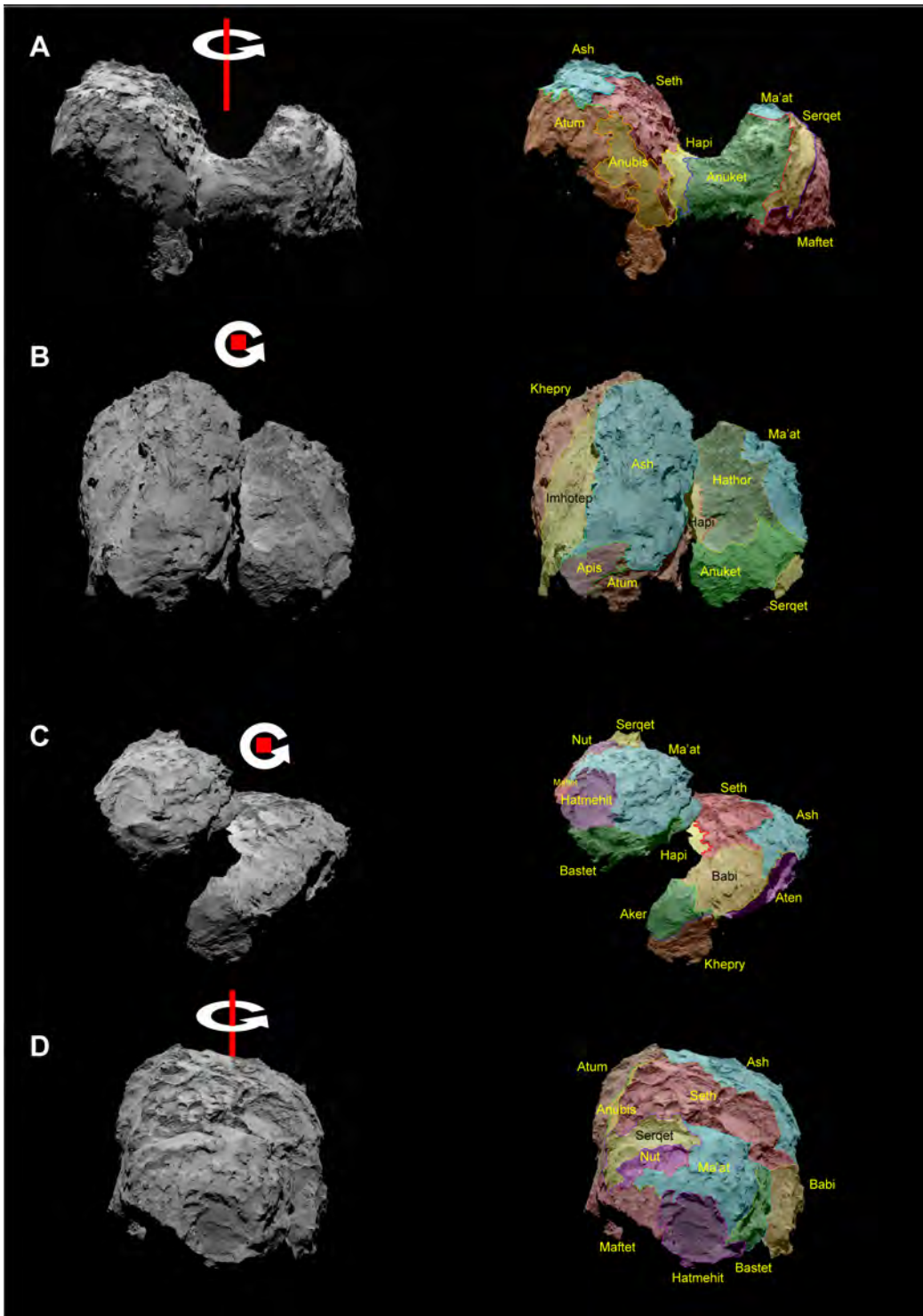
Fig. 2. [Left]: WAC (panel A) and NAC images (the rest) showing the comet in different orientations. Rotation axes have been added for better orientation. In panels B and C, the rotation axis is almost towards the viewer (north polar view). [Right] Same images with regional boundaries and nomenclature superposed.
