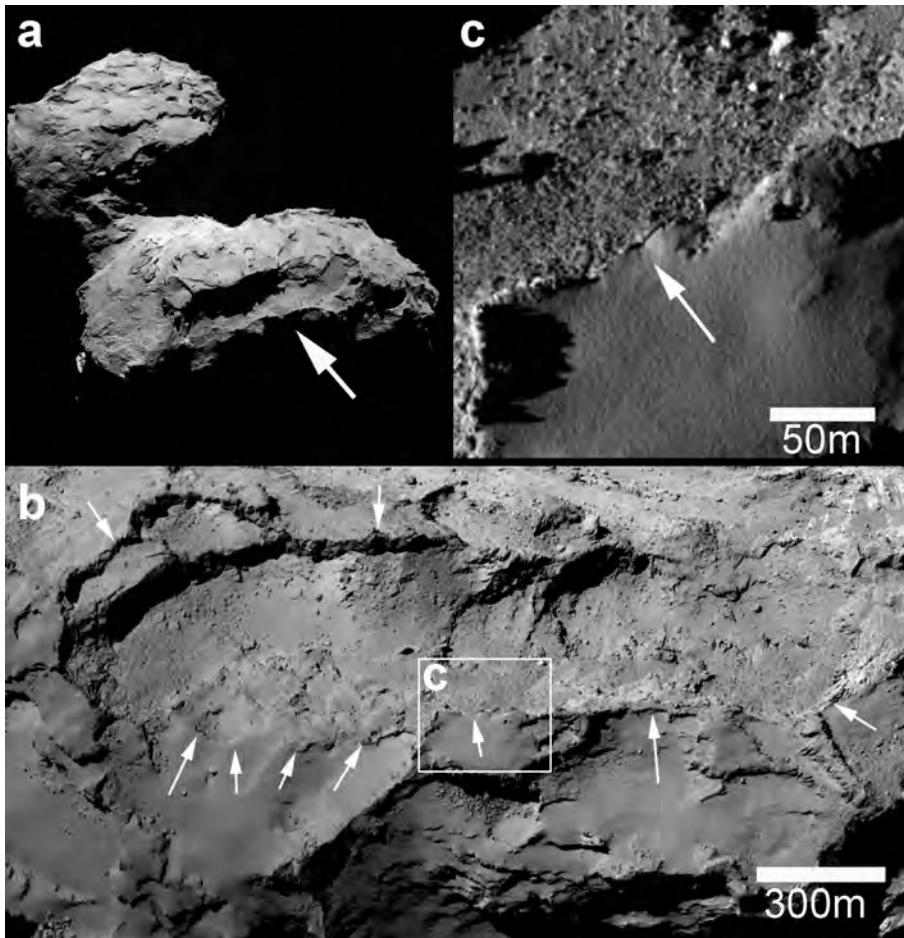
Fig. 8. [a]: NAC image showing the location of the Aten region on the comet's body. The region is mainly composed of a large irregular depression. [b]: Cropped NAC image showing the Aten depression. Note the presence of talus-like deposits resulting from material falling into the depression and the lack of smooth deposits in the interior. Box shows the position of the close up in the upper right. Arrows highlight the rim of the depression. [c]: Cropped NAC image showing the different morphology between the Aten's interior and the smooth deposits that are part of the Babi region. Note the sharp and irregular shape the depression's scarps, which might be indicative of short-term, possibly violent, mode of formation.
