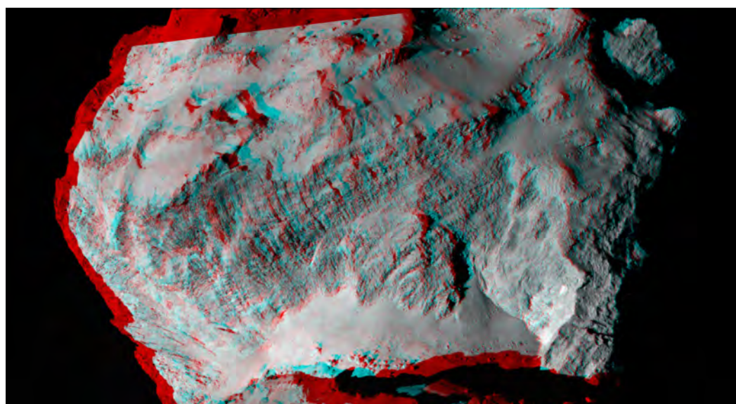
Fig. 17. Anaglyph version of part of figure 13a in the main text.
