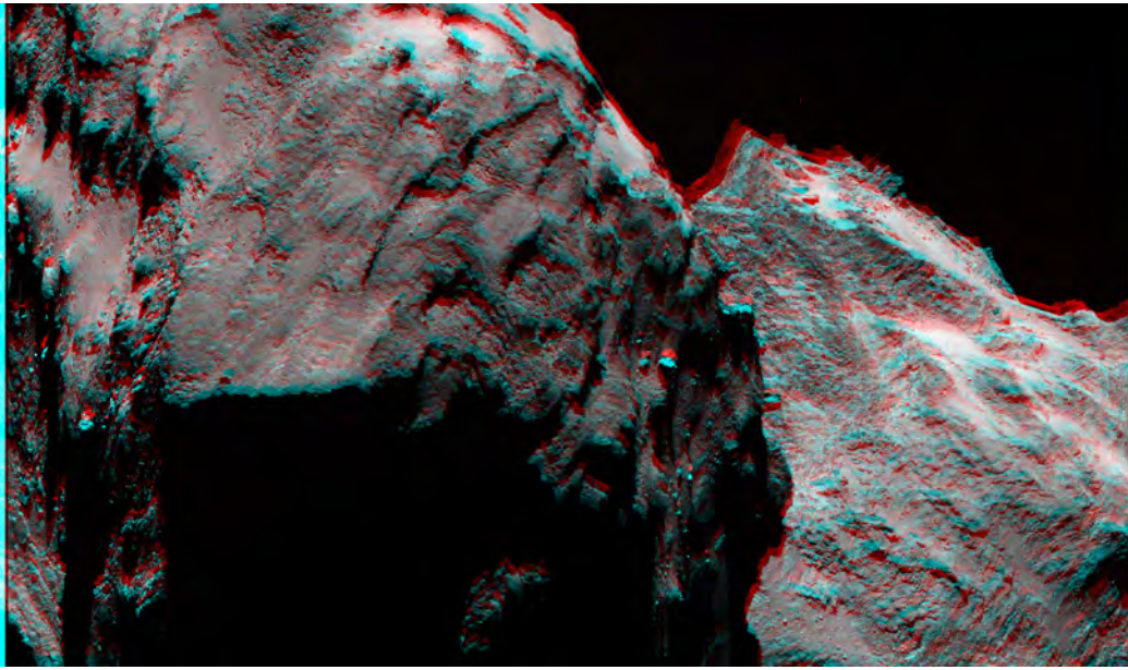
Fig. 13. Anaglyph version of figure 10b
