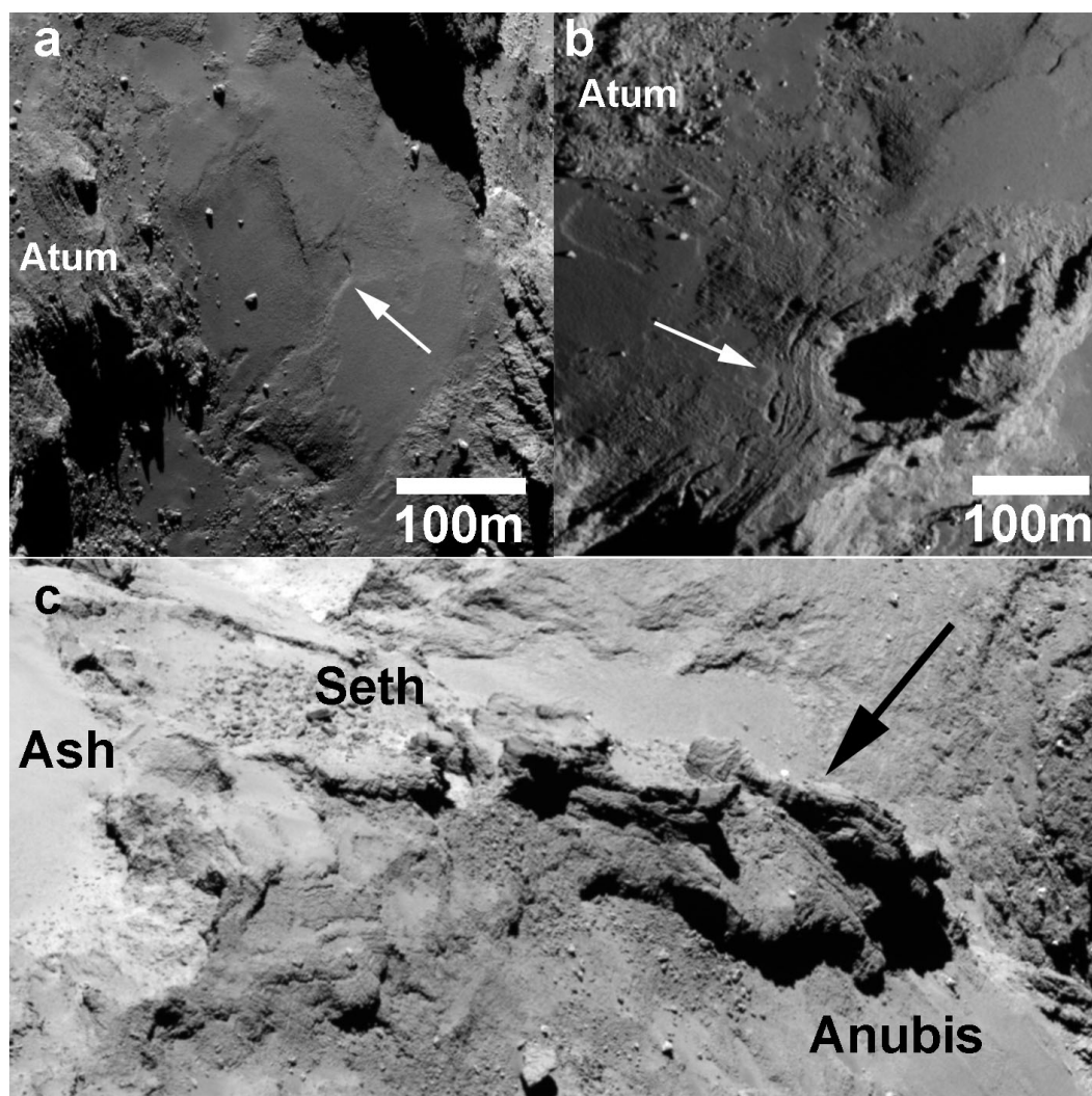
Fig. 14. [a] Crop of NAC image showing linear features in Anubis similar to Imhotep region. The Anubis region displays a considerable number of boulders, which may have originated from the Atum region. Note the smooth surface texture in comparison with the rough-textured enclosing regions of Atum and Seth. For context, refer to Fig. 12a. [b] Crop of NAC image showing possible folding in the Anubis deposits close to the boundary with Seth. [c] Crop of NAC image showing the ridge separating Seth and Anubis.
