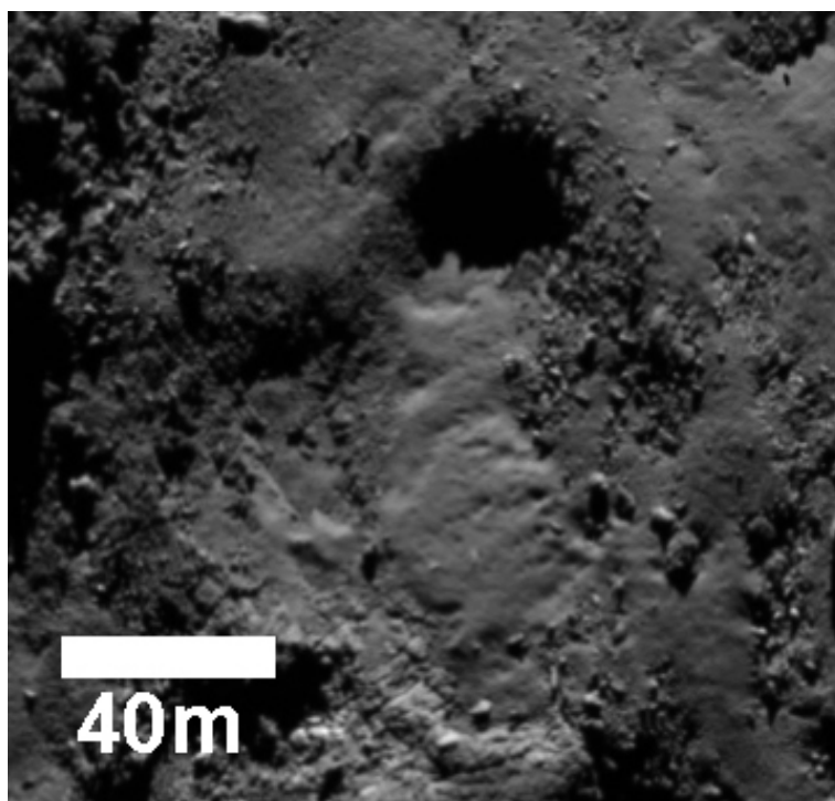
Fig. 23. Flow-like feature and associated pit in the Maftet region. The pit is ~35 meters-wide whereas the flow feature extends put for more ~75 meters.
