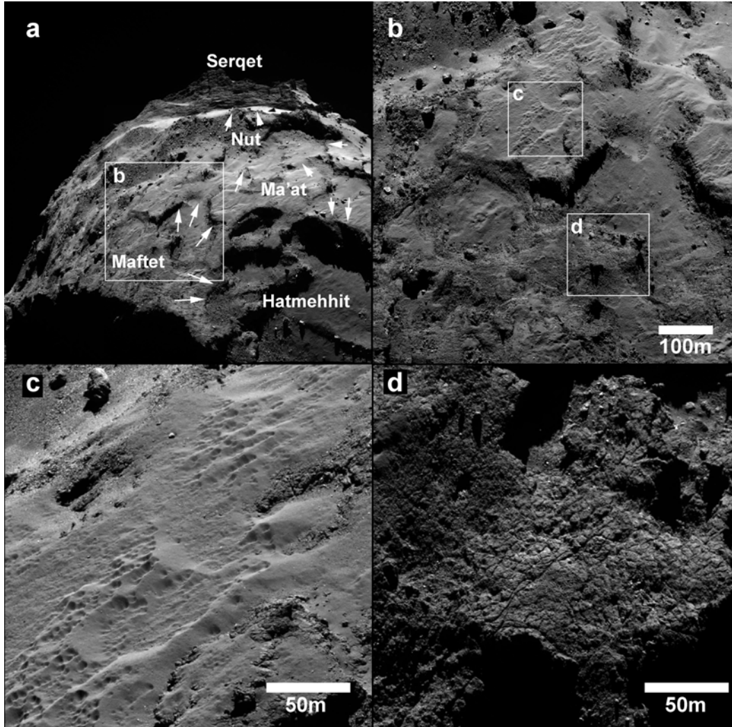
Fig. 22. [a] WAC image showing the Maftet region and its surroundings. Arrows point to locations of the boundaries between adjacent regions. [b] NAC image showing the surface morphology of the Maftet region. The region is mainly composed of rough and fractured terrain enclosing numerous irregular and heavily bouldered depressions. [c] Crop of NAC image showing the pitted texture in the debris at the boundary between Maftet and Ma'at. [d] Crop of NAC image showing the pervasive fracturing, which is a common feature in Maftet.
