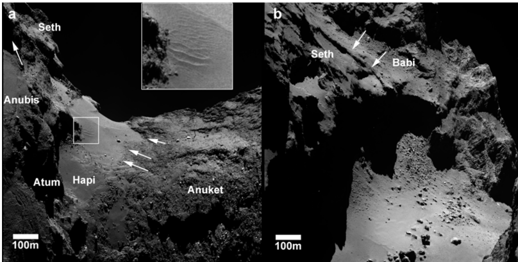
Fig. 15. [a] NAC image showing the section of Hapi facing the Anuket region. The region is distinguished by its smooth texture, which show surface ripples (inbox) indicative of dust mobilization by aeolian-like processes. The folded section of Anubis is visible as well in the bottom left corner. Note how the Anuket material appears to traverse the neck region in the lower section of the image creating a boundary with Atum. [b] NAC image showing part of the Hapi region facing the Hathor cliffs (outside the right bounds of the image), which is roughly beyond the horizon of [a]. Also visible in the foreground is the line of boulders along this section of the region in addition to the scarp boundaries with Seth and Babi. Arrows in both figures point to locations of the boundaries between adjacent regions.
