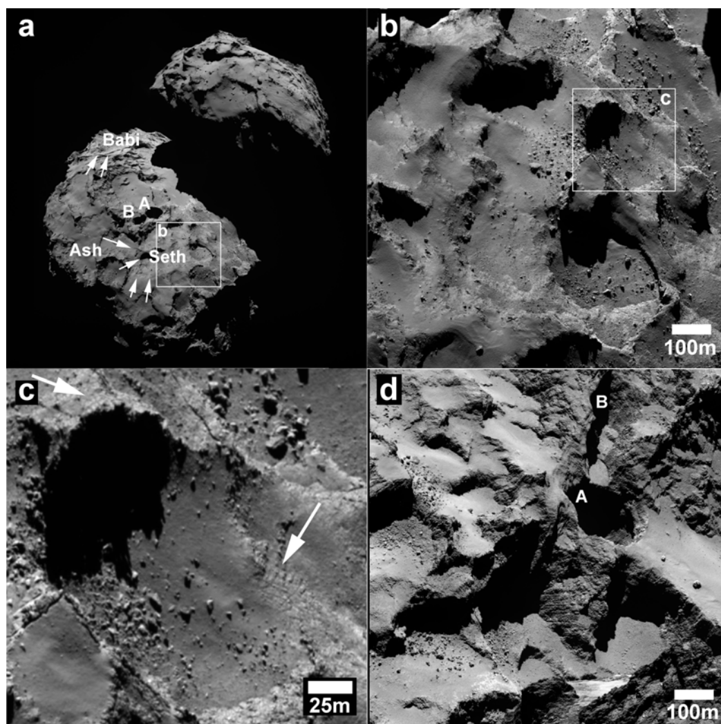
Fig. 7. WAC image showing the Seth region in addition to Ash and Babi. Arrows point to locations of the boundaries between adjacent regions. Also visible are a couple of circular pits (A and B). [b] Cropped NAC image showing prominent features of the Seth region. The material is light toned, brittle and susceptible to fracturing and collapse creating darker toned talus-like deposits as well as boulders. [c] Close up of [b] showing the fractures that often form polygonal patterns (arrows). [d] Cropped NAC image showing one of the most remarkable circular pits (A) on the surface of the comet as well as another pit (B), which together with pit A is part of a pit chain in the Seth region.
