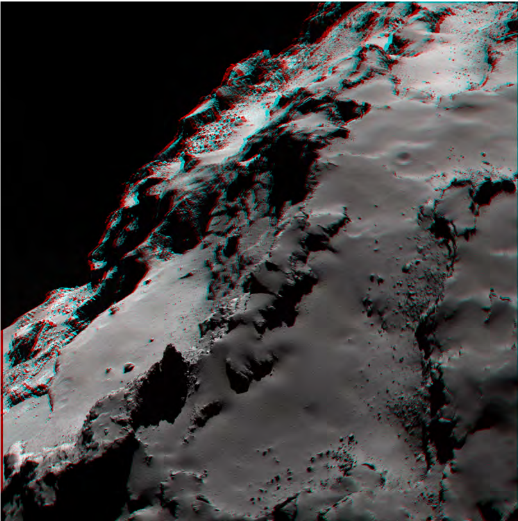
Fig. 6. Anaglyph version of Figure 5b in the main text
