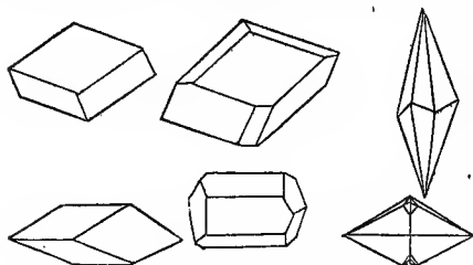
Calcareous Spar.—Various Forms of Crystals.
