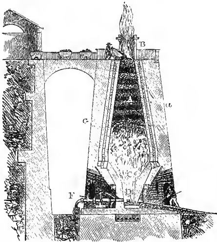
Blast Furnace.
