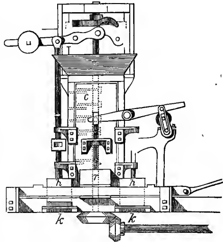
Brick-making Machine.
