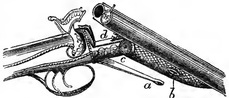
Breech-loading Rifle.
