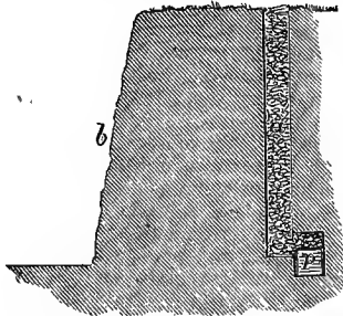
Vertical Section of Shaft : a , tamping; b , face of the rock; p , box for charge.
