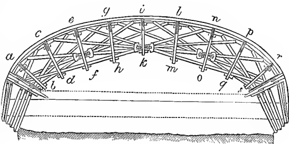
Centering of Waterloo Bridge.
