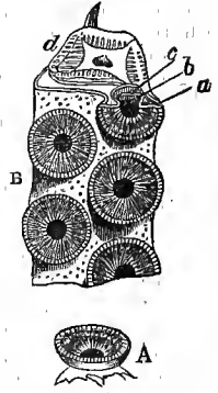
Cephalopoda, suckers of : A, a single sucker, side view : B, a portion of one of the tentacula, with several suckers, front view; a, cartilaginous circlet; b, central cavity; c, piston; d, section of the tentacle.
