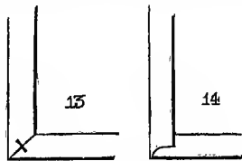
the common mitre, fig. 13; the lapped mitre, fig. 14; and the lapped and tongued mitre, fig. 15.
