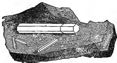
Beryl, in its primary form.
