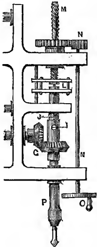
Boring Machine.
