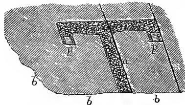
Sectional Plan of a Double Heading.
