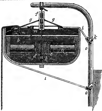
Transverse section of Boat.
