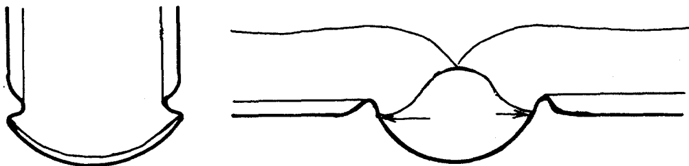
Fig. 11. Action of the tube hollow. Notice the reduced radius and lengthened arc of the backstrip, which is bent like a spring. The push of the backstrip is at the points and in the directions of the arrows.
