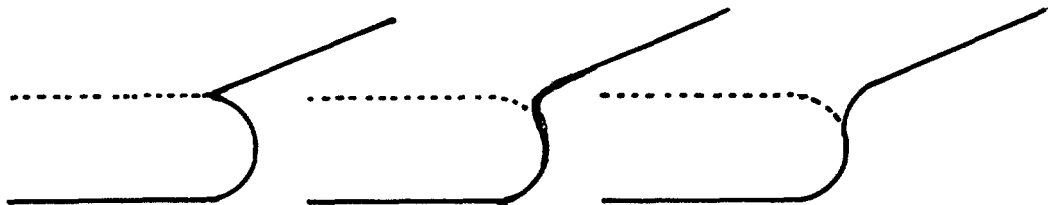
Fig. 43. Bending radius over the joint. When the bending radius of the covering material over the joint is small, the board can move almost independantly of the spine; as the bending radius increases, the influence of joint action on spine action increases.
