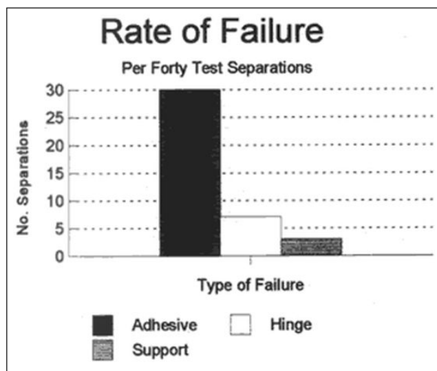
Fig. 5 Rate of failure per forty test separations - number of separations vs. type of failure
