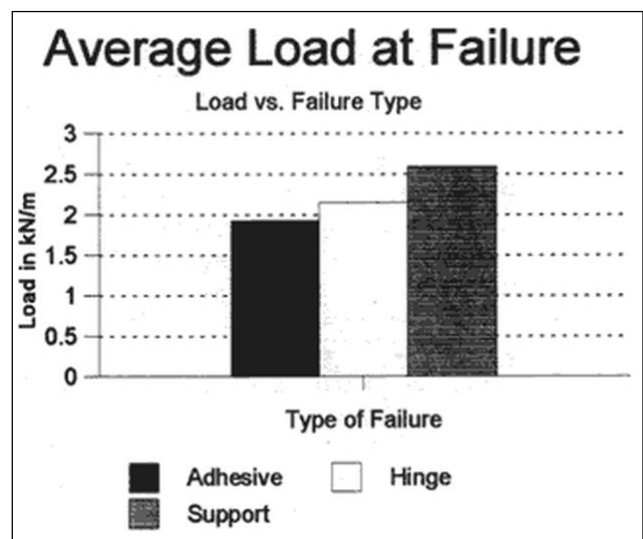
Fig. 6 average load at failure - load in kN/m vs. type of failure
