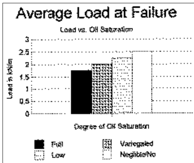
Fig. 13 Average load at failure - load in kN/m vs. degree of oil saturation
