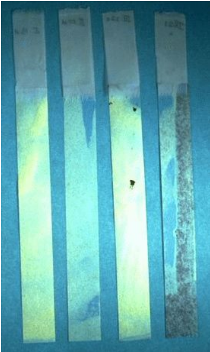
Fig. 15-16. UV/VIS Fluorescence. From left to right: Verso of samples I.13.d., II.20.d., III.22.c., IV.21.a. The more intense UV/VIS fluoresce reaction indicates that paint straight from the tube has a greater oil concentration than paint thinned with Winsor Newton oil painting medium
