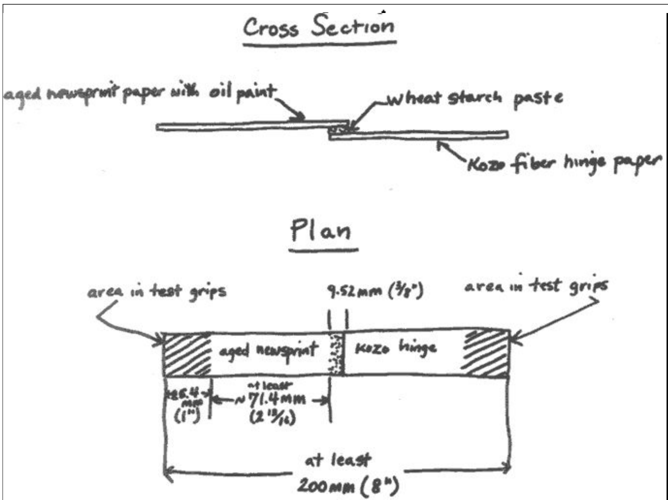
Fig. 3. Dimensions of test specimen
