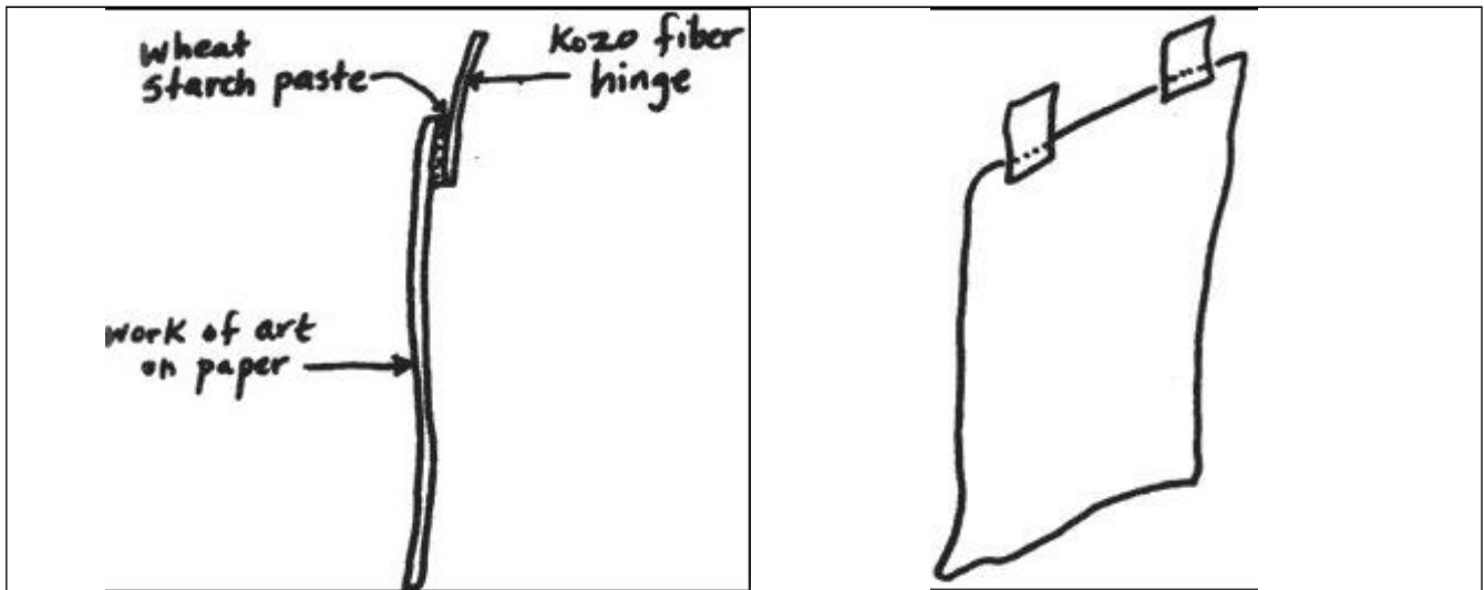
Fig. 1a. Side view of hinged work on paper
