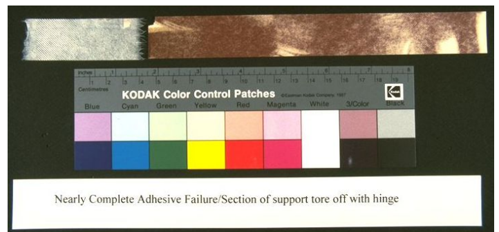
Fig. 19-20. Recto and verso of sample # IV.21.d. Adhesive failure with corresponding support failure
