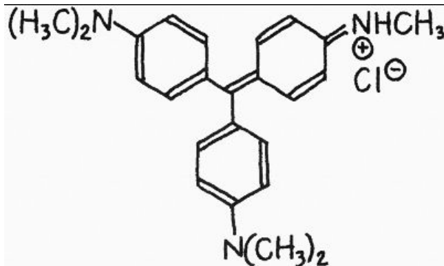
Fig. 4. Pentamethylpararosaniline hydrochloride, the primary species of methyl violet 2B (color index no. 42535)
