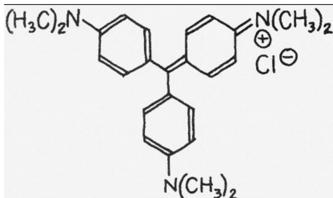
Fig. 3. Hexamethylpararosaniline chloride, or crystal violet (color index no. 42555)
