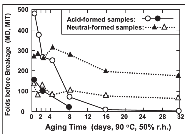
Fig. 9. Loss in folding endurance vs. time for light-weight-coated papers formed under acidic (circles) and near-neutral (triangles) conditions; figure redrawn (Lyne 1995).
