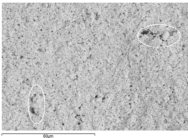
Fig. 5. Treated sample. Brush, 1:1 30% hydrogen peroxide and ether. 1000x magnification (SEM). Circled areas show possible physical alteration.
