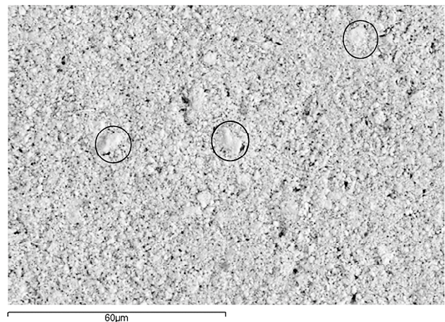
Fig. 4. Treated sample. Gel, <3% hydrogen peroxide, aq. 1000x magnification (SEM). Circled areas show particle agglomeration.
