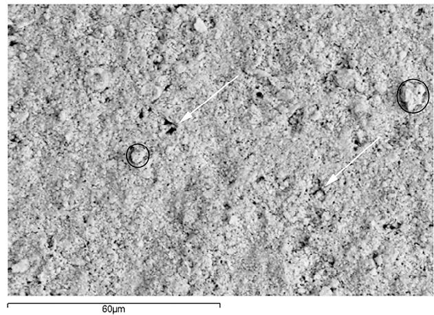
Fig. 2. Treated sample. Brush, 3% hydrogen peroxide, aq. 1000x magnification (SEM). Circled areas show particle agglomeration. Arrows point to complex pores.
