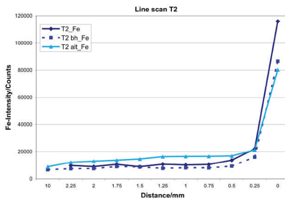
Fig. 14. Line scan on Lavater object T2: comparison of the intensities of the Fe-K \alpha -line of the untreated (line T2_Fe), treated (lining with wheat starch paste, line T2bh_Fe), and subsequently artificially aged sample (line T2alt_Fe).
