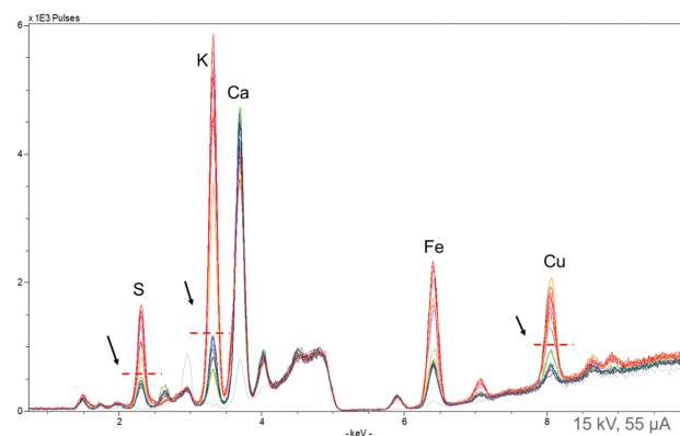
Fig 3. XRF spectra of paper spots from Quinta Europa (blue), Tabula Moderna Bossinae, Tabula Prima Africae, Tabula Prima Asiae, Nona Asiae Tabula, Tabula Secunda Africae, and air spectrum (grey); dotted lines and arrows indicate approximate demarcation of map groups in terms of elements associated with good vs. poor condition by dotted lines
