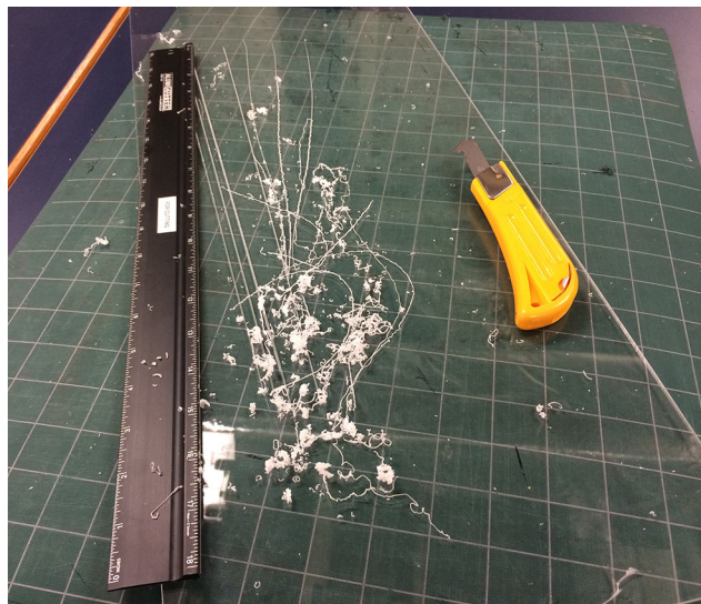
Fig. 1. Cut Plexi with Plexi cutter to make shavings to dissolve into paste.
