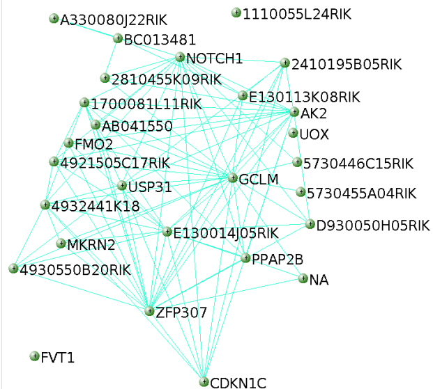
F. Network connections in brown module
