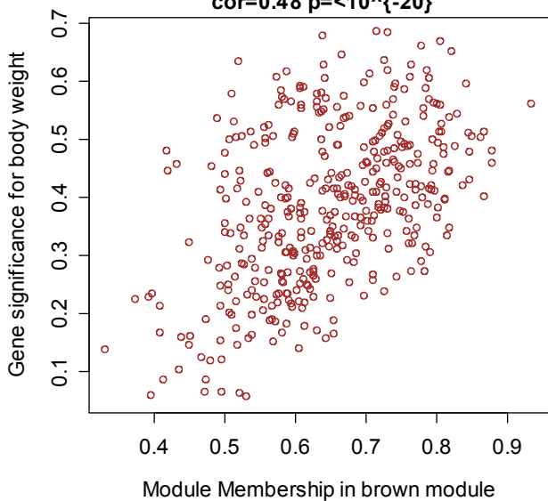
E. Module membership vs. gene significance brown module cor=0.48 p<10^{-20}
