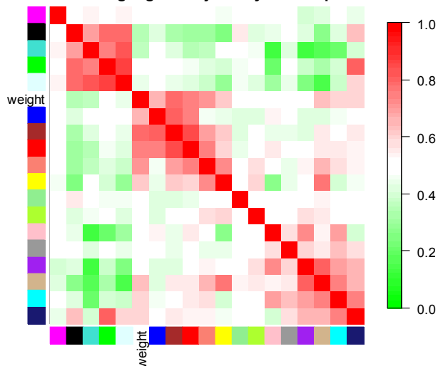
D. Eigengene adjacency heatmap
