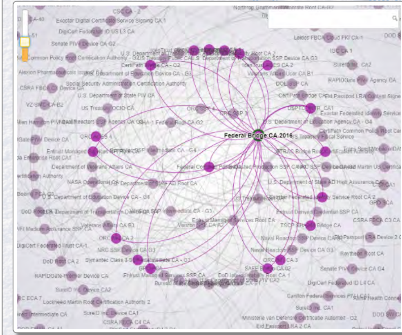
Fig. 13—Federal PKI Graph. (Accessed Nov. 17, 2018). Federal PKI Graph. (Accessed Nov. 17, 2018). Federal Public Key Infrastructure Guides. CIO.gov. Idmanagement.gov. GSA. https://fpki.idmanagement.gov/tools/fpkigraph/ PDF version.
