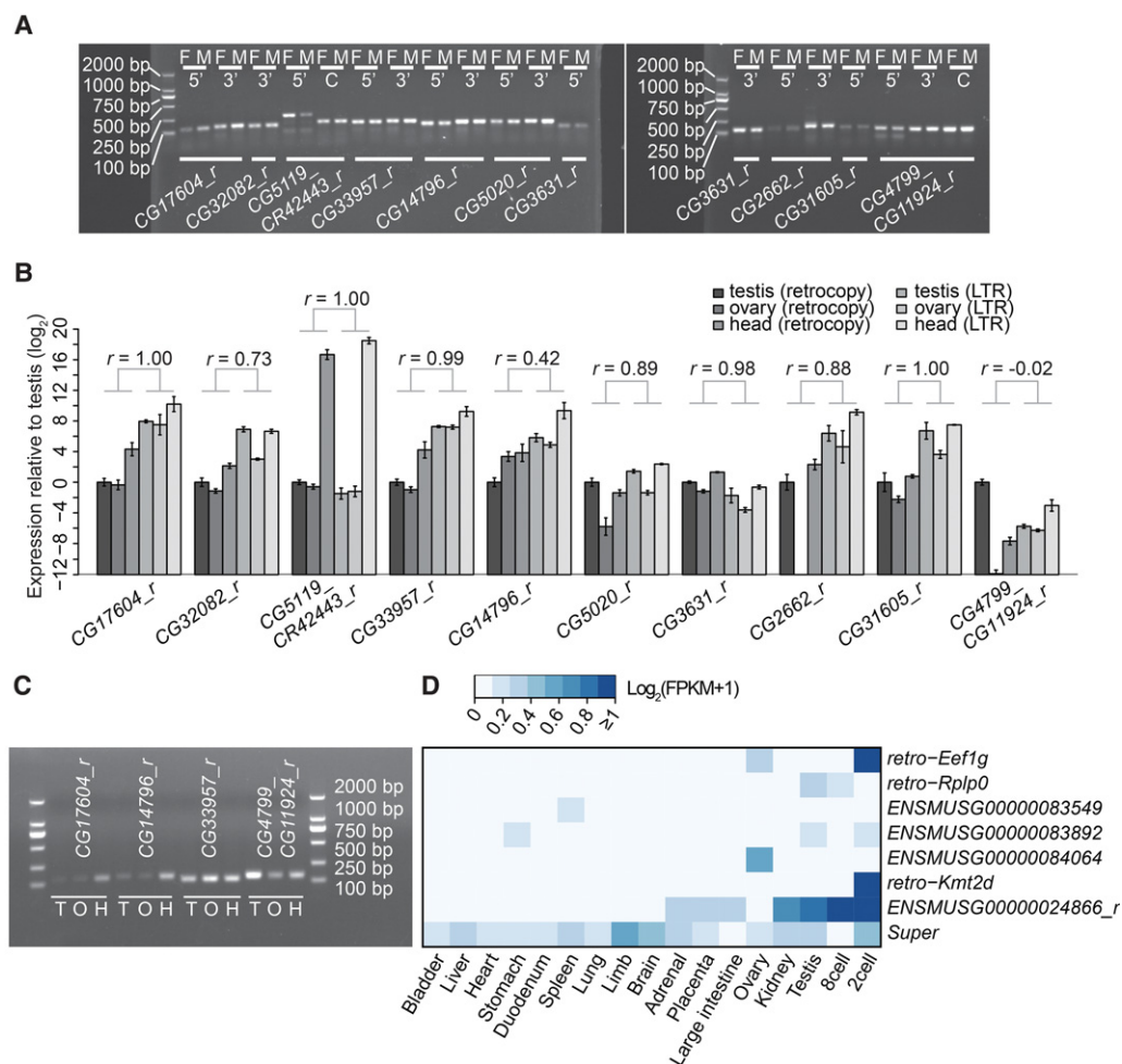
Figure 2. The expression of retrocopies in fruit fly and mouse. (A) Whole-body RT-PCR results for 10 retrocopies validated in Supplemental Figure 2, which are expressed in both male (M) and female (F). The primer sequences and expected product sizes are listed in Supplemental Table 9. For the chimeric genes, CG5119_CR42443_r and CG4799_CG11924_r, we also designed primers flanking the fusion point between the two parental genes, the product of which is marked with "C." (B) Tissue profiling via qRT-PCR. CG2662_r has no detectable expression in ovary. The Pearson correlation ( r ) between the retrocopies and corresponding retrotransposons across the three tissues is displayed above. (C) Tissue level RT-PCR results for four of 10 retrocopies encoded by line 208 across Testis (T), Ovary (O), and Head (H). (D) Expression profile of retrocopies encoded by the mouse genome. Tissues are hierarchically clustered on the basis of expression similarity across genes. Retrocopies are not clustered but instead are sorted by age as approximated by nucleotide divergence. To reveal relative moderate expression, the color-code scheme is truncated at the FPKM cutoff of 1 (i.e., all expression higher than 1 is shown in dark blue).
