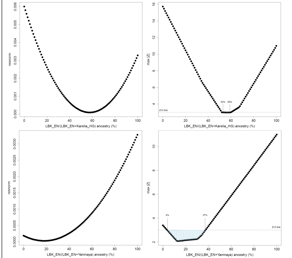
Figure S9.11: U-shaped curve of resnorm and \max|Z| for Corded_Ware_LN as a variable 2-way mixture of LBK_EN and Karelia_HG or Yamnaya.
