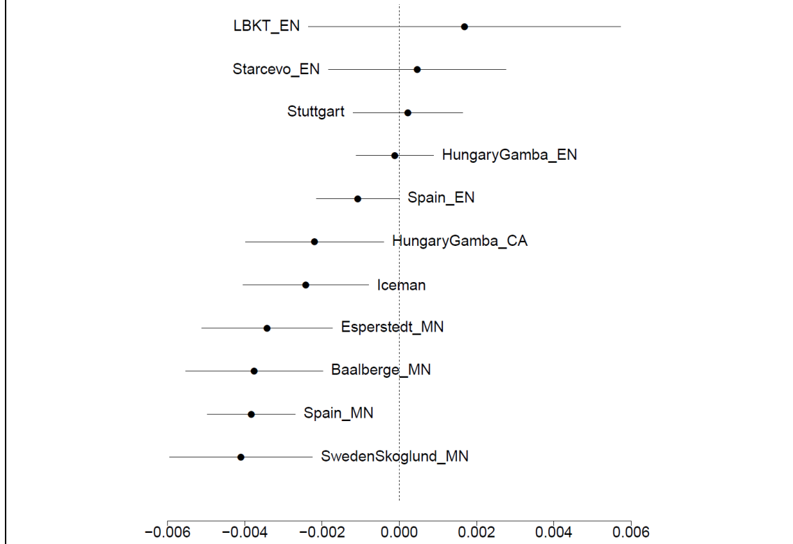
Figure S7.8: Western European hunter-gatherers like Loschbour shared more alleles with Middle Neolithic European farmers, documenting variable amounts of hunter-gatherer ancestry in Neolithic Europe. The estimated value of the statistic f_4(\text{LBK\_EN}, \text{European Farmer}; \text{Loschbour}, \text{Chimp}) and \pm 3 standard errors are shown.
