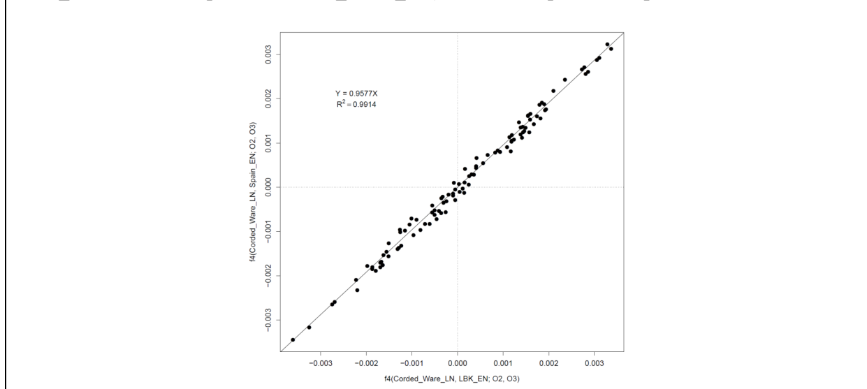
Figure S9.13: When the two references are a clade with respect to the Test (as Spain_EN and LBK_EN are with respect to Corded_Ware_LN), a line with positive slope is observed.
