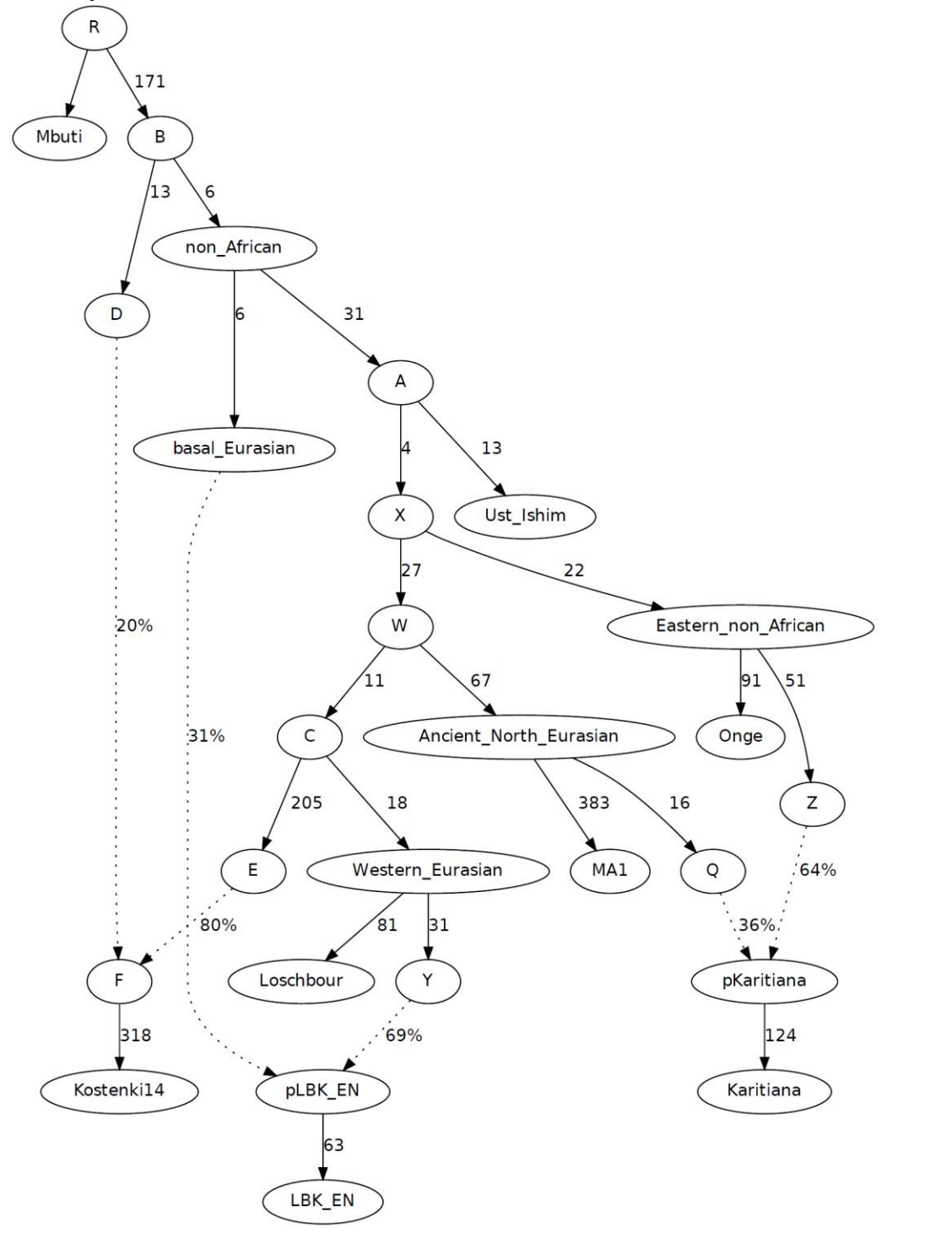
Figure S8.3 Kostenki14 as a 2-way mixture with basal Eurasian admixture before that of the early farmers
