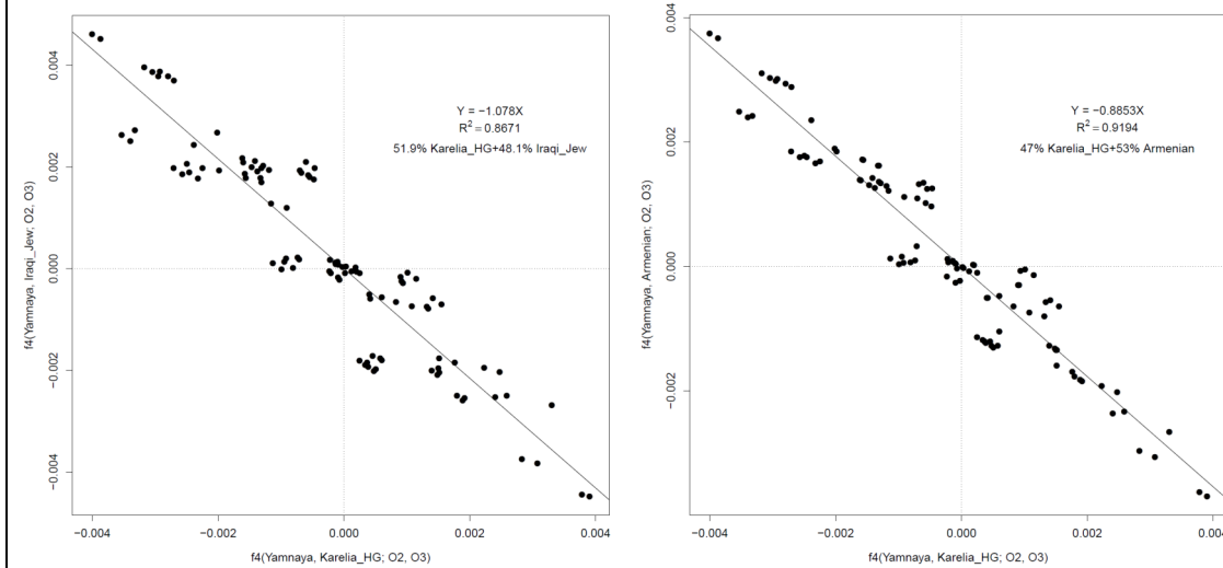
Figure S9.20: The Yamnaya show a pattern of negative correlation when using Karelia_HG and either Iraqi_Jew or Armenian as references. This is consistent with it having a component of ancestry related to the Caucasus/Near East, suggesting that ancient DNA work in these regions may reveal a good surrogate for this type of ancestry.
