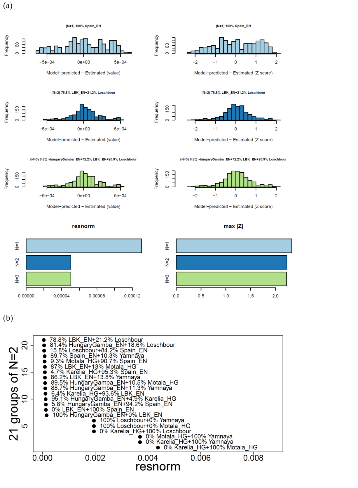
Figure S9.6: Modeling Spain_MN as a mixture of earlier populations. (a) We present in the left column a histogram of raw f_4 -statistic residuals and on the right Z-scores for the best-fitting (lowest resnorm ) model at each N . In the bottom row, we show on the left how resnorm and the maximum |Z| score change for different N . (b) resnorm of different N=2 models.
