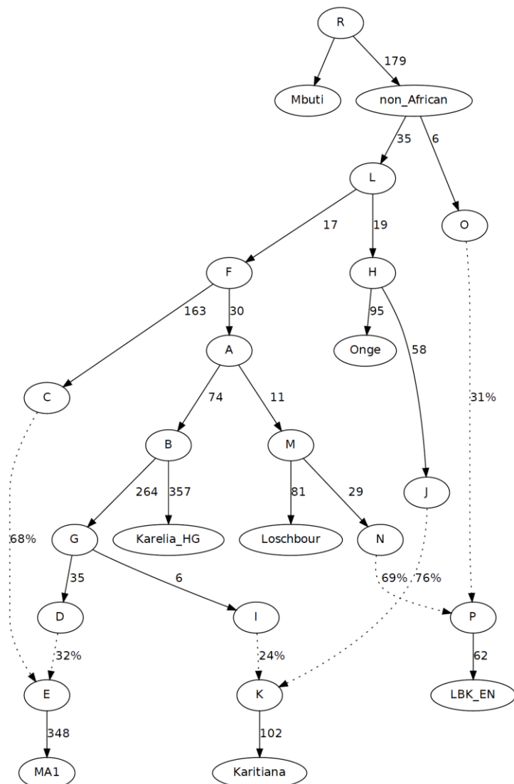
Figure S8.10: Adding LBK_EN to the Fig. S8.9a model (MA1 admixed; this weakly fails |Z|=3.2 )
