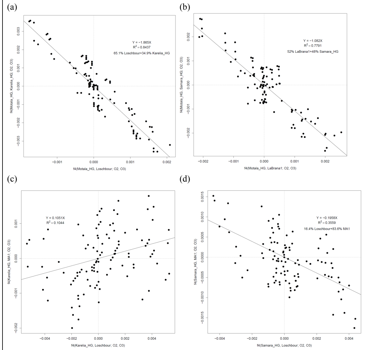
Figure S9.14: Motala_HG is a mixture of (a) Loschbour and Karelia_HG or (b) LaBran1 and Samara_HG. By plotting these statistics we recover a signal of admixture that is not shown by the f_3(\text{Motala\_HG}; \text{Loschbour}, \text{Karelia\_HG}) statistic due to post admixture genetic drift in Motala_HG ancestors. However, Karelia_HG (c) and Samara_HG (d) do not appear to be a mixture of Loschbour and MA1. The lack of a negative correlation does not disprove the presence of such admixture, but it provides an additional motivation for considering the alternative models in SI8.
