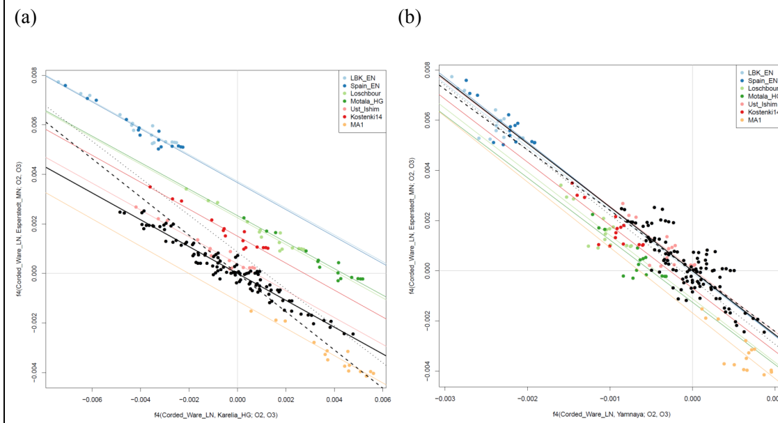
Figure S9.21: Adding different outgroups in position O_3 of the statistics f_4(\text{Corded\_Ware, Eastern}; O_2, O_3) vs. f_4(\text{Corded\_Ware, Esperstedt\_MN}; O_2, O_3) . (a) Eastern=Karelia_HG, (b) Eastern=Yamnaya
