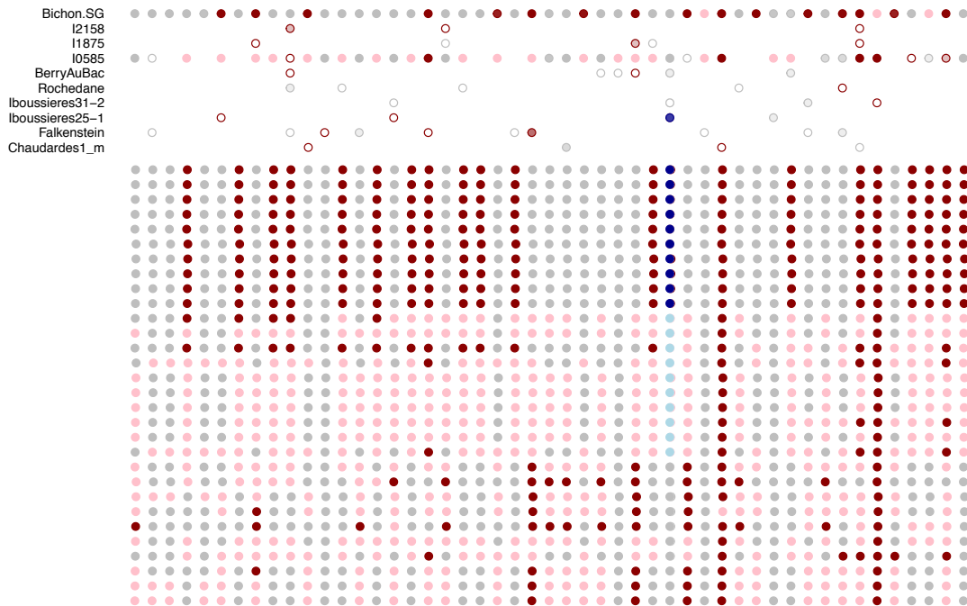
Figure S2.4: Haplotypes at the LCT locus for WHG individuals (top, labeled), and 30 present-day individuals from the GBR and TSI populations, with 10 of each genotype at the focal SNP rs4988235 (in blue). Each column is a SNP, each row is an individual. A grey point indicates homozygous for the ancestral allele, light colored heterozygous, and dark colored homozygous for the derived allele. Ancient individuals are shaded according to how many reads there are at that site, so an open circle means there is only one read, and darker colors indicate more reads, and therefore more certainty about homozygous genotypes.
