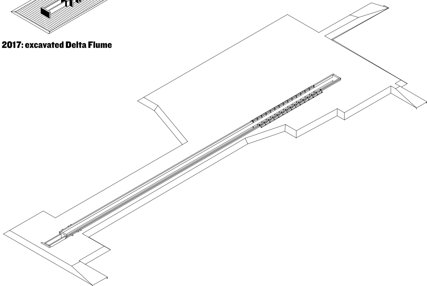
1970-2016: existing Delta Flume
