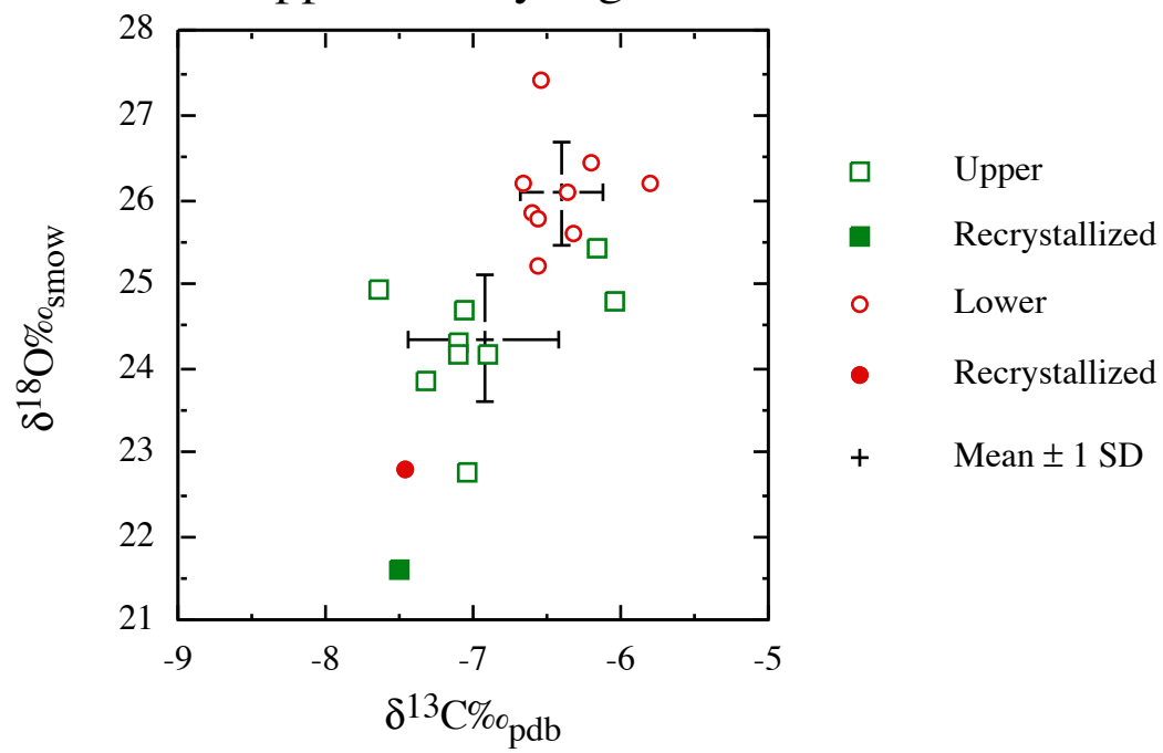
Supplementary Figure 1. ASI Paleosol Carbonates
