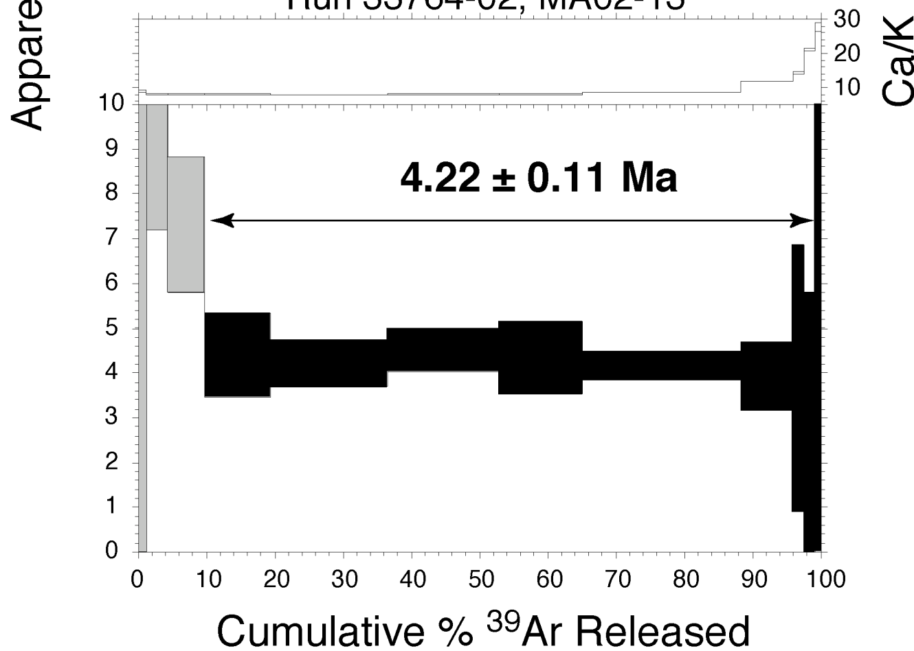
Supplementary Figure 3. Argon-Argon results.
