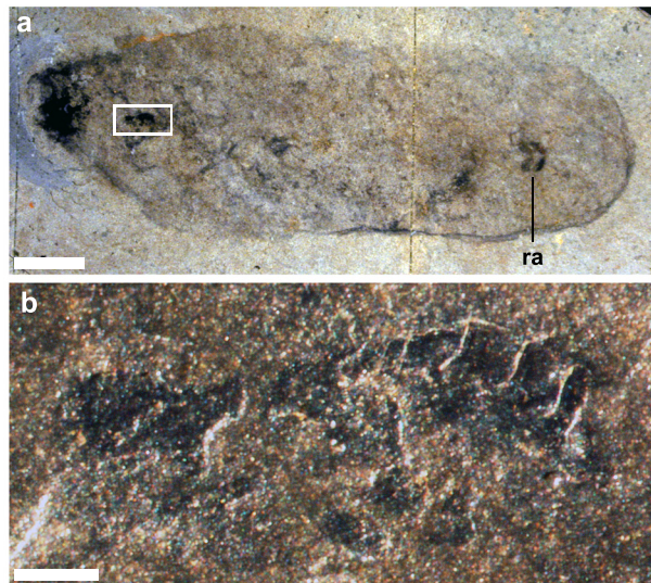
Supplementary Figure III. Odontogriffus omalus from the Middle Cambrian Burgess Shale, ROM57718. Specimen preserved dorso-ventrally. a , overall view, anterior to the right - the presence of a row of teeth inside the gut is emphasized by the white frame; b close-up view of the framed area from a . Scale bars: 5mm in a ; 0.5mm in b . ra=radula
