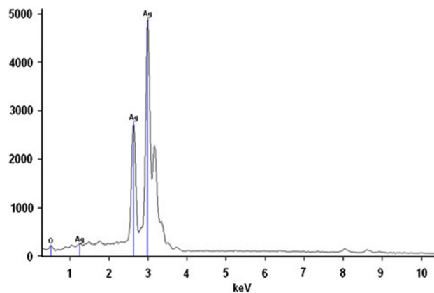
Fig. 6 EDAX pattern of silver nanoparticle
