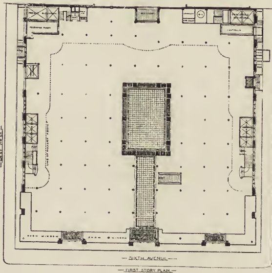
FIRST FLOOR PLAN OF STORE OF ADAMS & CO. Sixth Ave., 21st to 22d Sts., New York City. De Lemos & Cordes, Architects.
