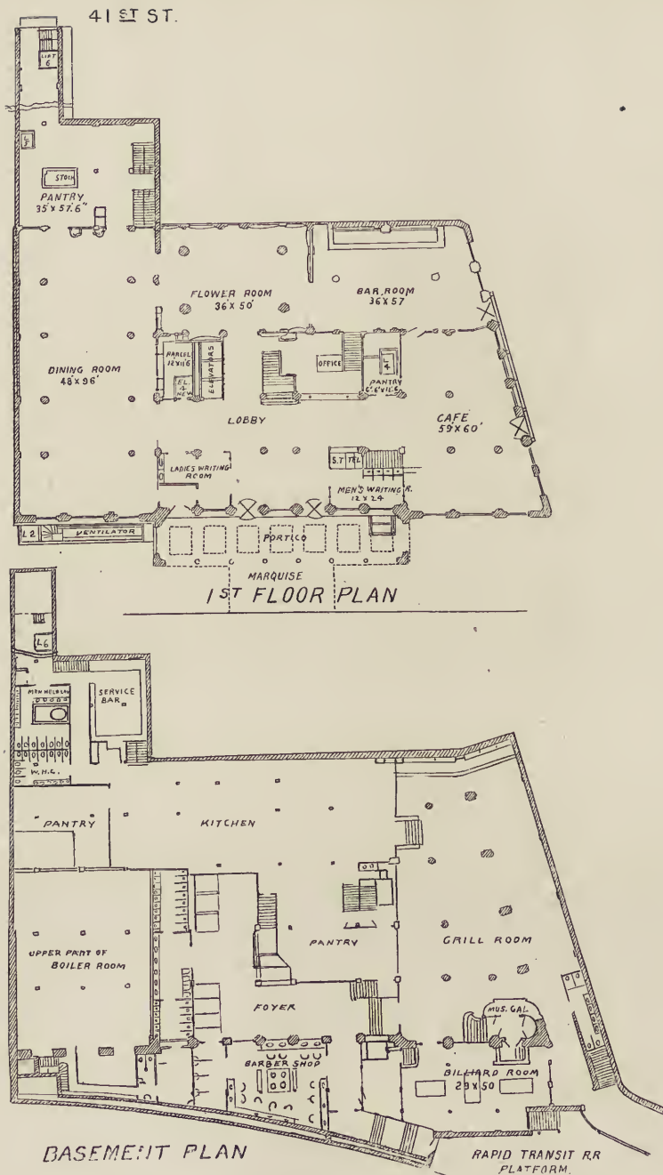
BASEMENT AND FIRST FLOOR PLAN OF HOTEL KNICKERBOCKER. New York City. Warren & Davis & Bruce Price, Architects.
