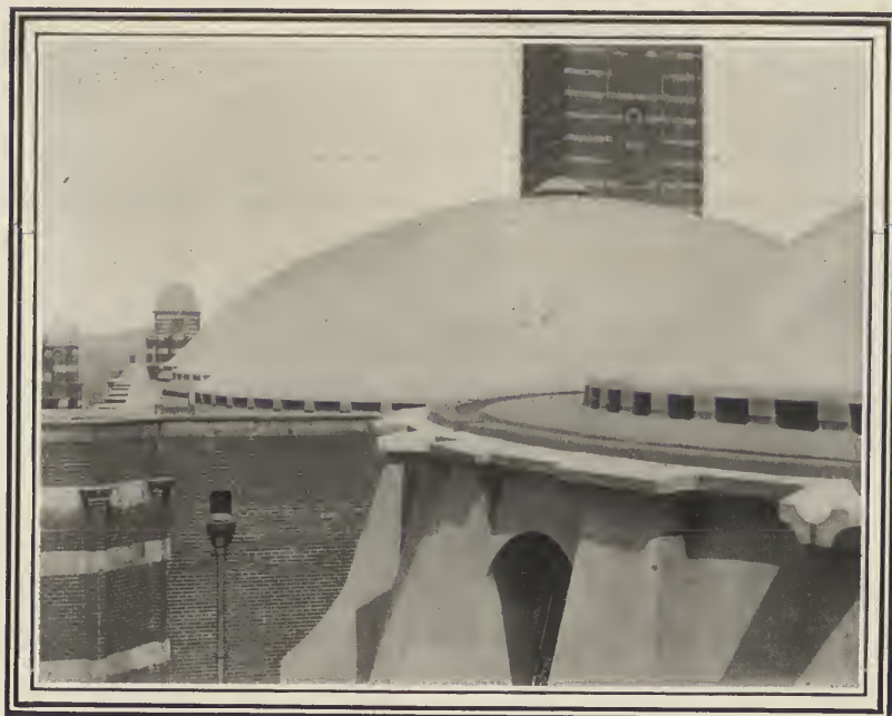
THE DOMES OF THE SANCTUARY AND OF THE NAVE, SHOWING THE EX- TERNAL COVERING OF CEMENT SLABS, ENCLOSING AN AIR SPACE.
