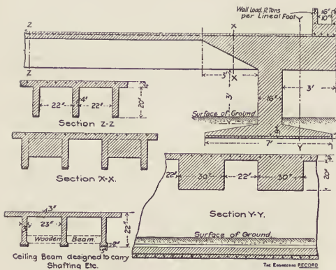
FIG. 33.—CANTILEVER SUPPORT FOR FACTORY WALL ON SOFT GROUND.
