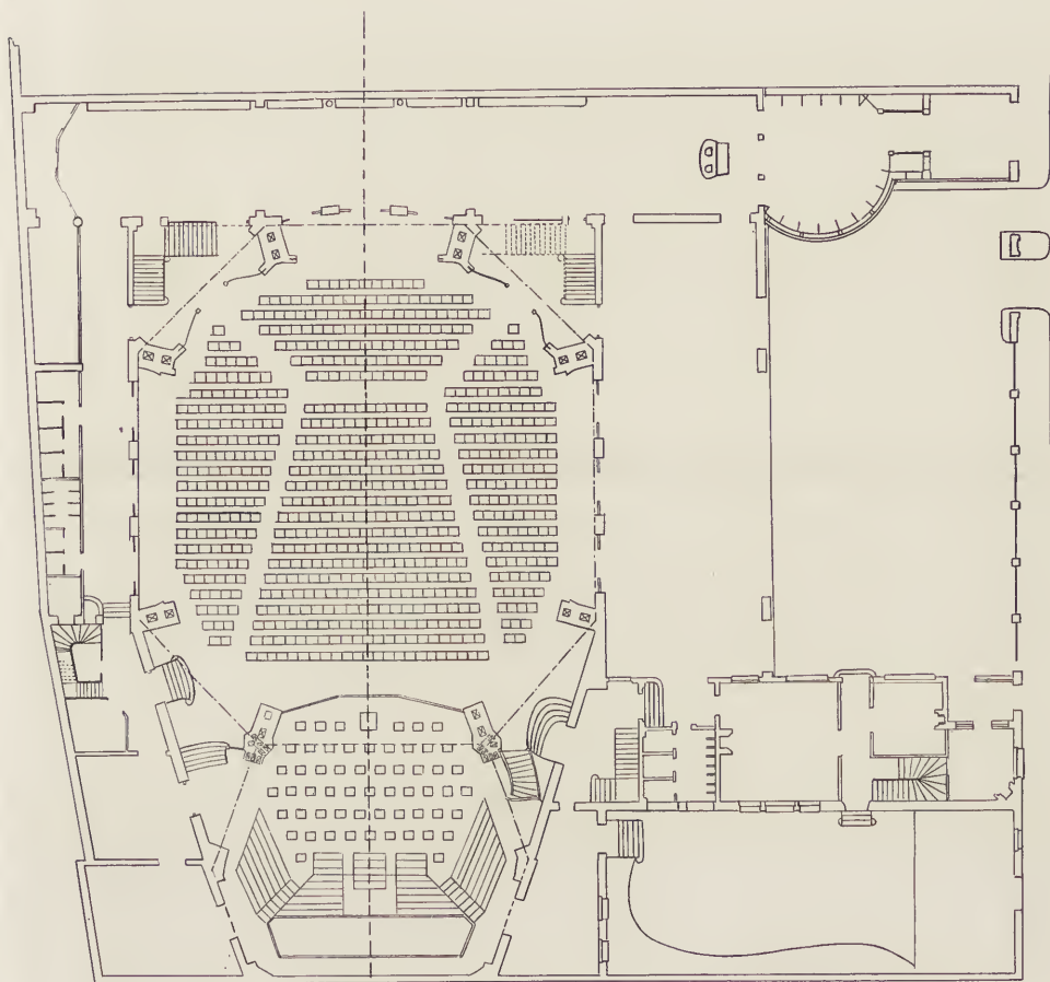
PLAN OF THE HALL.
