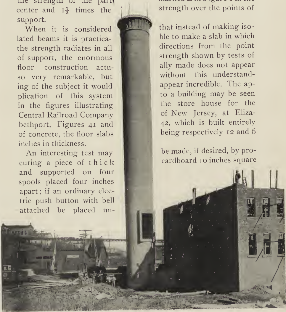
FIG. 10.—CHIMNEY CONSTRUCTED OF REINFORCED CONCRETE. No outside scaffolding was used.
