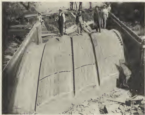
FIG. 9.—CENTERING FOR A BRIDGE. Situating on Evergreen Road, near Pitts- burgh, Pa.
