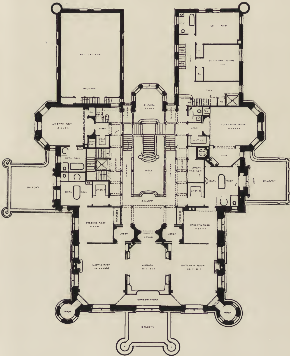
PLAN OF THE SECOND STORY OF THE SCHWAB MANSION.
