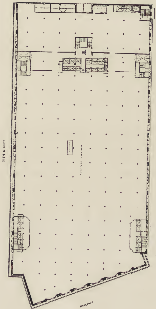
PLAN OF 4TH STORY
