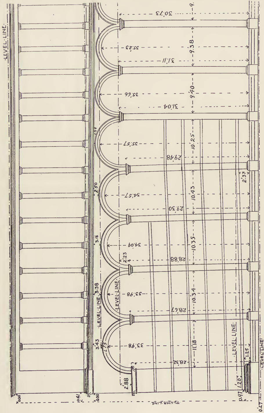
FIG. 6. SURVEY OF THE SOUTH CATHEDRAL WALL AT PISA, NEAR THE FACADE.
