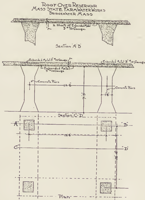
FIG. 17.—SECTION OF RESERVOIR ROOF.
