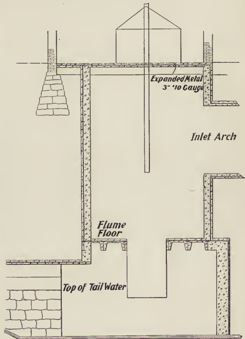
FIG. 20.—GENERAL VIEW OF THE WHEEL PIT.
