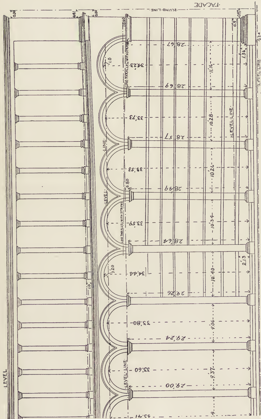
FIG. 5. SURVEY OF THE NORTH CATHEDRAL WALL AT PISA, NEAR THE FACADE.
