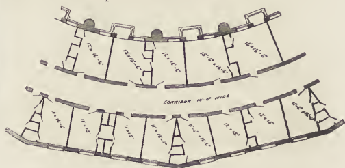
FIG. 25.—FLOOR PLAN OF HOTEL AT WEST BADEN SPRINGS, IND.
