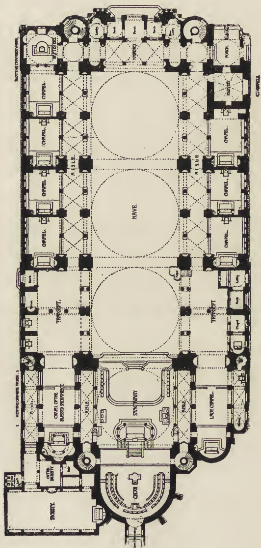
GROUND PLAN OF THE NEW CATHEDRAL AT WESTMINSTER. John Francis Bentley, Architect.
