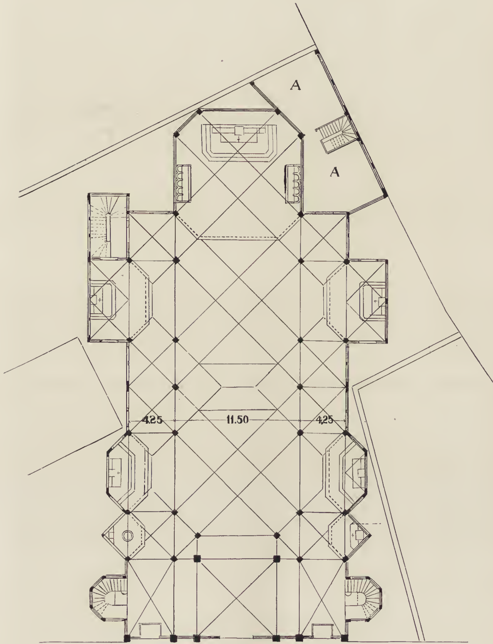
FIG. 1.—PLAN OF THE CHURCH.
