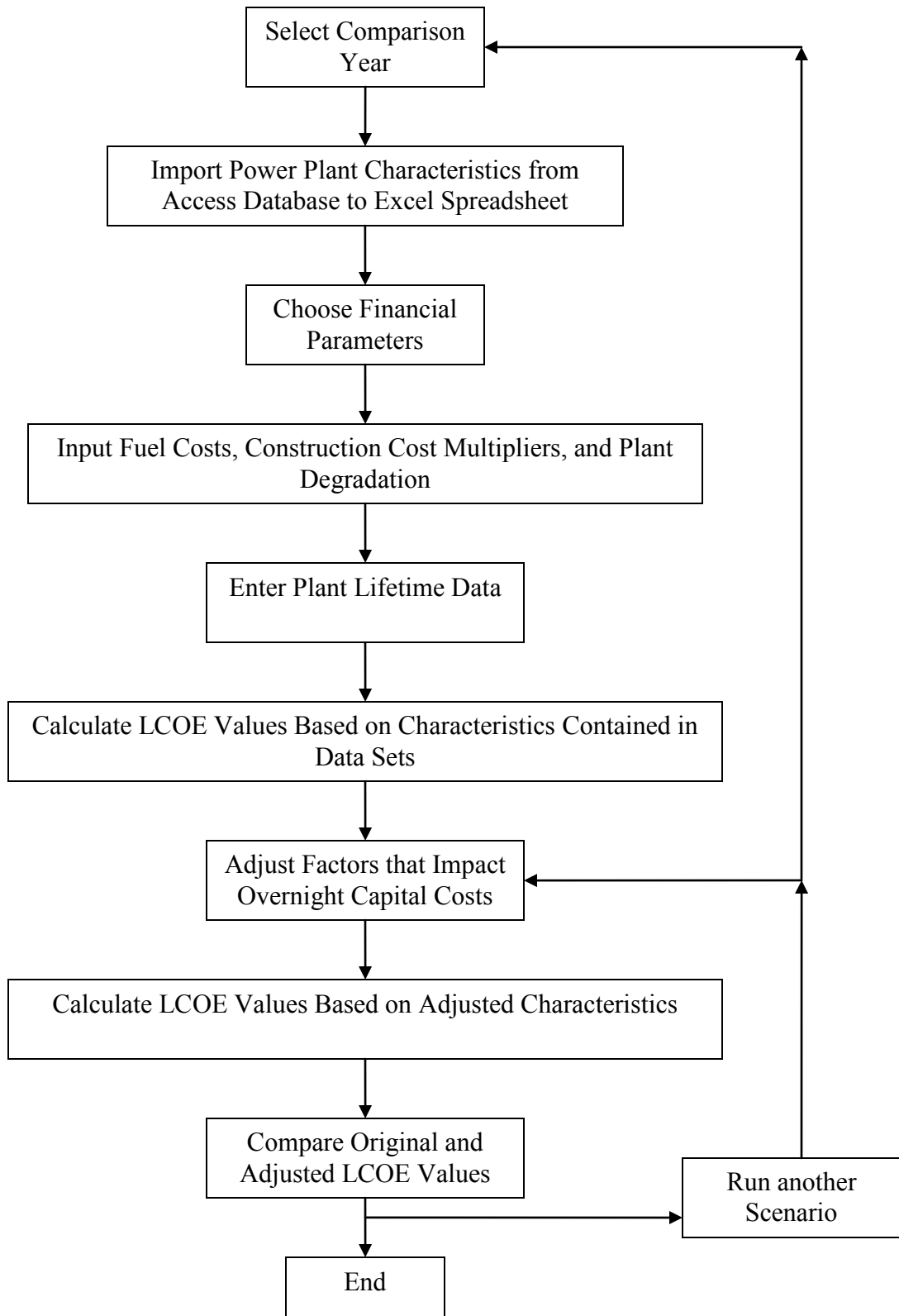
Figure 130. Flow chart for the LCOE tool
