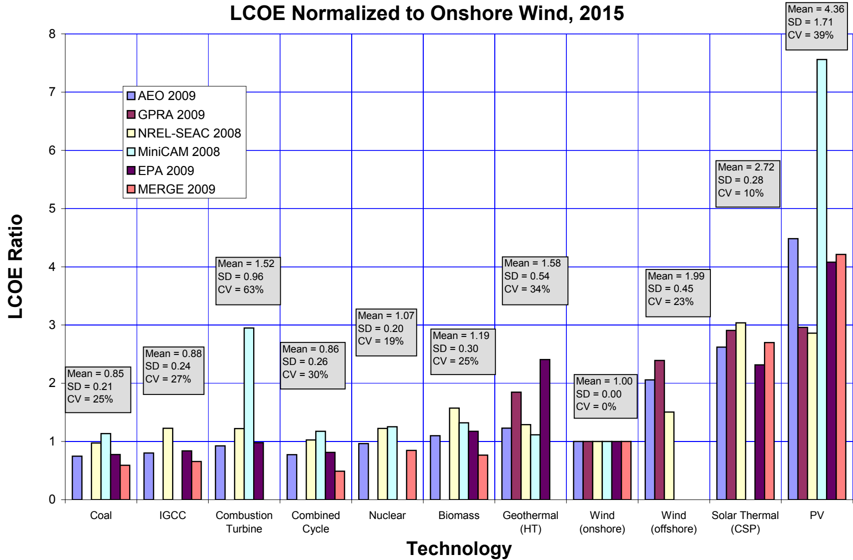
Figure 41. LCOE cost ratios relative to wind, 2015
