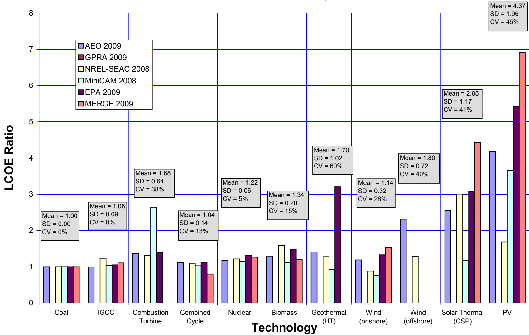
Figure 40. LCOE cost ratios relative to coal, 2030
