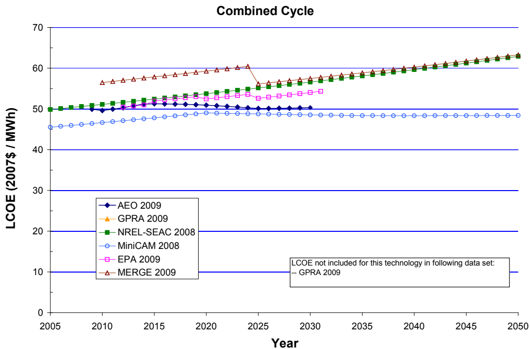
Figure 57. LCOE—combined cycle
