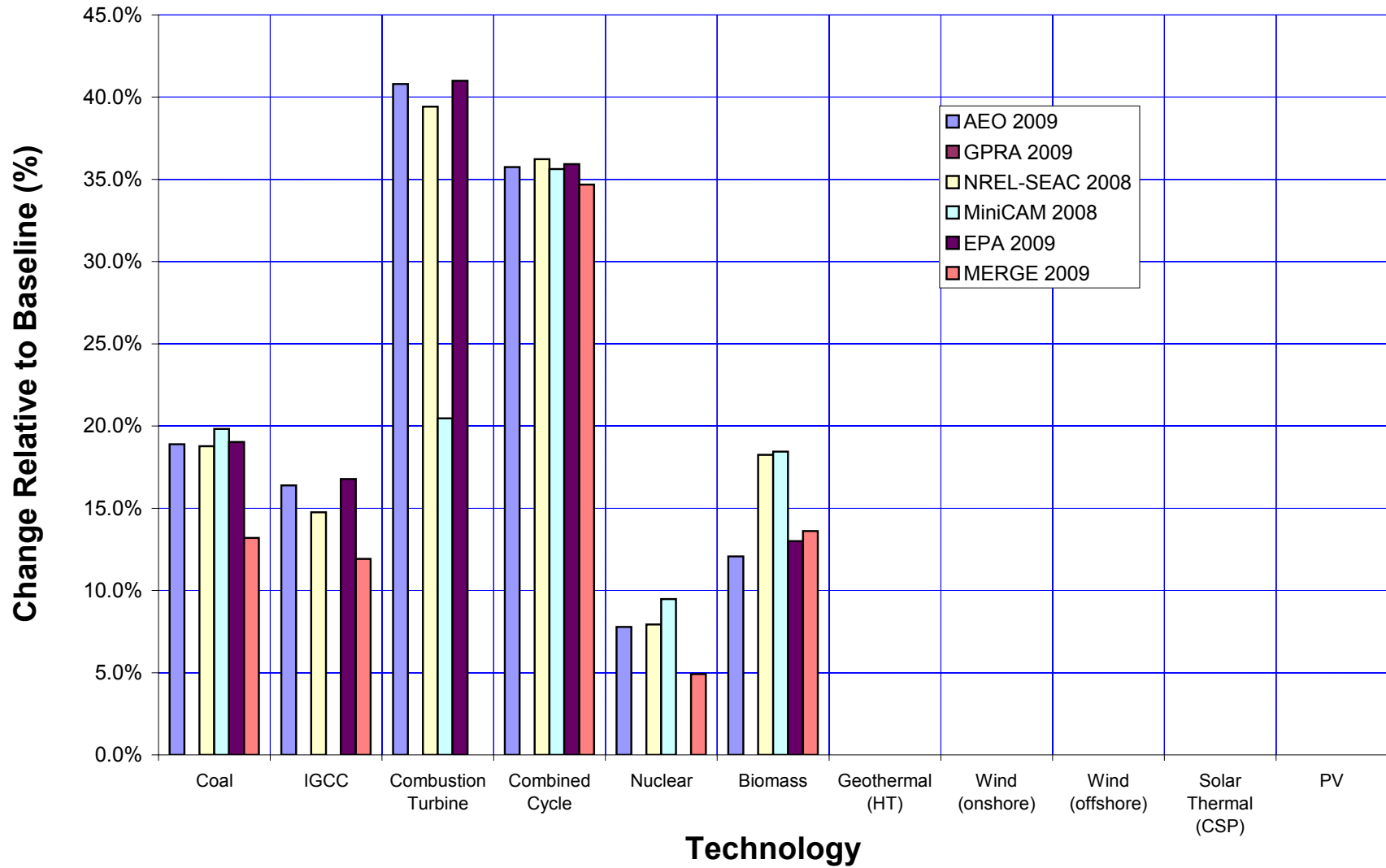
Figure 70. Impact on LCOE of fuel cost, 50% change
