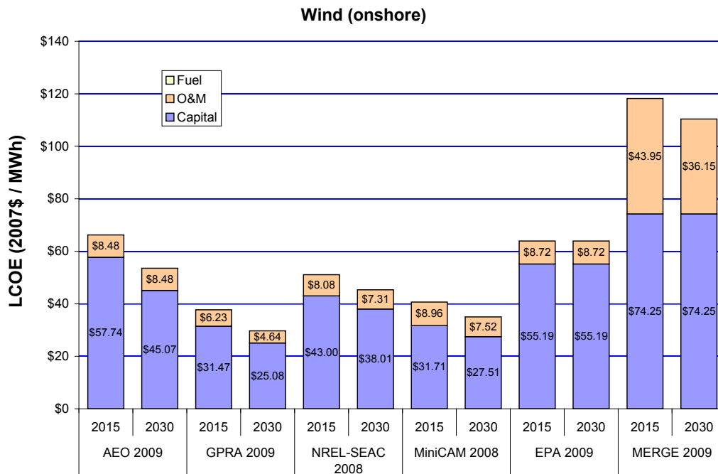
Figure 50. Capital, fuel, and O&M costs—wind (onshore)
