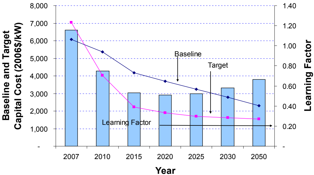
Figure 92. GPR 2009, commercial PV learning factor
