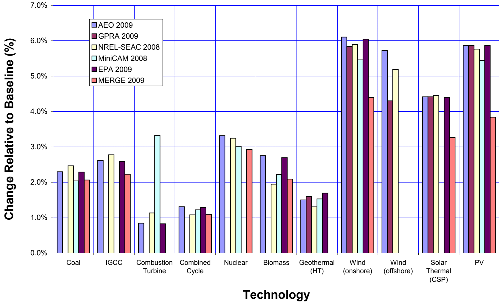
Figure 65. Impact on LCOE of equipment cost, 10% change
