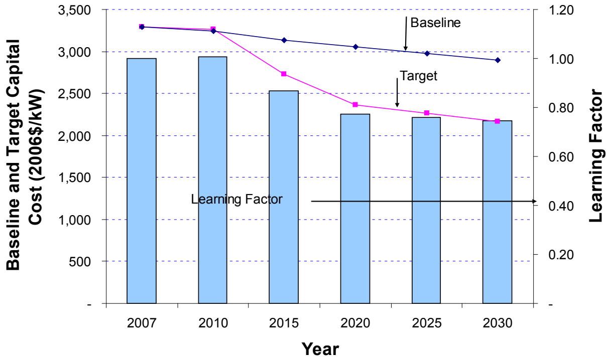
Figure 88. GPR 2009, geothermal flash learning factor
