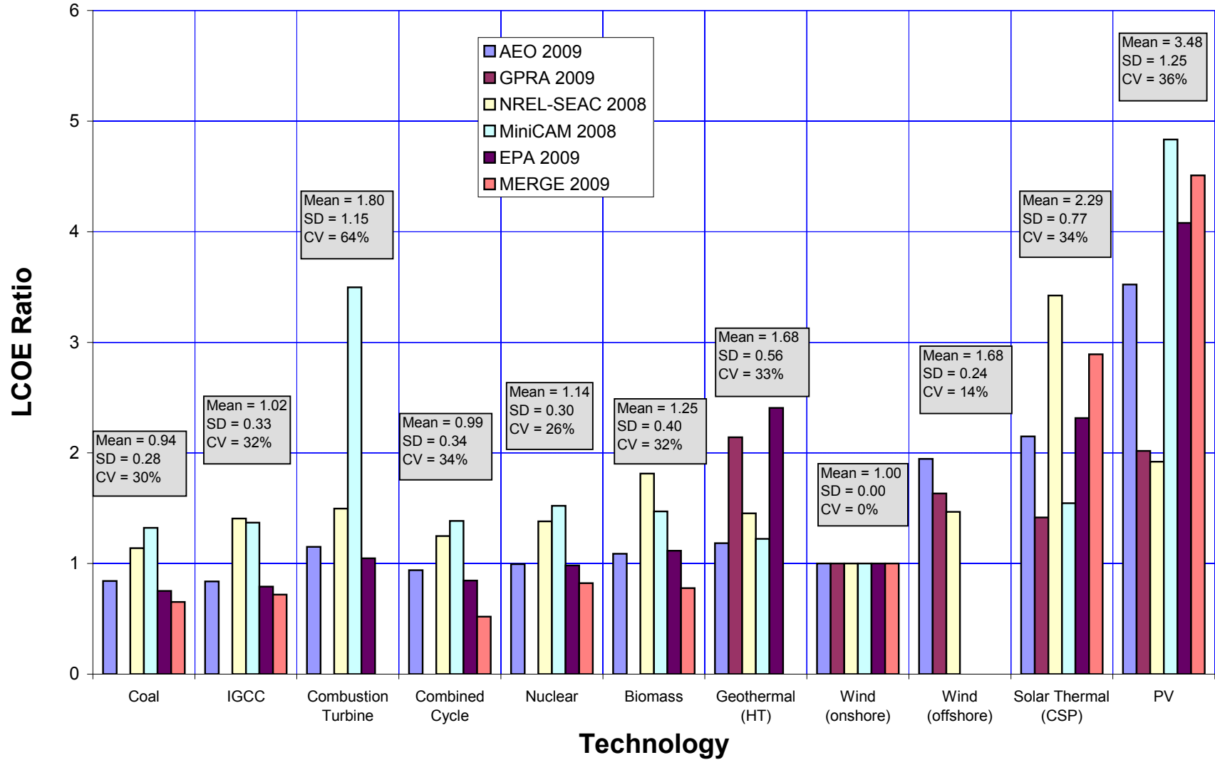
Figure 42. LCOE cost ratios relative to wind, 2030
