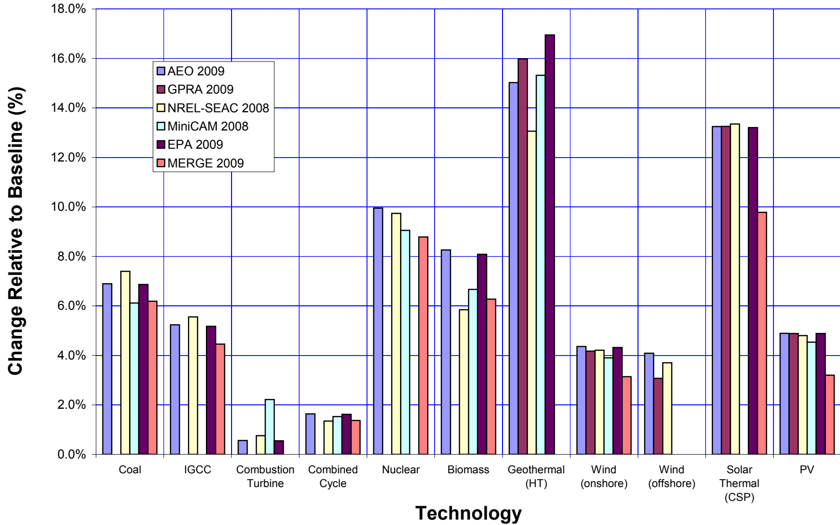
Figure 68. Impact on LCOE of labor cost, 50% change
