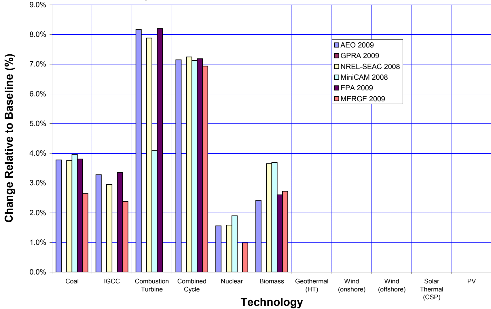
Figure 69. Impact on LCOE of fuel cost, 10% change
