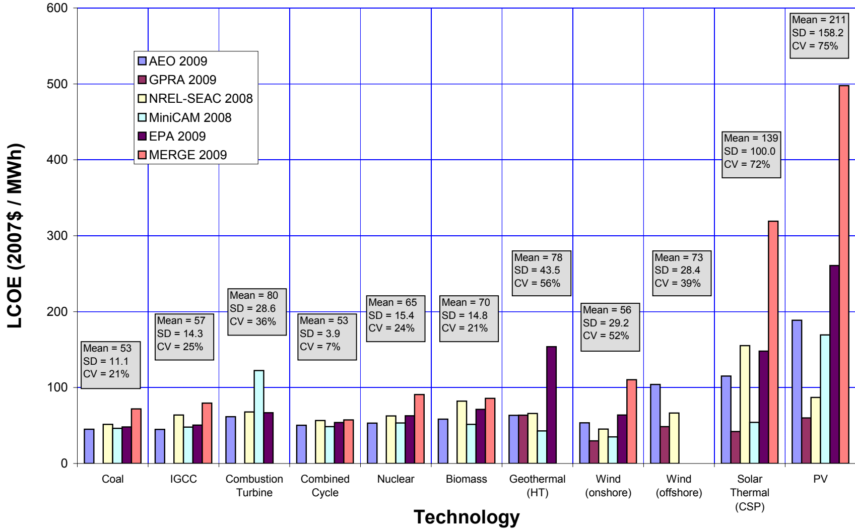
Figure 38. LCOE costs, 2030
