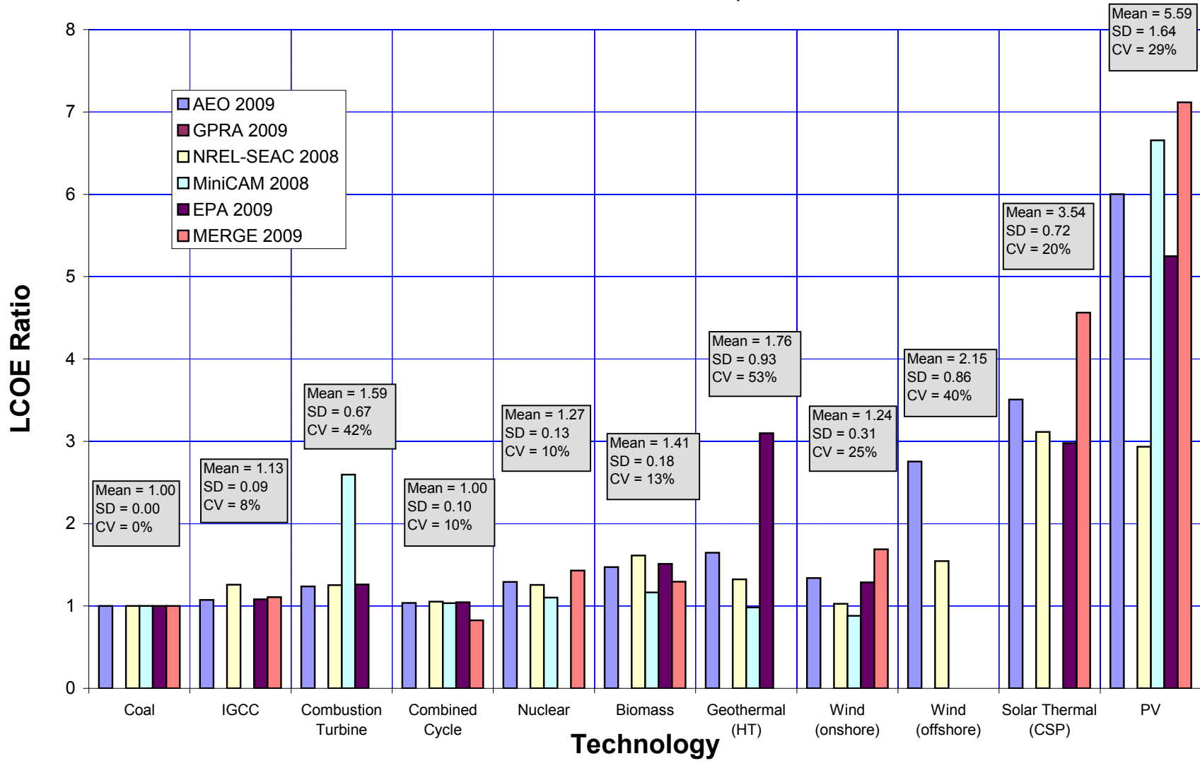
Figure 39. LCOE cost ratios relative to coal, 2015
