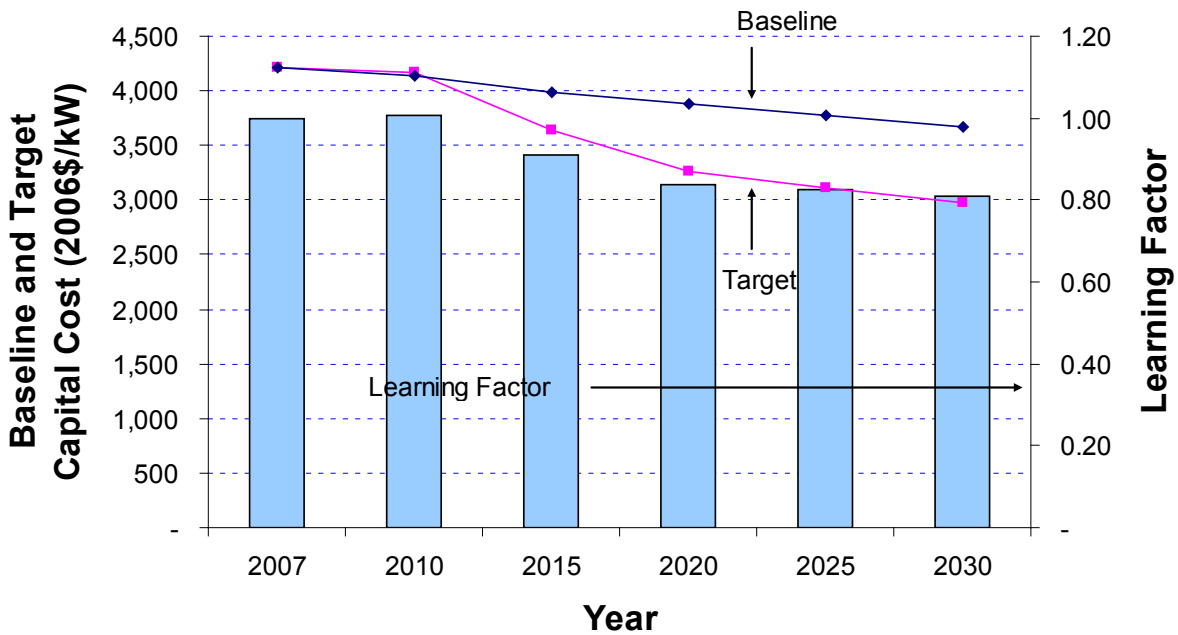
Figure 90. GPR 2009, geothermal EGS—convective learning factor
