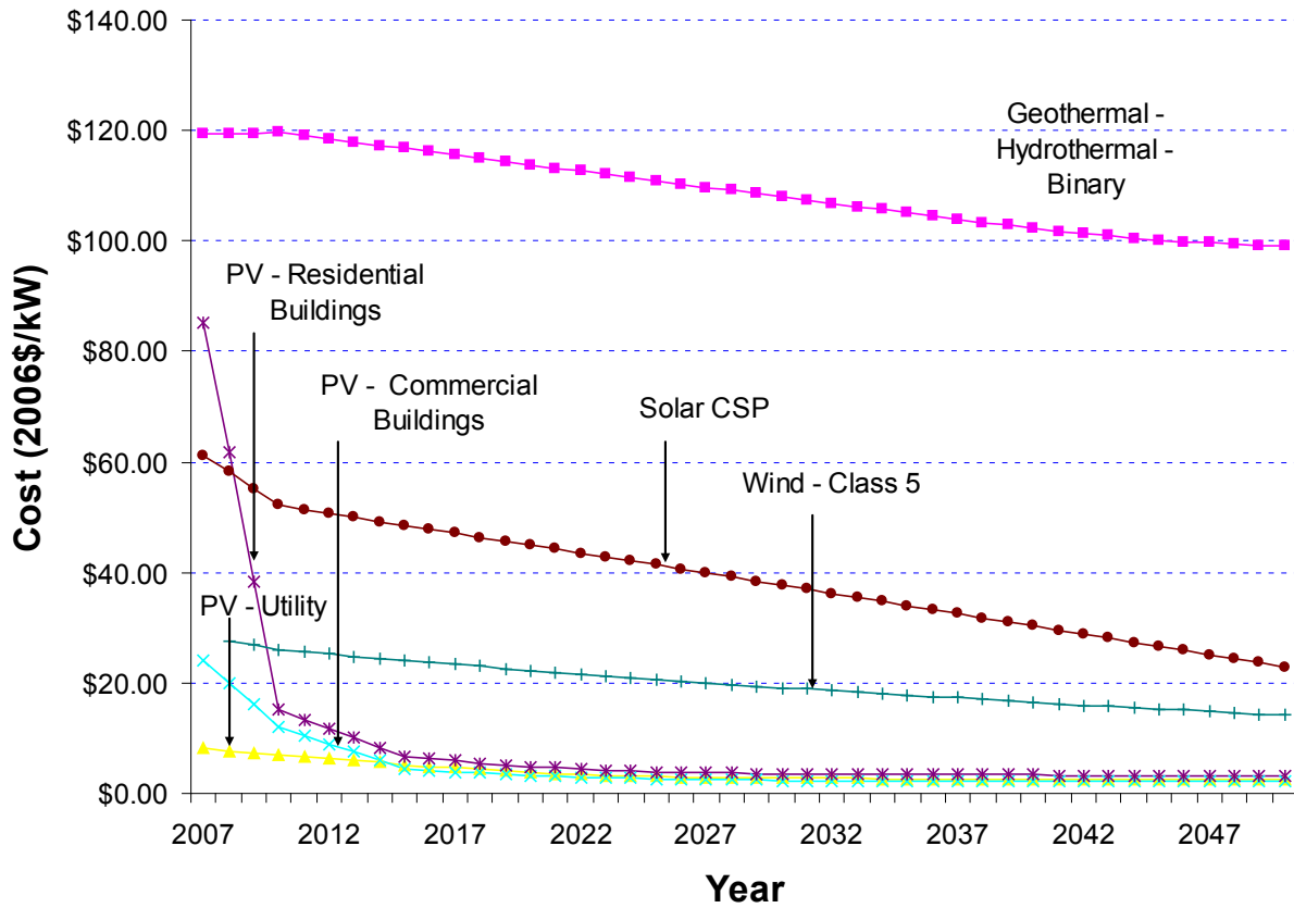
Figure 94. GPR 2009, fixed annual O&M costs for renewable technologies
