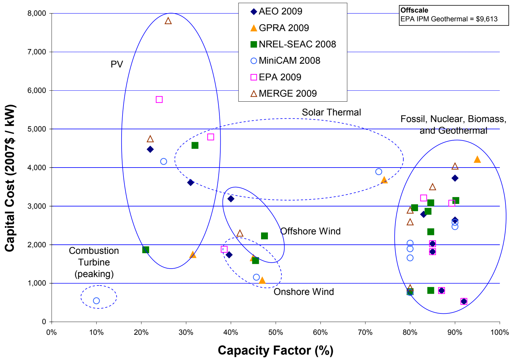
Figure 23. Overnight capital costs versus capacity factors, 2025
