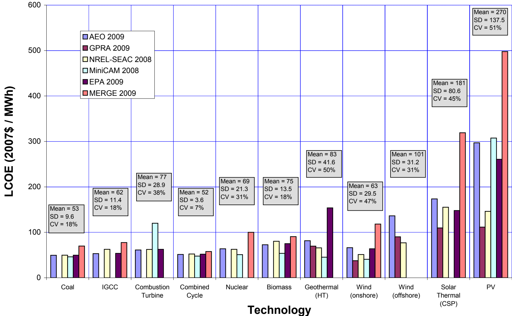
Figure 37. LCOE costs, 2015
