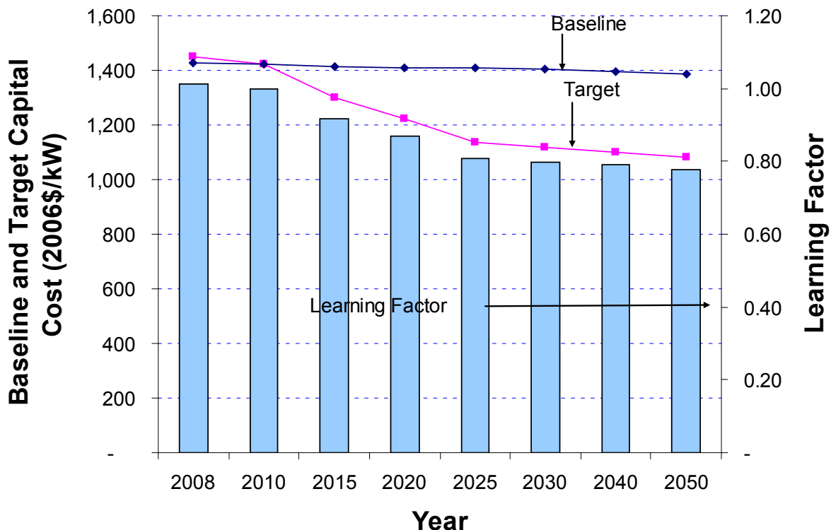
Figure 85. GPR 2009, onshore wind class 4 capital costs (base and target cases)
