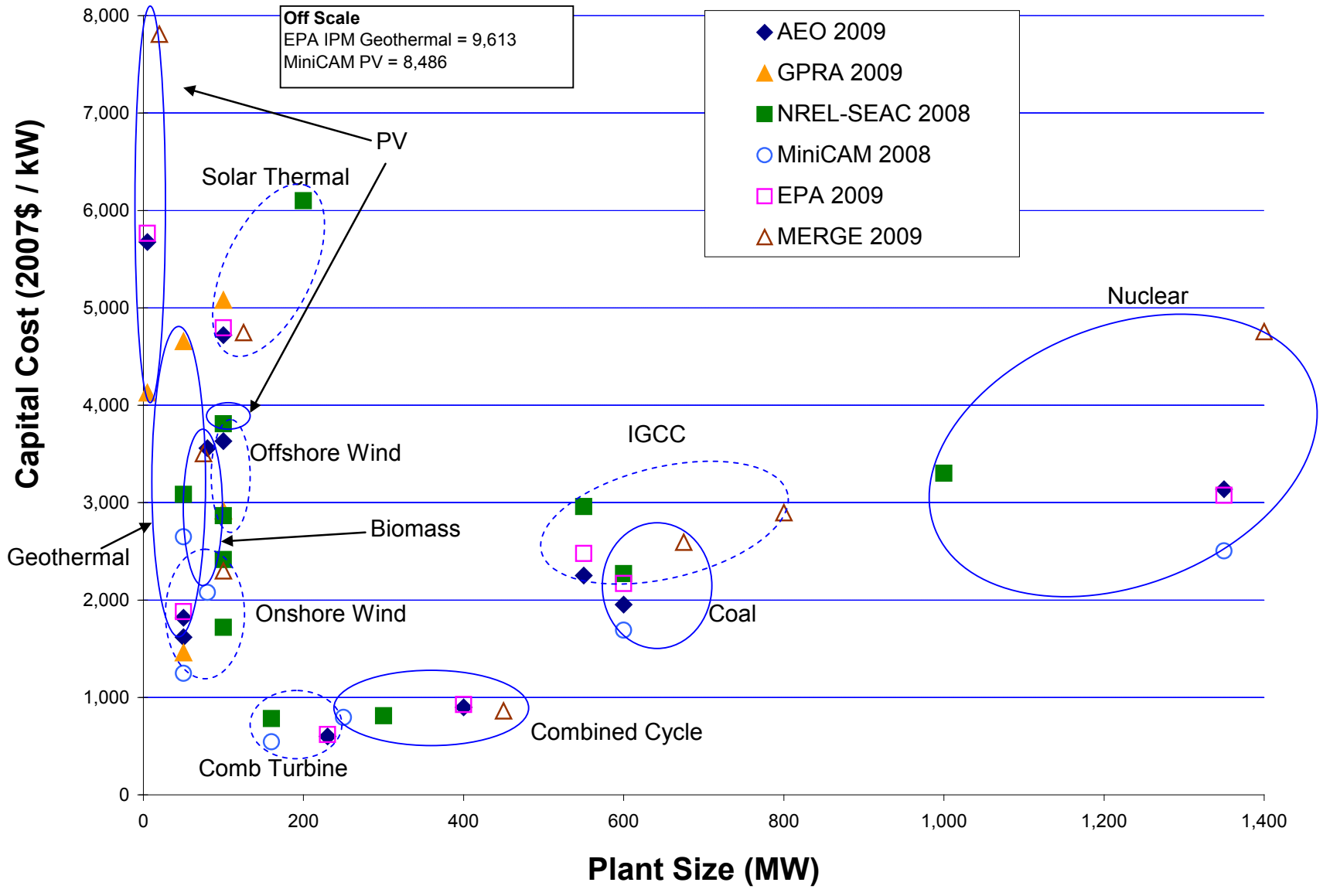
Figure 20. Capital cost versus plant size, 2010
