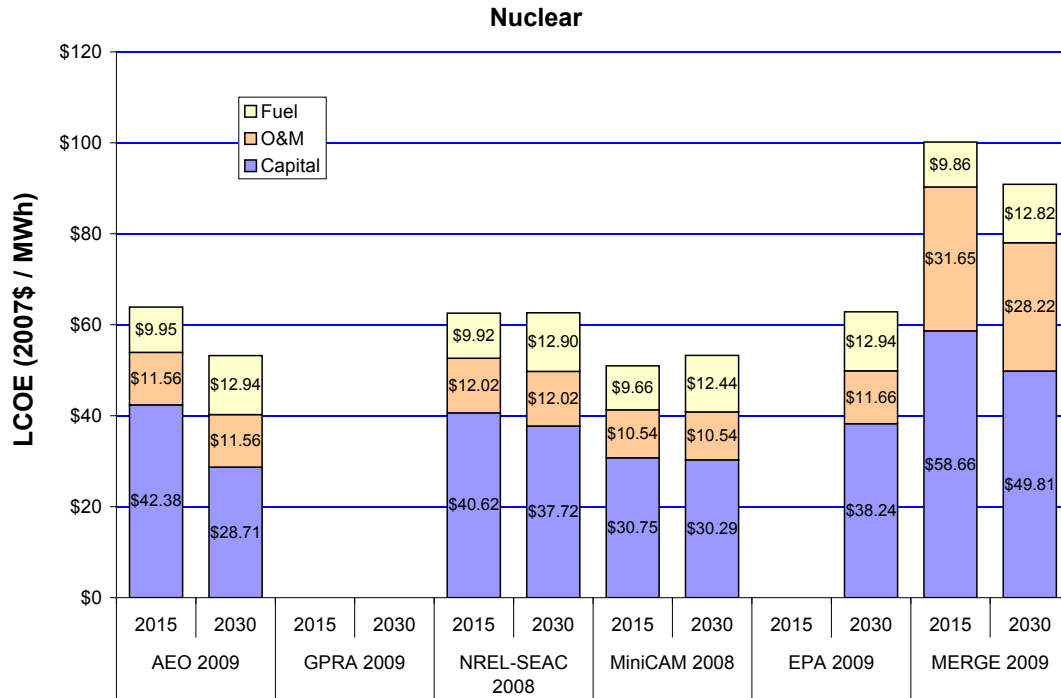
Figure 47. Capital, fuel, and O&M costs—nuclear
