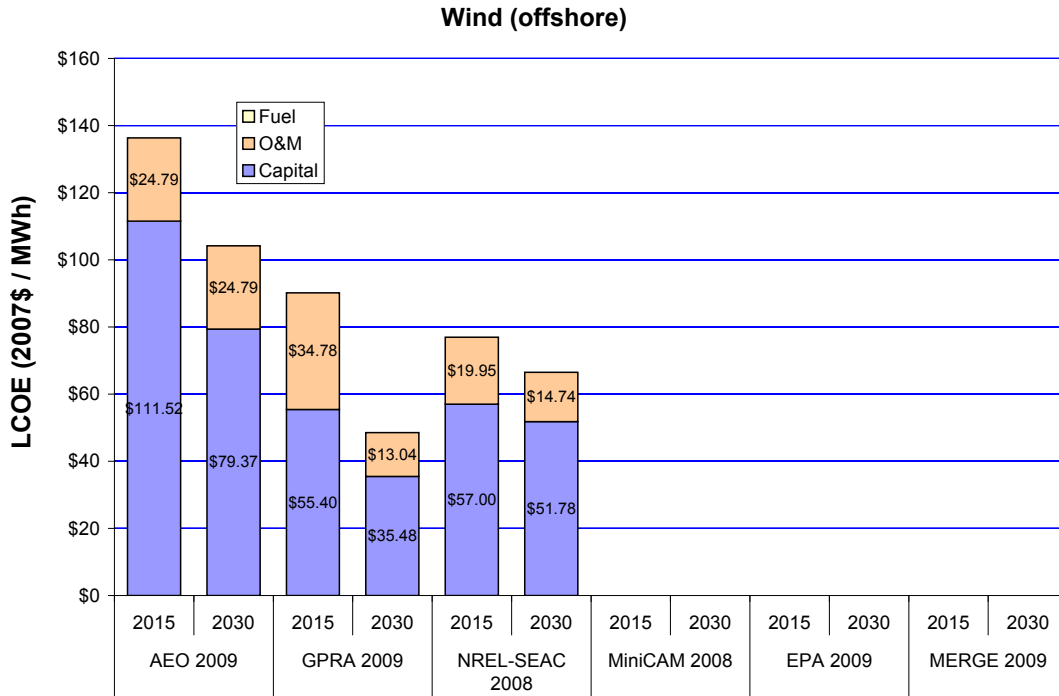
Figure 51. Capital, fuel, and O&M costs—wind (offshore)
