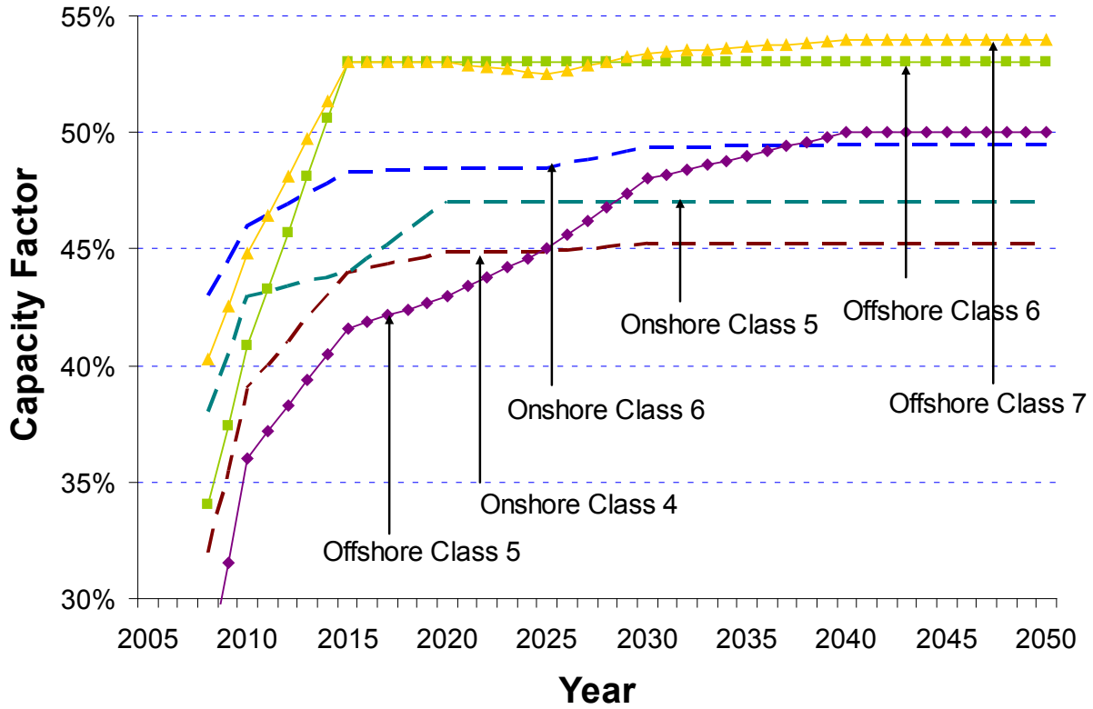
Figure 81. GPR 2009, wind capacity factors
