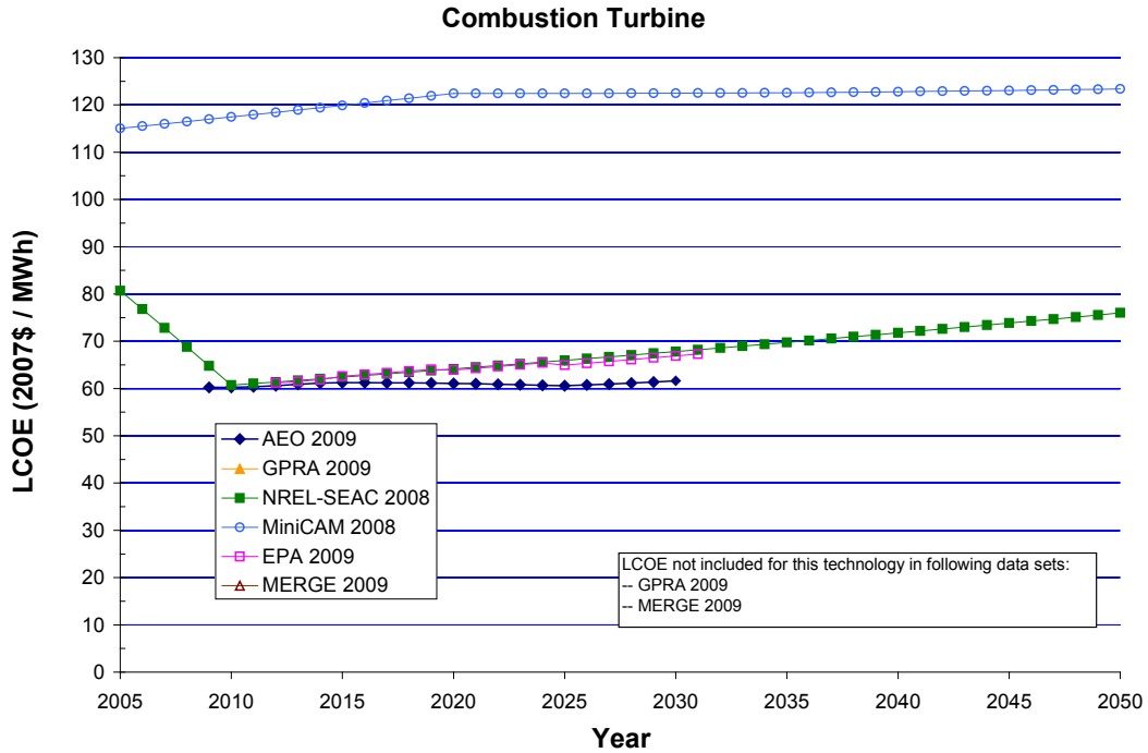
Figure 56. LCOE—combustion turbine
