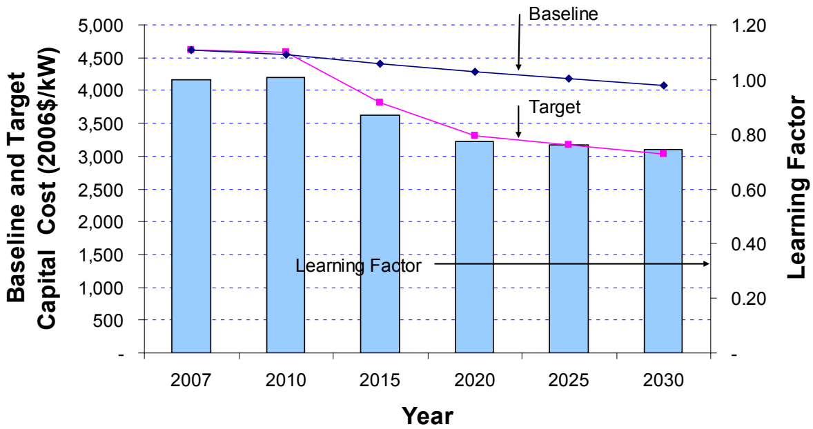
Figure 89. GPR 2009, geothermal binary learning factor
