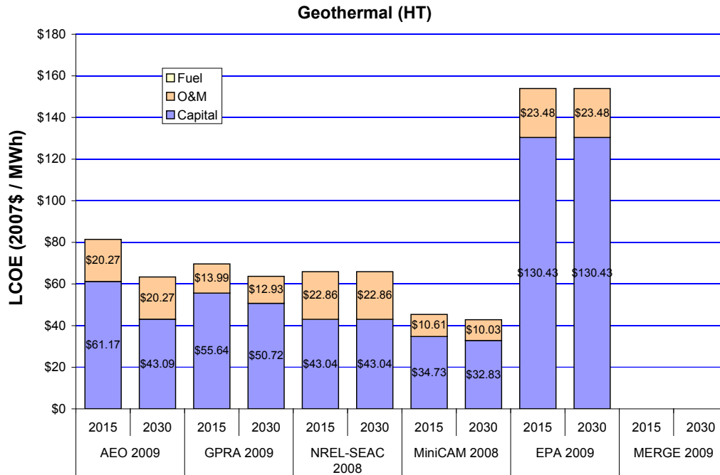
Figure 49. Capital, fuel, and O&M costs—geothermal (HT)
