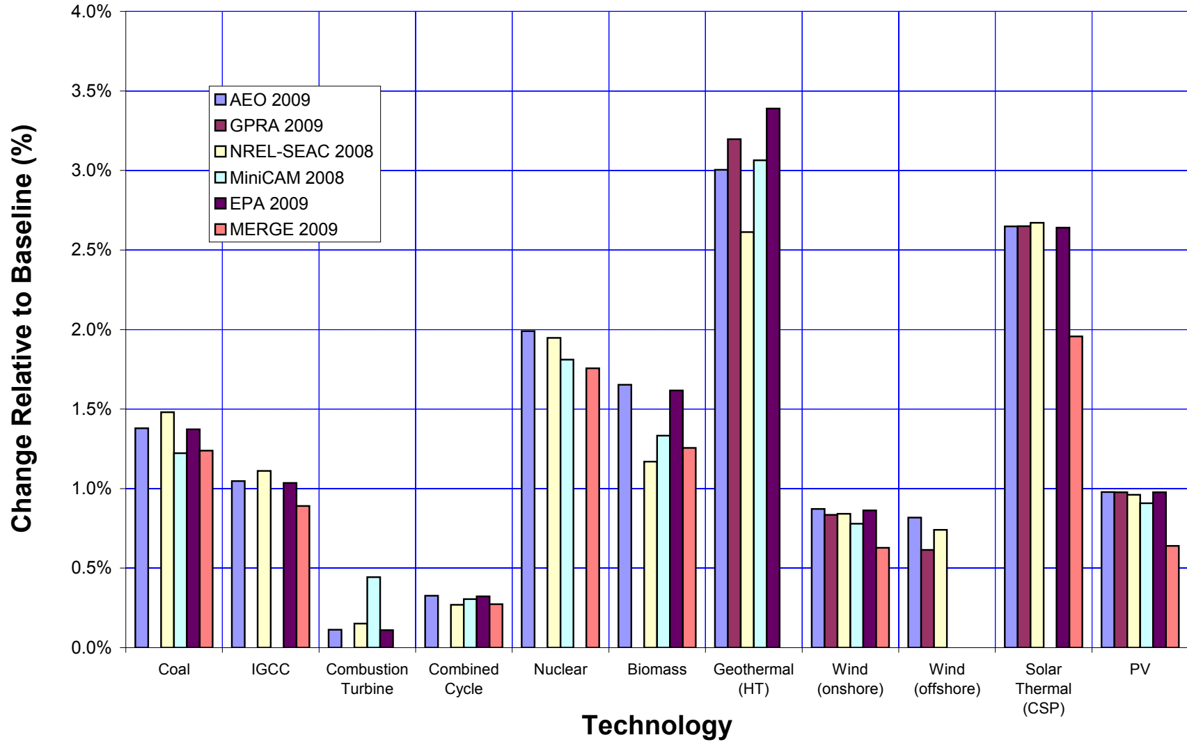
Figure 67. Impact on LCOE of labor cost, 10% change
