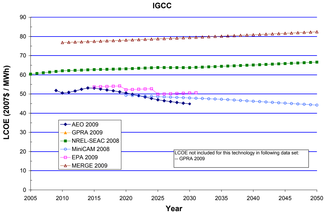
Figure 55. LCOE—IGCC
