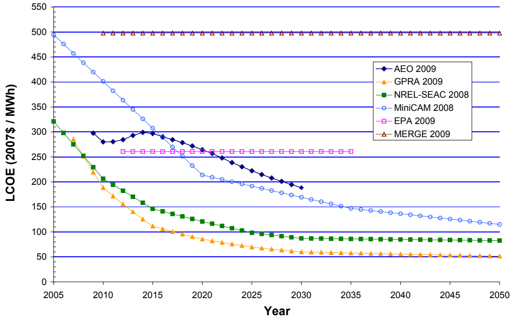
Figure 64. LCOE—PV
