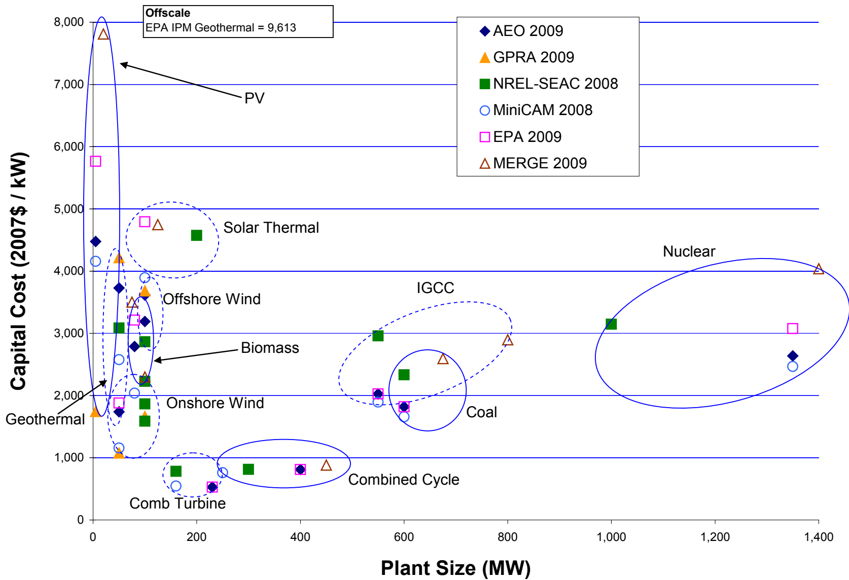
Figure 21. Capital cost versus plant size, 2025
