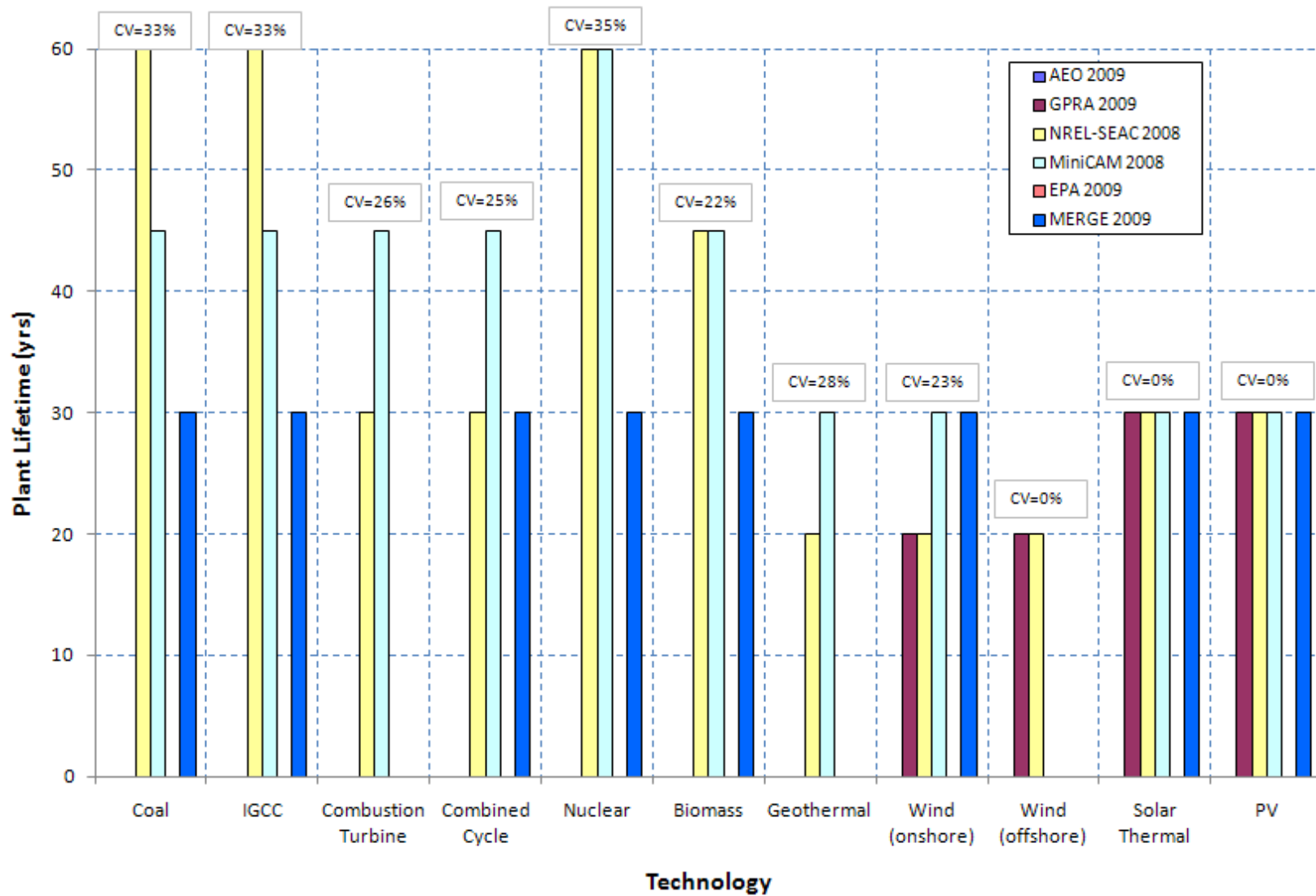
Figure 5. Plant lifetime comparison
