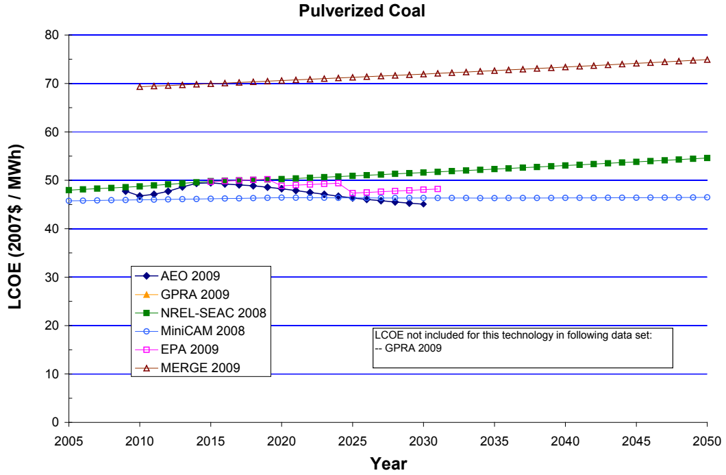
Figure 54. LCOE—coal
