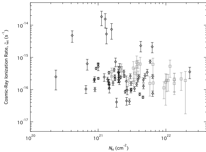
Figure 25. Cosmic-ray ionization rate vs. total hydrogen column density, N_{\text{H}} . We have estimated N_{\text{H}} using values of N(\text{H}) and f_{\text{H}_2} reported in Table 5. Black diamonds are from the present study, and gray squares from \text{H}_3^+ observations of Indriolo & McCall (2012). All ionization rates above 10^{-15} \text{ s}^{-1} are from sight lines toward the Galactic center.
