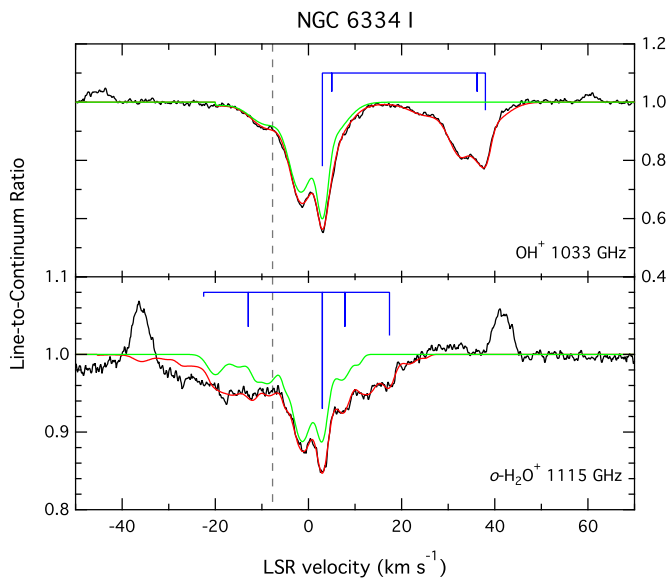
Figure 20. Same as Figure 2 but for NGC 6334 I.
