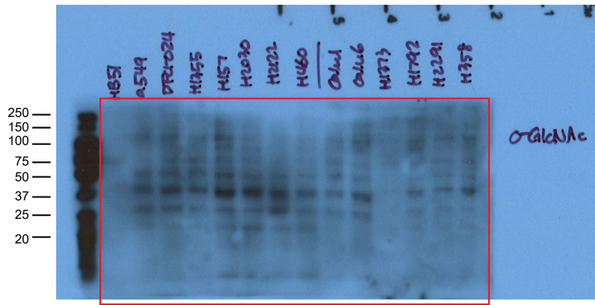
O-GlcNAcylation
