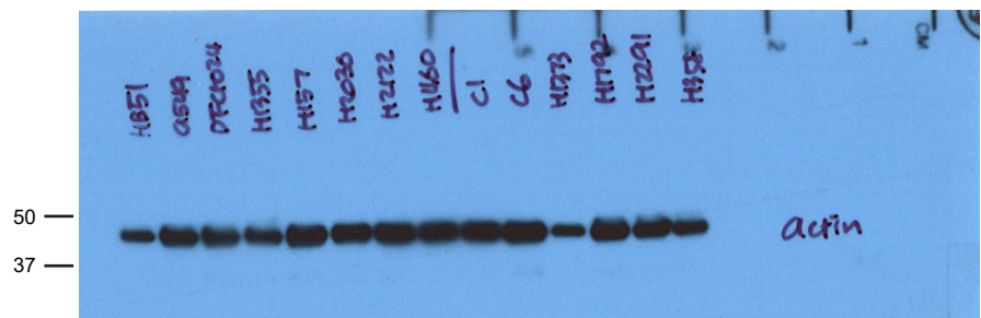
Actin
