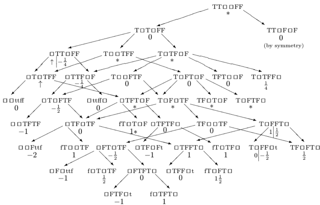
Figure 18. The 6-place Toads-and-Frogs Game (2, 2)_2 .
