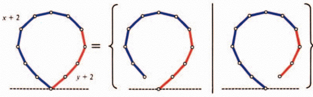
Figure 4. A Childish Hackenbush Loop Worth \{x \mid -y\} .
