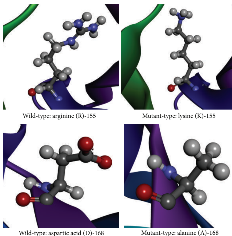
FIGURE 2: The figure depicts the native and mutated residues (shown in balls-and-stick model) of the variants R155K and D168A in the structure of NS3 protease (color rainbow). As can be inferred, the change in the residues introduced larger amino acid groups for R155K that will decrease the binding efficiency of drug molecules due to more steric hindrances. Also, the introduction of nonpolar groups for D168A transition will contribute to only weaker molecular interactions and thus reduced binding.
