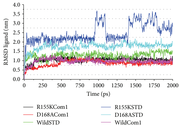
FIGURE 7: Ligand RMSD calculation plots for ligand bound complexes. The curves colored in blue and cyan show the instability of Asunaprevir inside the binding cavity of R155K and D168A mutants, respectively, while good stability is seen in wild type as shown by the green curve. Andrographolide is relatively very stable with very less deviation in the RMSD values for all the complexes (curves colored in black for R155K, red for D168A, and pink for wild-type structures, resp.). (Note: Asunaprevir is mentioned as STD and Andrographolide as Com 1.)
