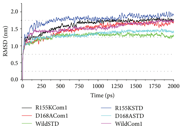
FIGURE 6: Protein backbone RMSD calculation plots for ligand bound complexes. Asunaprevir perturbs backbone of the protein mutant R155K (curve in blue) more than Andrographolide (curve in black). Surprisingly, Andrographolide seems to disturb protein structure for the mutant D168A more than Asunaprevir (check cyan curve for Asunaprevir and red for Andrographolide). (Note: Asunaprevir is mentioned as STD and Andrographolide as Com 1.)
