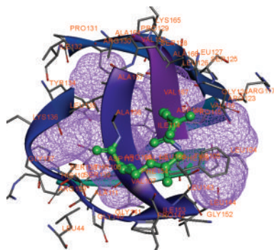
FIGURE 3: Active site of target protein with mutant structure shown in ball-and-stick model of variants R155K and D168A (violet wire mesh indicates binding cavity in the active site).
