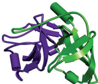
FIGURE 1: The figure depicts the structure of NS3 protease with schematic model. Violet color shows the N-terminal serine protease domain region in the protein, and green color shows the C-terminal domain region that is a member of the DExH/D-box helicase superfamily II with NTPase activity.
