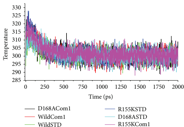
FIGURE 5: Temperature equilibration of the ligand-protein systems. As can be seen from the plots, the systems for all the ligand-protein complexes readily attained the temperature set at 300 K and maintained it throughout the simulation period. (Note: Asunaprevir is mentioned as STD and Andrographolide as Com 1.)
