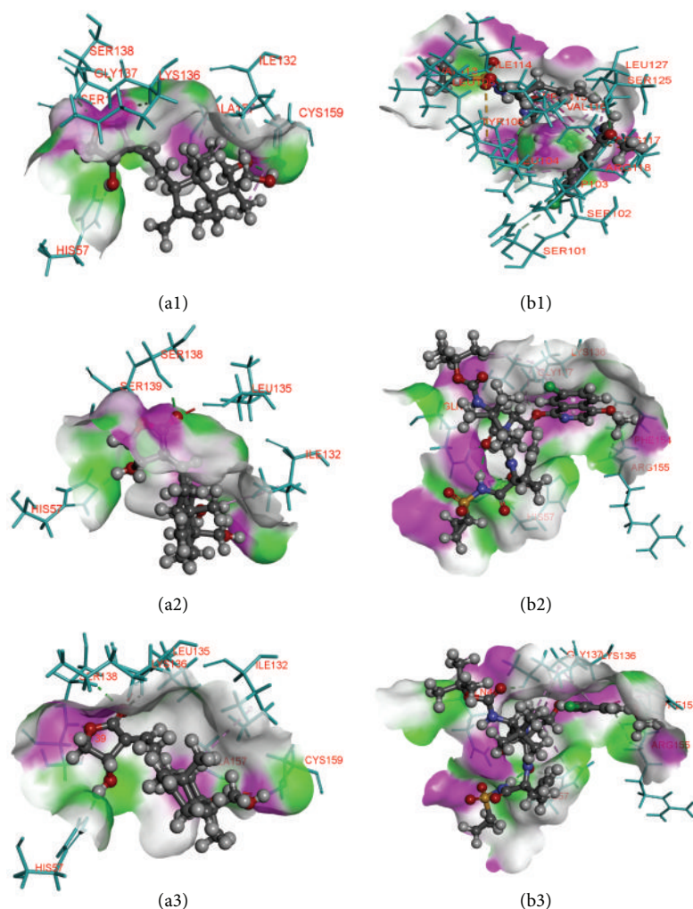
FIGURE 4: Binding poses and atomic interactions between ligands and receptors. (a1, a2, a3) series depicts Andrographolide interactions with the wild-type mutant R155K, and mutant D168A, respectively. (b1, b2, b3) series depicts the same with Asunaprevir and mutants in the same order above (see text for interacting residues). Note: ligands shown in ball-and-stick pattern and interacting residues shown in stick pattern, protein surface. Pink: donor, green: acceptor.
