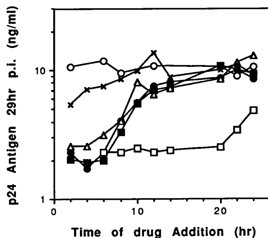
FIG. 2. Time-of-addition experiment. H9 cells were infected with HIV-1 III B at a multiplicity of infection of 0.1, and compounds were added at various times postinfection (p.i.) as described in Materials and Methods. The amounts of p24 accumulated at 29 h p.i. were determined with a Coulter enzyme assay kit. ○, no drug; ●, 1506 (7.4 \mu\text{M} ); ■, 1580 (7 \mu\text{M} ); △, AZT (1.9 \mu\text{M} ); □, Ro 31-8959 (HIV PR inhibitor; 0.65 \mu\text{M} ); ×, dextran sulfate (molecular weight, 8,000; 6.3 \mu\text{M} ).
