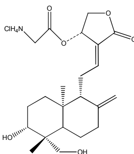
14-Glycyl andrographolide hydrochloride
