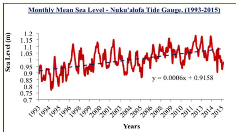
Figure 7: Monthly Mean Sea Level in Nuku'alofa, (1993-2015)
