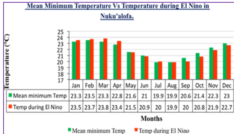
Figure 6: Mean Minimum Temperature Vs Temperature during El Nino in Nuku'alofa
