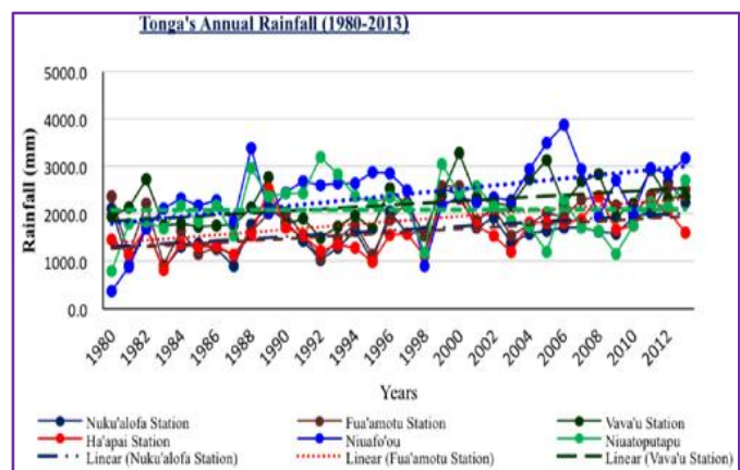
Figure 4: Tonga's Annual Rainfall, (1980-2013).
