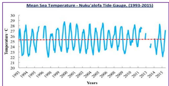
Figure 3: Yearly Sea Temperature in Nuku'alofa, (1993-2015).
