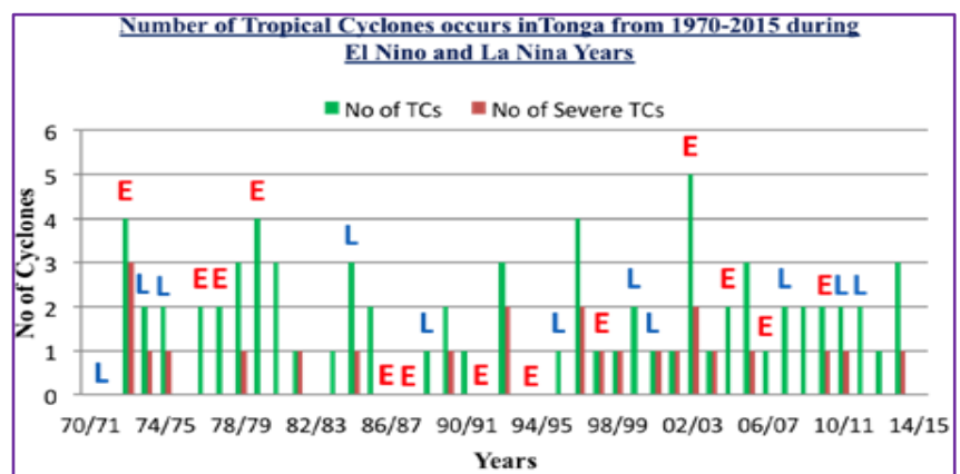
Figure 5: Number of Tropical Cyclones occurs in Tonga, (1970-2015)
