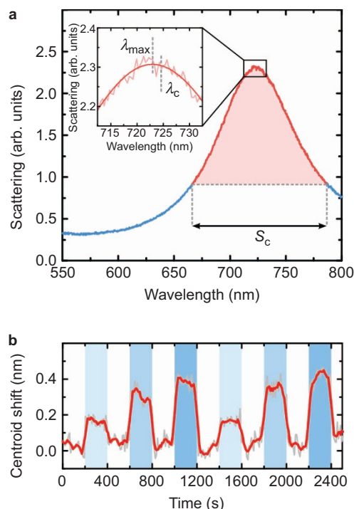
Figure 5 (a) Dark-field scattering spectrum of a single Au–DNA–Pd nanorod on a glass substrate. S_c indicates the wavelength span included in our centroid calculation. Comparison of the wavelength of the scattering maximum \lambda_{\max} and the centroid wavelength \lambda_c (inset). (b) Time-resolved sensing performance of the DNA-assembled nanosensor when exposed to cycles of 10, 20 and 30 vol.-% H_2 in N_2 and N_2 carrier gas. The gray line represents the centroid wavelength from scattering spectra taken every 10 s with an integration time of 8 s. The red line is a running average over five data points.
