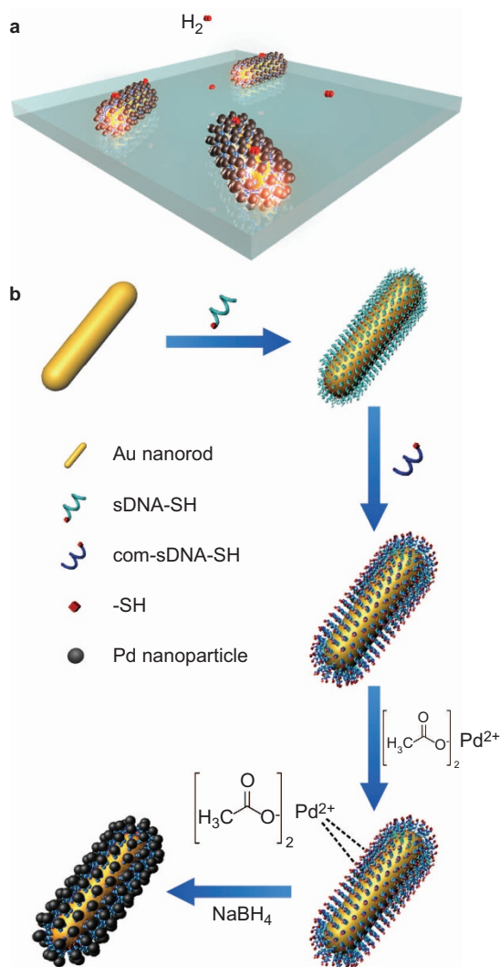
Figure 1 (a) Schematic of the DNA-assembled bimetallic nanosensor, which is composed of palladium (Pd) nanoparticles that are connected to a gold (Au) nanorod via DNA linkers. (b) Synthesis details for the self-assembled device.
