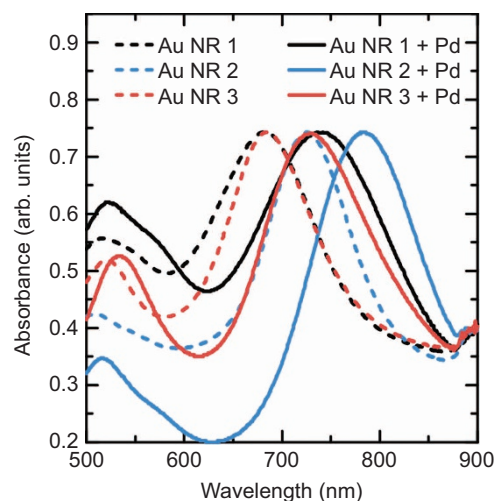
Figure 4 Ensemble absorbance spectra for three batches of Au nanorods of different design lengths, with and without DNA-assembled Pd nanocrystals (solid and dashed curves). NR, nanorod.
