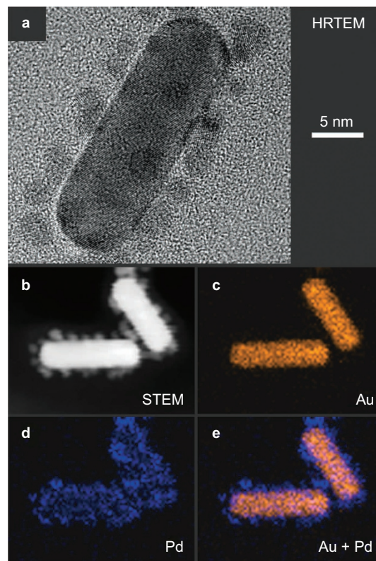
Figure 3 (a) HRTEM image of an Au–DNA–Pd nanorod from batch 1. The sub-5-nm satellite Pd nanocrystals are clearly visible. (b) STEM image of two nanorods from batch 1. (c–e) Element-resolved (energy-filtered) STEM images of the same nanorods. HRTEM, high-resolution transmission electron microscopy; STEM, scanning transmission electron microscopy.
