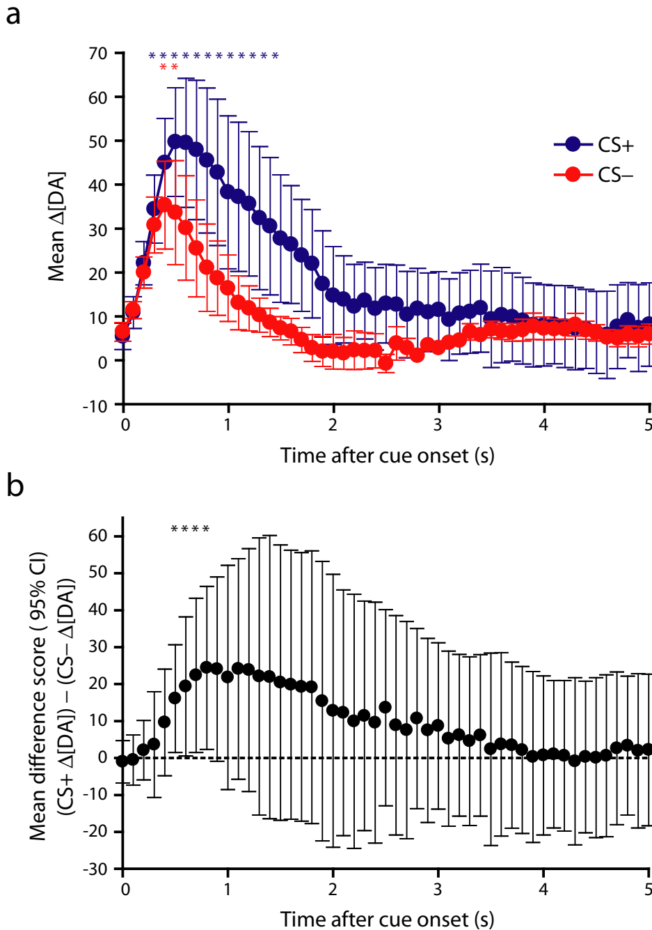
Supplementary Figure 3. Cue-evoked dopamine release after extended conditioning. (a) Mean differential dopamine concentration for 5 s after CS+ (blue trace) and CS- (red trace) onset. CS+ evoked NAc [DA] was significantly elevated from baseline levels at 0.3–1.4 s after cue onset (blue asterisks; p < 0.05 for each comparison). CS- evoked [DA] was significantly increased from baseline levels at 0.4–0.5 s after cue onset (red asterisks; p < 0.05 for each contrast). (b) CS+/CS- difference score ((CS+ [DA]) - (CS- [DA])) during the same time period. CS+ evoked [DA] was significantly higher than CS- evoked [DA] at 0.5–0.8 s after cue onset (*95% CI does not include zero).
