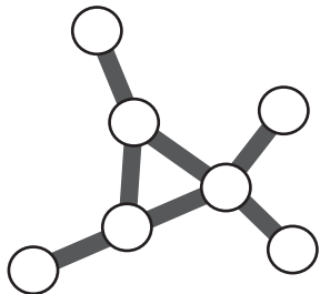
Biomolecular network
