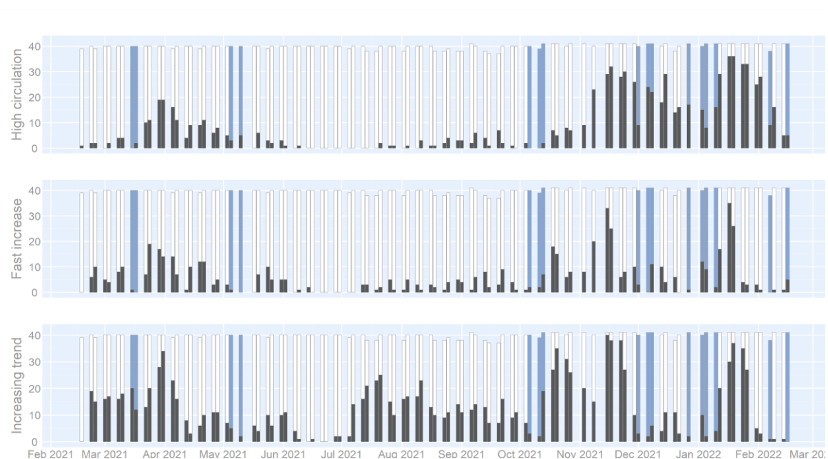
Figure 3: The number of areas (among the 41 covered by the wastewater surveillance this week and the 42 normally considered), with positive alerting indicators (black) compared to total number of areas considered every week in the wastewater surveillance (white). Latest results (last bar) from February 16 th 2022. The white bars represent the total number of areas considered every week in the wastewater surveillance. The blue bars indicate dates at which an underestimation of the number of areas in which indicators are fulfilled due to dilution in the wastewaters.
