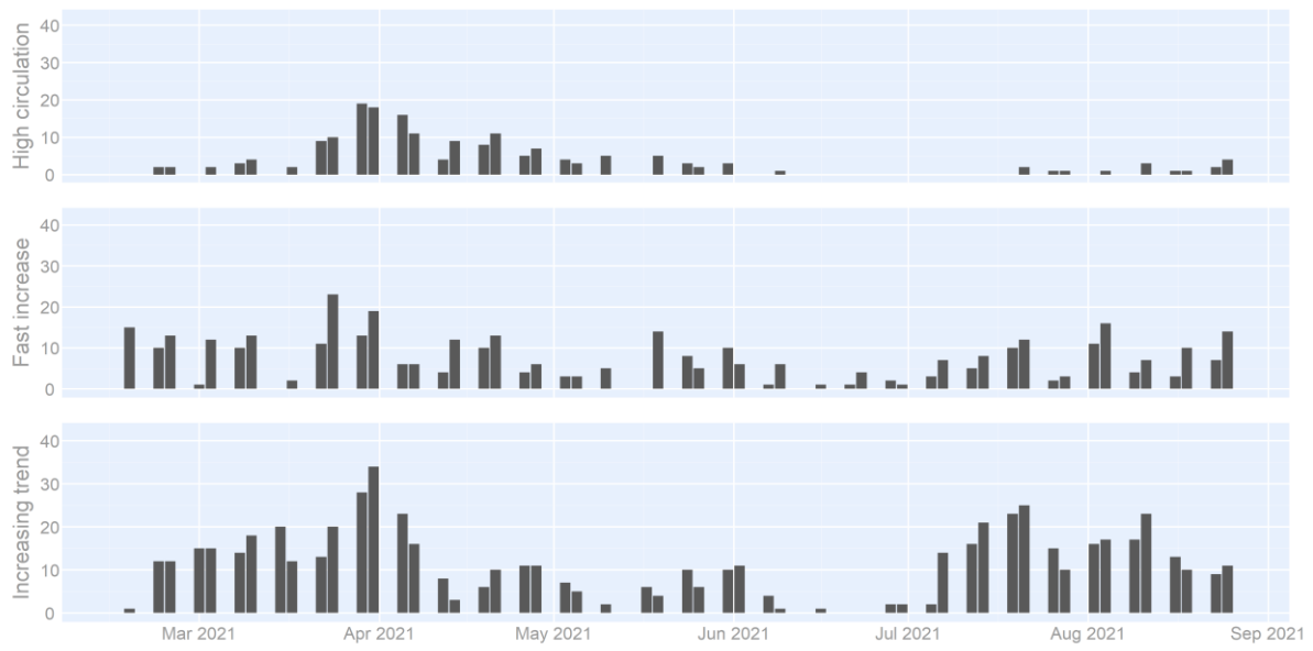
Figure 3: The number of areas, amongst the 38 areas covered by the wastewater surveillance, with positive alerting indicators (latest results on August 25th 2021).
